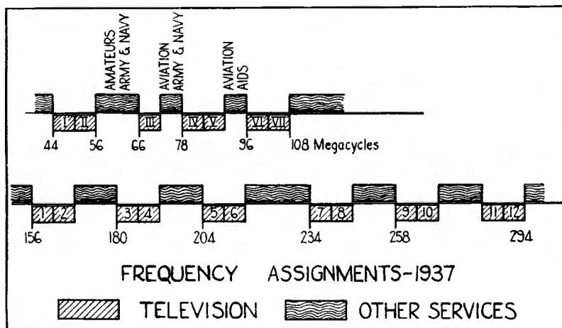
Fig. 4. The recent television frequency assignments.
