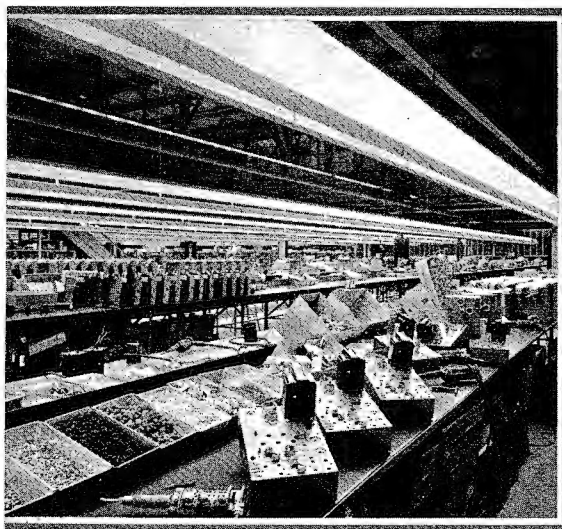
The lower part of the light-hood consists of an aluminum reflecting trough mounted on a wiring channel. All the wires for each line are carried in this channel. A pipe batten hung from the ceiling furnishes main support.
