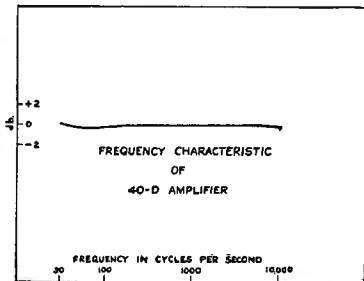
Uniform frequency response
