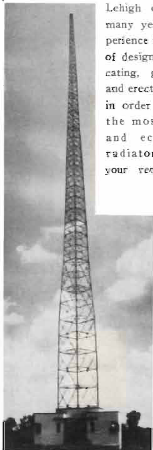
485 ft. Shunt- excited Lehigh Antenna at WJBO Baton Rouge, La.
