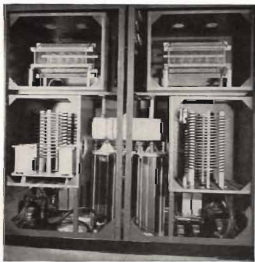
Rear view of the new 50 KW amplifier which employs the Doherty high efficiency circuit.
