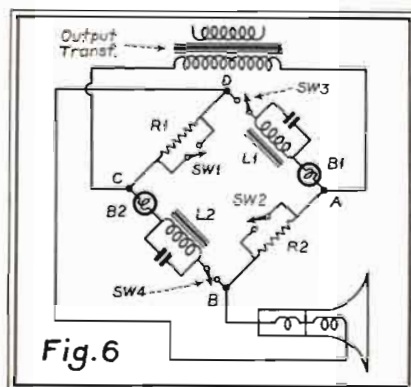
Fig. 6 Illustrating the variable-resistance method of expansion.
