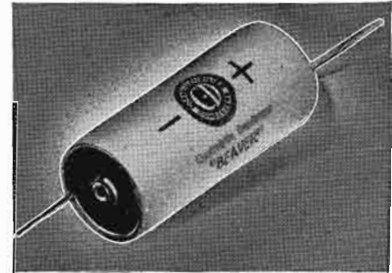
TYPE BR "Blue Beavers." The Type BR etched foil dry electrolytics are hermetically sealed, vented and encased in round aluminum containers with a protective outside sleeving. These capacitors eliminate drilling of chassis, use of pal nuts, washers and minimize assembly operations as well as save space and afford quick wiring.
