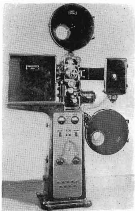
(1) A Farnsworth type disector tube film scanner as manufactured by the Fernseh A. G. It is possible to scan four pictures with this device.
