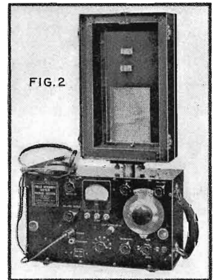
FIG. 2 The field intensity meter set up for use.
