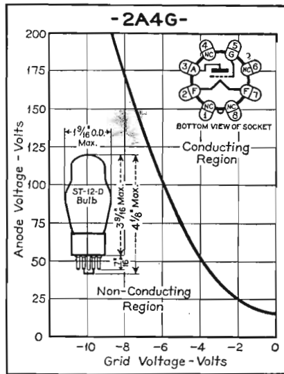
Fig. 3. The E_g-E_a characteristic of the Raytheon thyratron rectifier.
