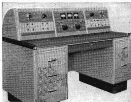
The 5-DX Operating Console—smart, streamlined—contains V1 and monitoring amplifier, controls for transmitter and speech input equipment.
