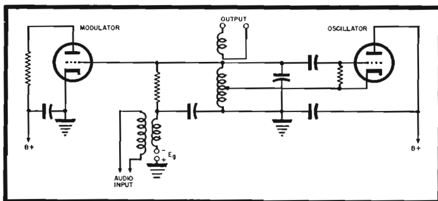
Figure 2 (left) An f-m generator circuit with the modulator shown in Figure 1.
