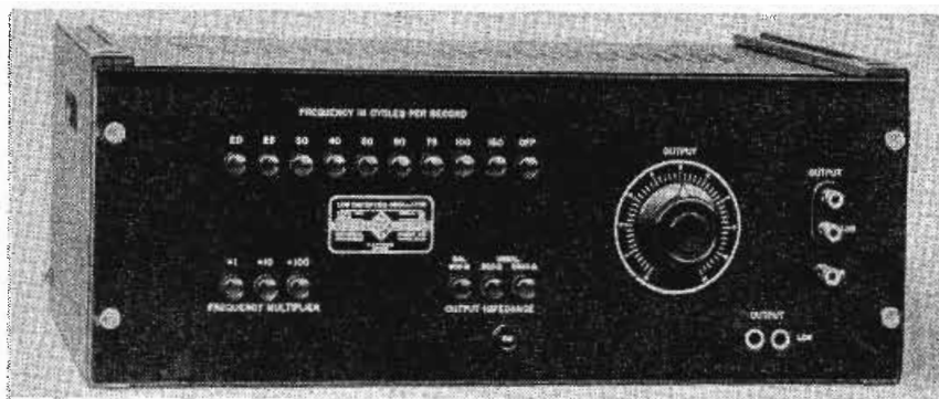
Typical low-distortion (.1%) RC oscillator. (G.R. 1301-A)
