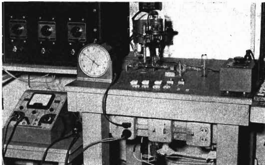
Figure 1 View showing upper section of quartz-crystal plating setup.
