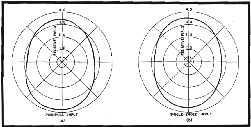
(Scheldorf Paper) Circular antenna patterns: (a) push-pull input; (b) single-ended input.
