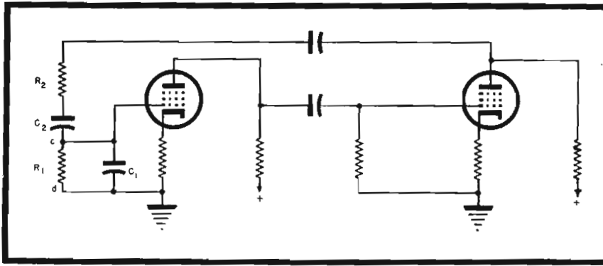
Figure 6 Simplified circuit of an RC oscillator where R_1 , C_1 , R_2 and C_2 are the frequency-determining constants.
