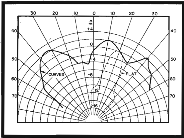
(Morrill Paper) Polar distribution characteristics of reflected wave for convex and flat panels.
