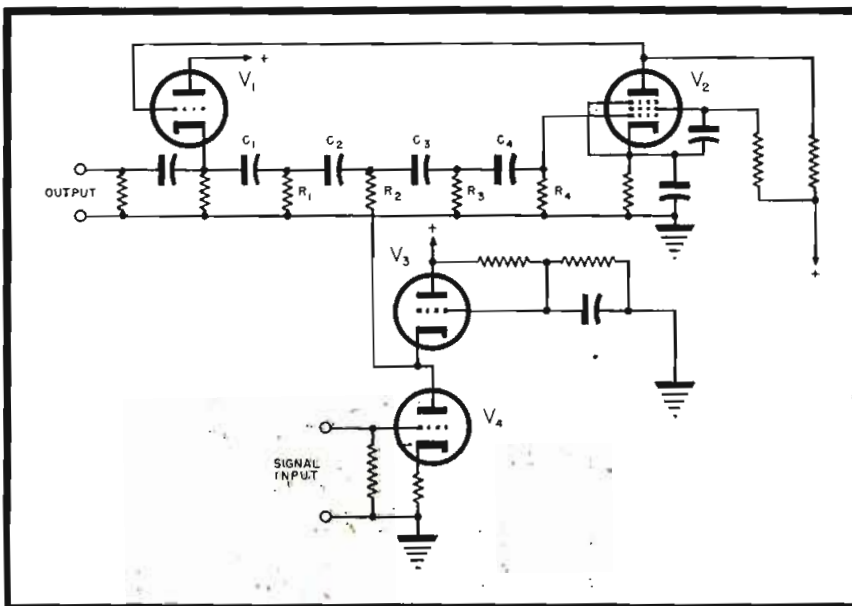
Figure 8 A ladder-network RC oscillator employing a four-step ladder and tubes, V_3 and V_4 , to vary the frequency.
