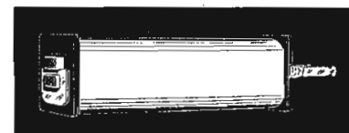
Coil core of a.c. relays is of thin laminations of silicon steel, riveted together. This reduces hysteresis and eddy current losses, gives large amount of power with small heat losses.
