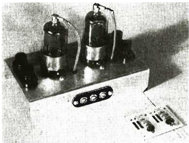
Comparison of an amplifier built by the customary method and the printed circuit method.
