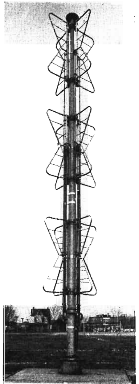
(Holtz Paper) Super turnstile antenna.
