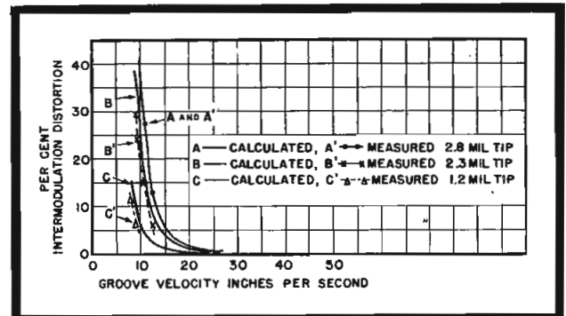
(Roys Paper) Comparison of measured and calculated results of intermodulation distortion tests with pickups of different tip radii.
