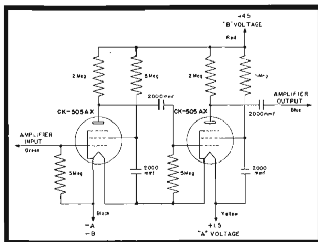
Typical circuit used for printed amplifier.
