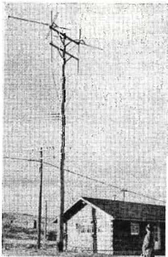
Installation above is on Mount Coolidge, 6400' above sea level. The 250-w transmitter antenna is atop. Rapid City h-f link antennas below; at left 81-mc antenna and at right 79-mc antenna. Below appears installation at Rapid City sub-headquarters.
