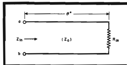
Figure 3 A length of transmission line \theta^\circ long with a characteristic impedance Z_0 that is terminated in a resistance R_m . The input impedance of the lines is Z_{in} .
