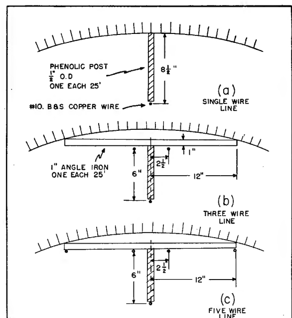
Figure 2 Physical arrangement of the transmission lines. Arrangement in C was used in final setup.
