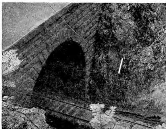
East portal of the Mt. Airy tunnel showing the radio transmission lines. The double-wire feedline at the upper part of the illustration is connected to the rhombic antenna placed atop of the tunnel.
