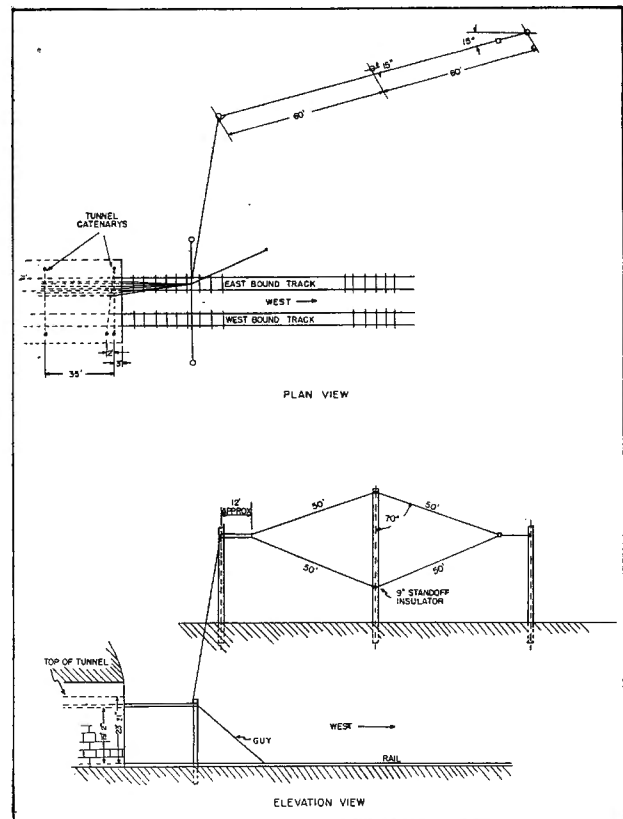
Figure 5 Layout of rhombic-antenna system located on top of the tunnel at either tunnel mouth. Rhombics had a theoretical gain of 15 db.
