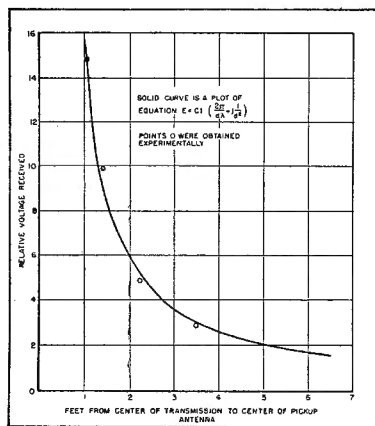
Figure 3 (Below) Plot of voltage received at varying distances from the five-wire line of C in Figure 2.
