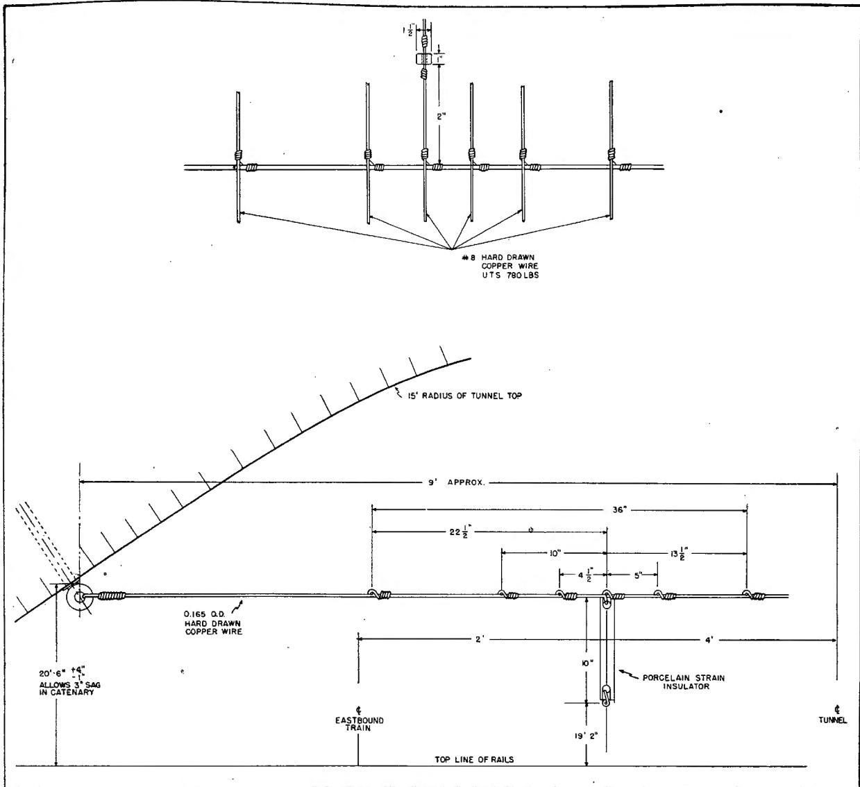
Figure 4 Installation setup in B. & O. tunnel at Mt. Airy, Md.; a double-track-lined tunnel 2,760' long.
