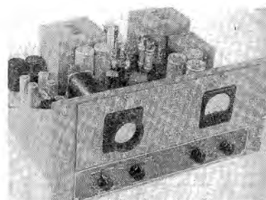
H-f frequency-shift receiver converter.
