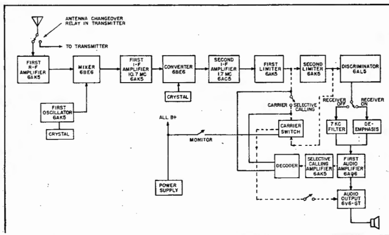
Figure 2 Block diagram of the mobile receiver.
