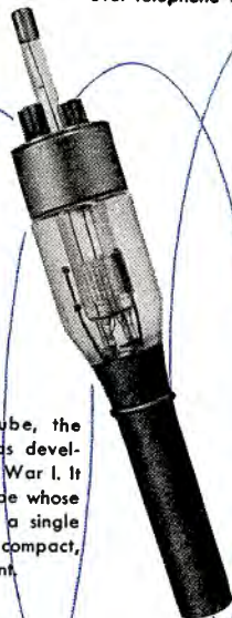
1919. The introduction of the copper-to-glass seal made water cooled tubes practical. The resulting high power tubes were used for broadcasting and for transoceanic radio-telephony.
