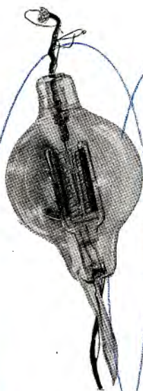
1912. The first effective high-vacuum tube, developed by the Laboratories for long distance telephony, was capable of operation at both audio and radio frequencies, and thus marked the beginning of modern electronics.
