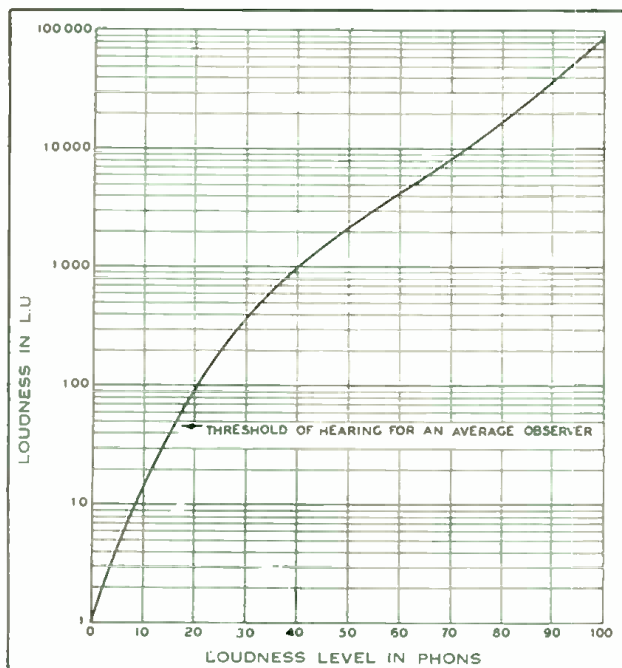
Figure 3 Relation between loudness and loudness level. (Courtesy ASA)
