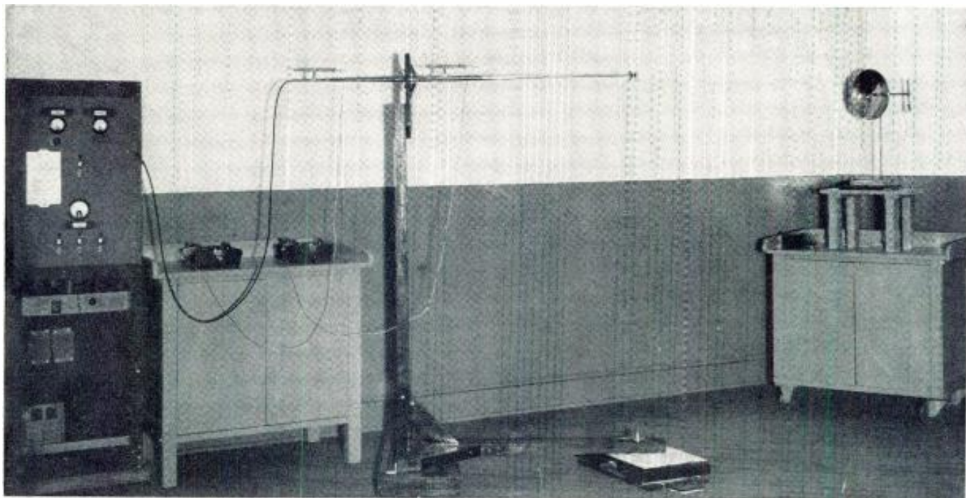
Figure 1 Complete setup of equipment used for measuring vertical radiation pattern of microwave antennas.
