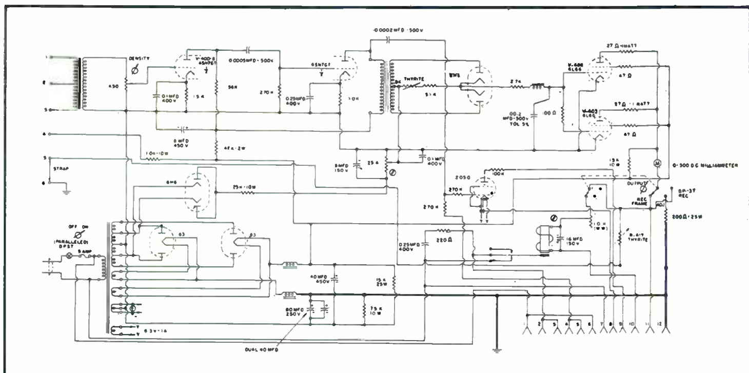
Figure 3 The recorder amplifier.
