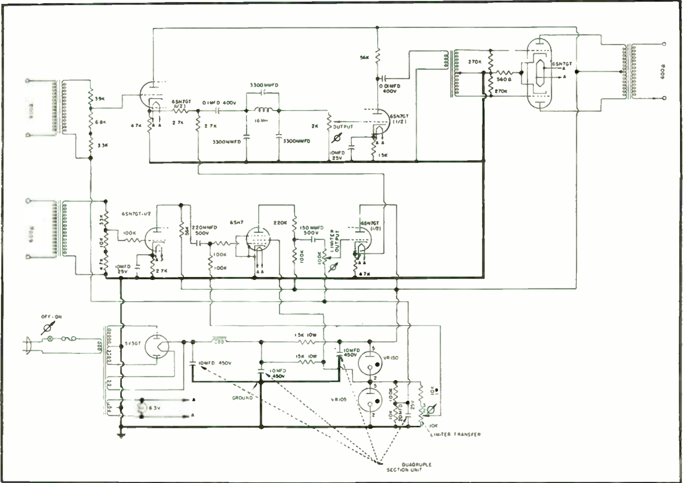
Figure 4 Limiter-line amplifier schematic.
