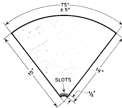
DIMENSIONS OF SHEET STOCK FOR PHASING CONES FIG. 5
