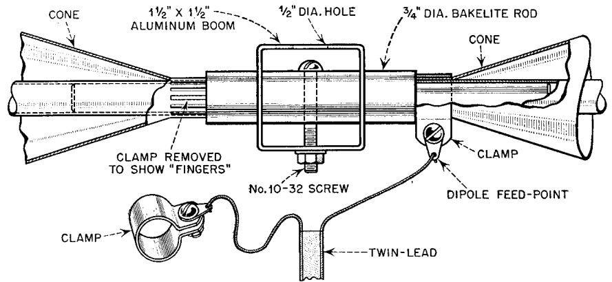
SHOWING DETAILS OF CENTER INSULATOR AND MOUNTING FIG. 6
