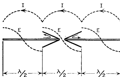
OPERATION OF DIPOLE ON HIGH CHANNELS
