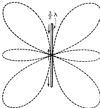
SHOWING "SPLIT" RADIATION PATTERN OF ANTENNA \frac{3}{2} WAVELENGTHS LONG FIG. 2
