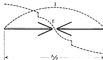
OPERATION OF DIPOLE ON LOW BAND
