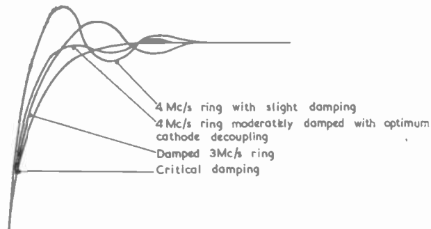
Fig. 4. Wave-front distortions produced by simple video stage
