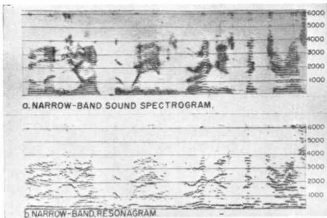
Fig. 2. Comparison of narrow-band spectrogram and resonogram of connected speech
