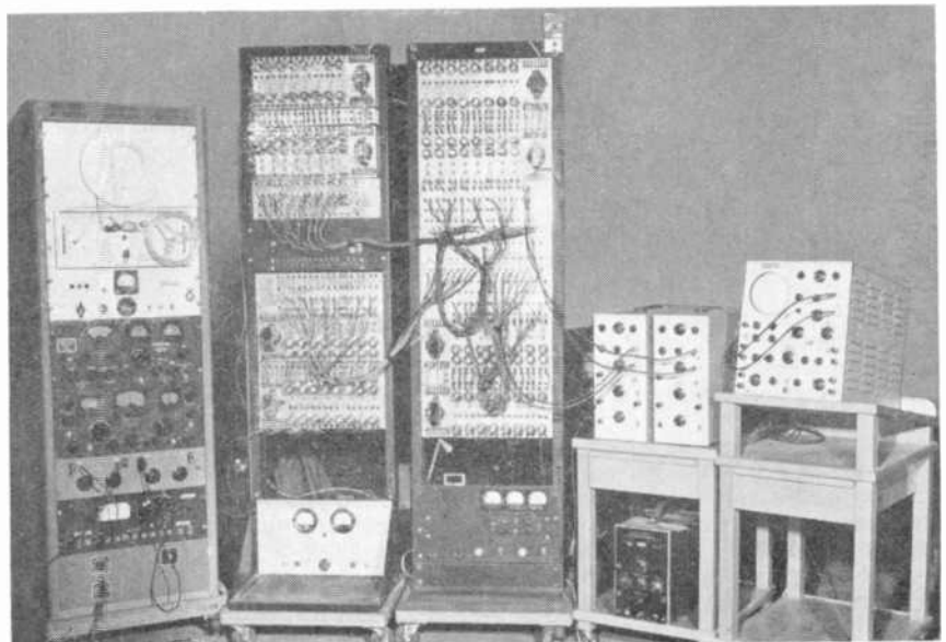
Fig. 9. The speech analyser and auxiliary equipment
