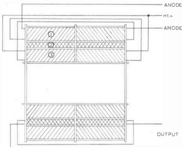
Fig. 5. Winding details of output transformer (15 \Omega termination). Winding 1—1310 turns 34 s.w.g. } enamel and Winding 2—114 turns 20 s.w.g. } single cupronium Winding 3—1310 turns 34 s.w.g. } insulation (The winding in each slot is the same but wound in the opposite direction).
