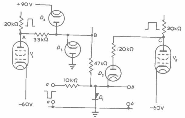
Fig. 10. Circuit diagram of combined subtracting and muting switch
