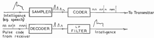
Fig. 1. Block diagram representing the essential parts of a pulse code modulation system
