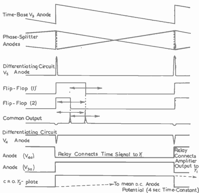
Fig. 3. Waveforms
