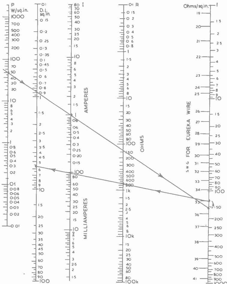
Chart for the design of wire wound resistors
