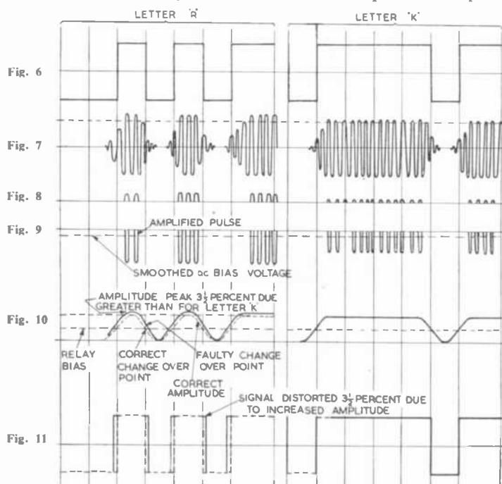
Figs. 6-11. Telegraph converter waveforms
