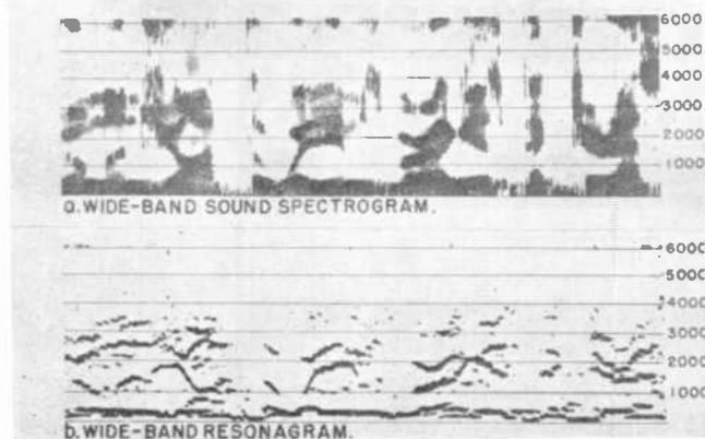
Fig. 3. Comparison of wide-band spectrogram and resonogram of some speech sample as Fig. 2
