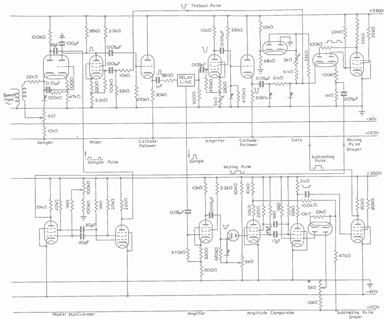
Fig. 12. Circuit diagram of sampler and coder.
