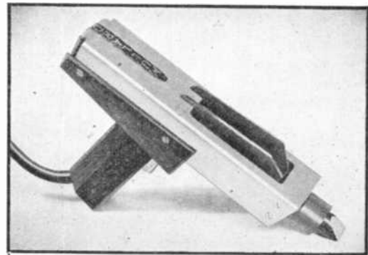
The soldering iron has a nickel silver bit driven by a magnetostriiction transducer. The transducer is arranged to run at its natural resonant frequency by a feed-back system. A conventional low voltage winding heats the soldering bit.
