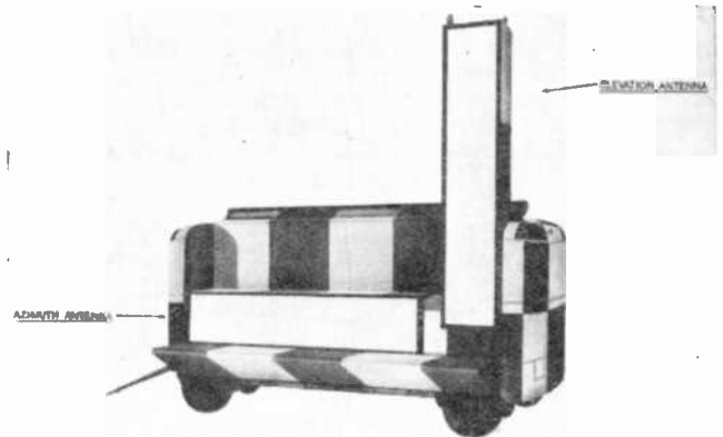
Fig. 9. Precision approach radar vehicle
