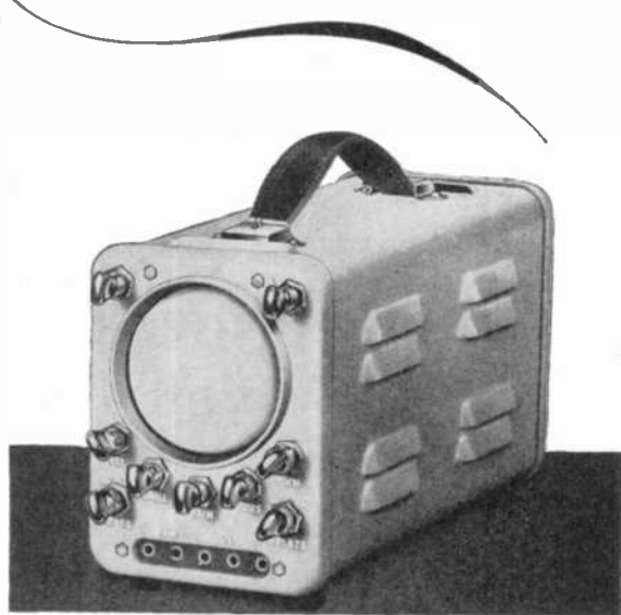
COSSOR Model 1039 PORTABLE OSCILLOGRAPH
