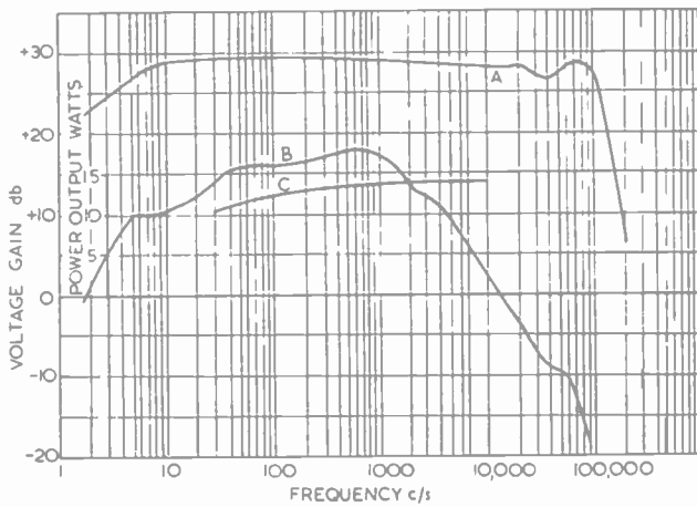
Fig. 3. Amplifier response curves A—complete amplifier with feedback, B— \mu\beta characteristics, C—power output for 5 per cent total harmonic production.
