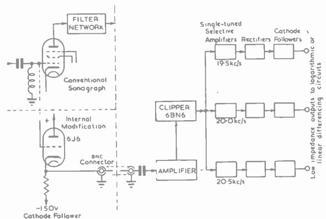
Fig. 5. Resonograph modification of sound spectrograph
