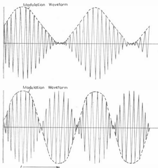
Fig. 1. The two modes of operation of bridge pick-ups
