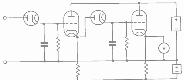
Fig. 2. Practical arrangement of two rectifier circuits in cascade
