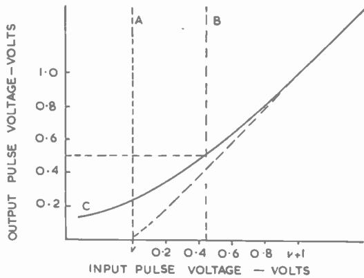
Fig. 8. Dynamic characteristic of diode switch near the cut-off point when set for subtracting
