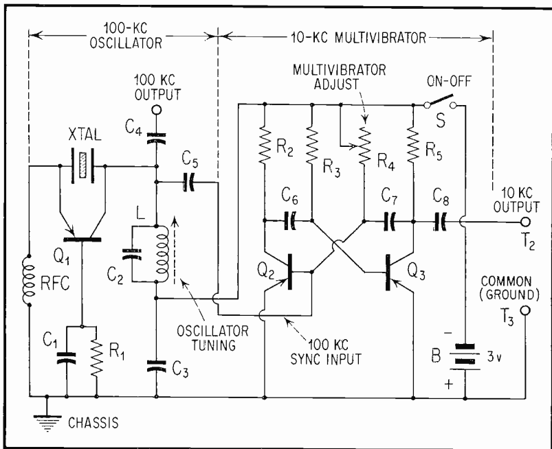
Fig. 3. Complete Circuit of the Frequency Standard.
