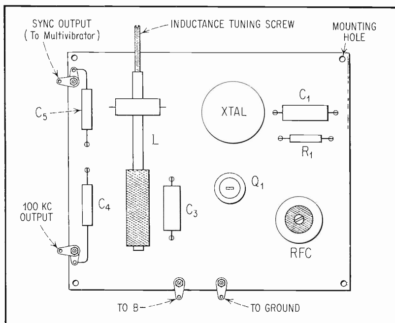
Fig. 5. Layout of Oscillator Circuit Board.
