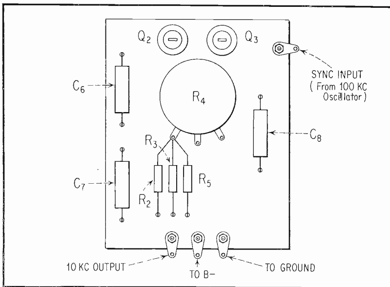
Fig. 7. Layout of Multivibrator Circuit Board.
