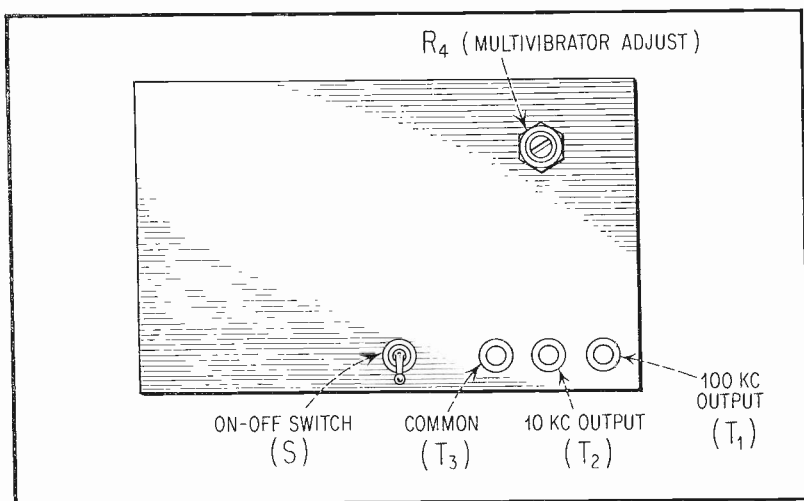
Fig. 8. Front Panel Layout.
