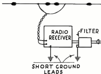
Fig. 4. Conventional doublet antenna connected to receiver with line filter. Use separate ground leads to eliminate common impedance in filter and receiver circuits.
