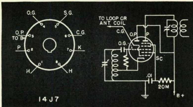
Fig. 4—A 12SA7 may be replaced by 14J7. Above circuit for Hartley type oscillators. The 12A8 can also be replaced by this tube.
