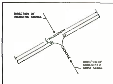
Fig. 5. Signal response of a half-wave dipole.
