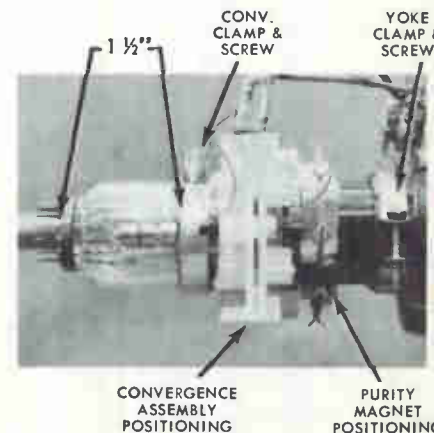
Fig. 4. Convergence Assembly Positioning
