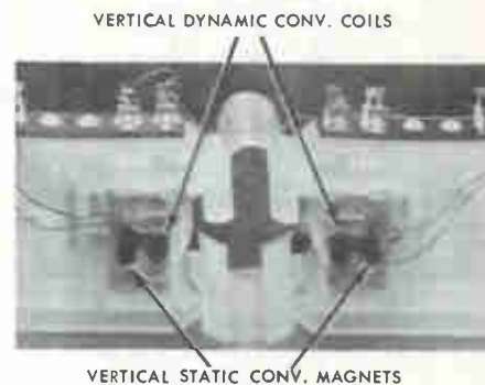
Fig. 2. Convergence Assembly Rear View
