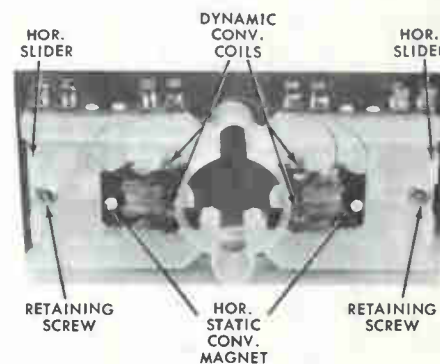
Fig. 3. Convergence Assembly Front View
