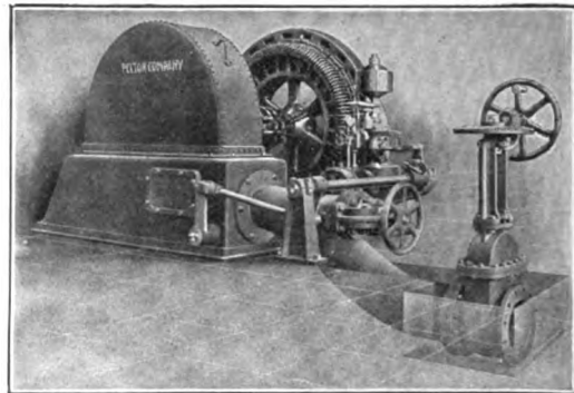
200-h.p. single overhung Pelton Impulse Wheel at a Mine in the Philippine Islands
