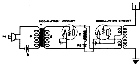
Fig. 14. Diagram of Transmitter Modulation and Oscillation Circuits
