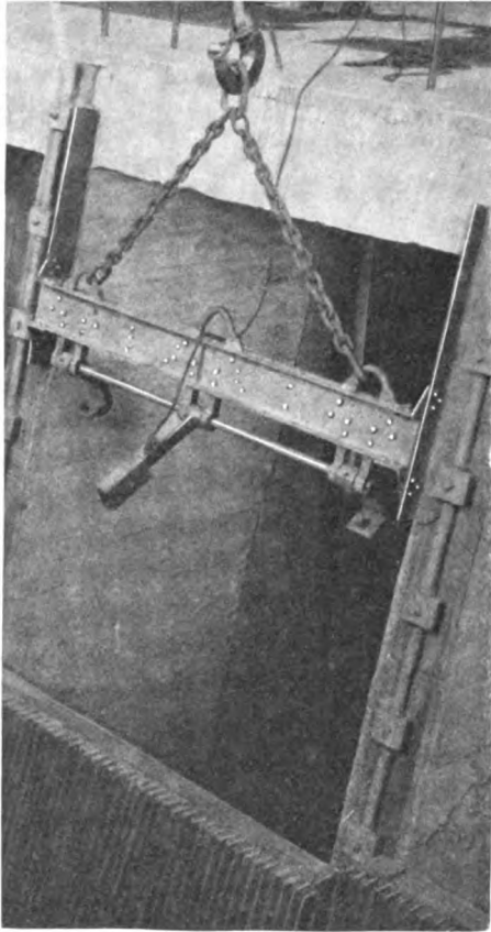
Fig. 5. This Screen Lifting Device eliminated the hazardous practice of grappling for the screen, pulling it to the water surface, and sending a man down to sling it to the crane hook
