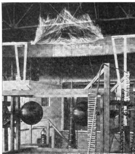
Fig. 36. 1,000,000 Volts Arcing Across a 9-ft. Spark Gap
