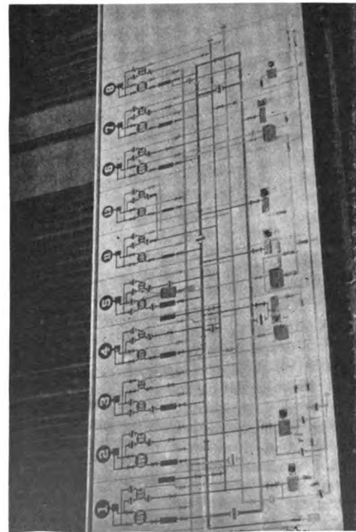
Fig. 1. A Hydraulic Mimic Board to which Hold-off Cards are Attached. It covers the piping and valves of governor and hand-control systems and other related piping. The operation of the pumps is indicated by red pilot lights
