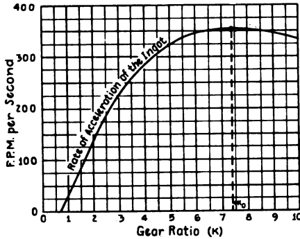
Fig. 22. Effect of the Gear Ratio on the Rate of Contactor Acceleration
