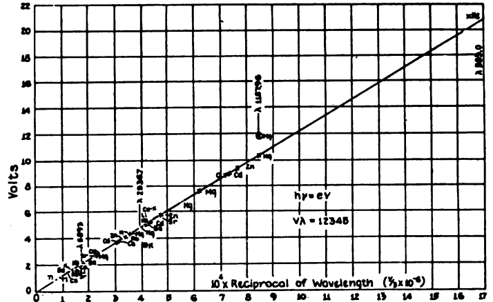
Fig. 4. The quantum relationship or the relation between frequency and voltage; critical values of voltage of a few elements are shown
