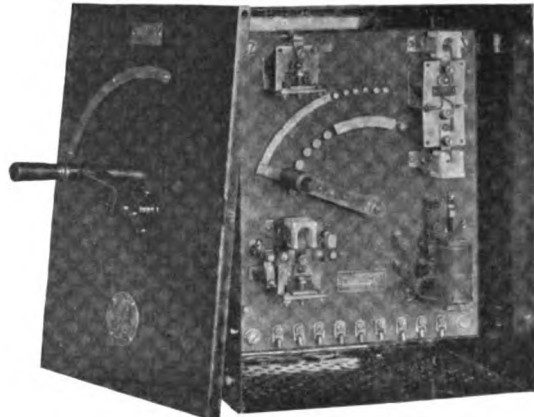
Fig. 49. Safety Type Predetermined Speed Controller
