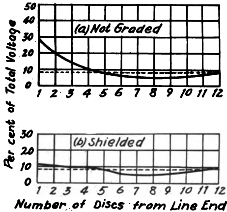
Fig. 7. Distribution of Voltage Over String of 12 Insulator Disks (a) Not graded; (b) Shielded by antenna or shielding ring. Dotted line shows even distribution of voltage.
