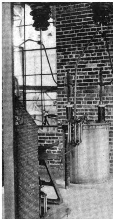
Fig. 3. Precipitator Transformer and Synchronous-motor-driven Mechanical Rectifier
