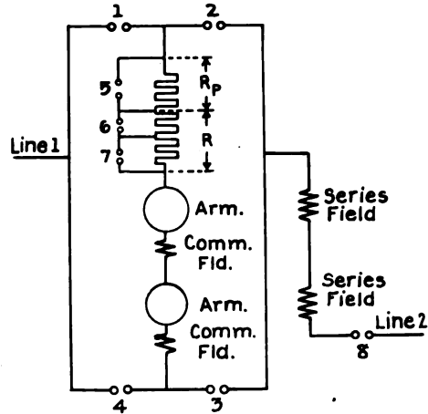
Fig. 14. Elementary Wiring Diagram of the Control Equipment
