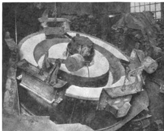
Fig. 24. 4000-lb. Induction Furnace Showing Rammed Lining in Place
