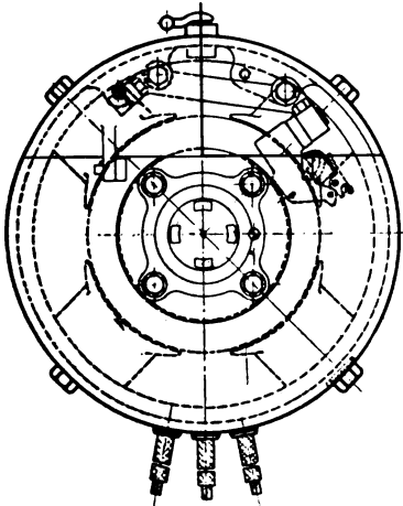
Fig. 2. A Cross Sectional View of a Standard Automotive Motor of the Two-brush Stud Type
