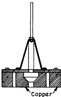
Fig. 3. Positive Arc Electrode
