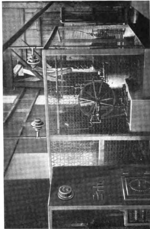
Fig. 8. Electrical Precipitator Equipment at a Commercial Size Copper Plant
