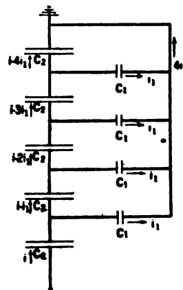
Fig. 7. Cause of Uneven Distribution. 7 The Capacities to Ground C_2 Cause an Uneven Distribution of Current Through the Insulator Capacity C_1
