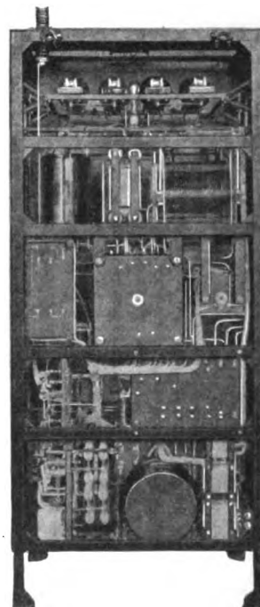
Fig. 6. Rear View of Transmitter shown in Fig. 4
