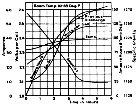
Fig. 2. Charging a 4-cell Ironclad Exide Battery in 5¼ Hours by the Modified Constant Potential System. Bus voltage 10.12 volts (2.53 volts per cell). Resistance in series 0.0214 ohms (0.00535 ohms per cell)
