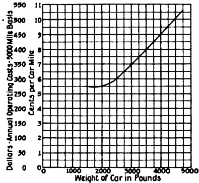
Fig. 2. Operating Costs of Automobile Passenger Cars
