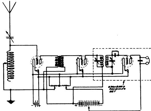
Fig. 18. Diagram of Connections for Radio Amplification
