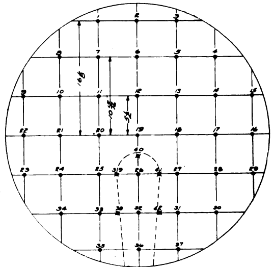
Fig. 4. "Checkerboard" Location of Thermocouple Stations on Back of Searchlight Mirror under Test
