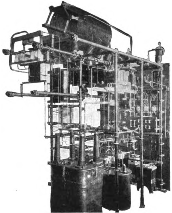
Fig. 13. Near view of Transmitter shown in Fig. 12
