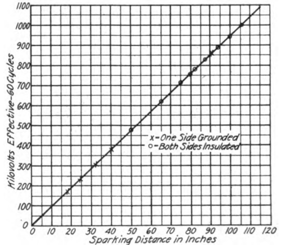
Fig. 16. Needle Gap Spark-over
