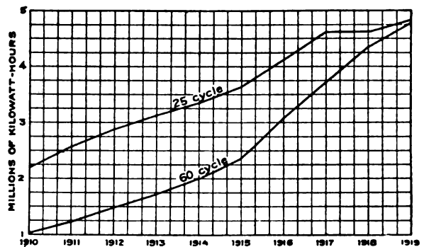
Fig. 8. Average Performance of Existing Steam-electric Plants to be Retained in the Superpower System
