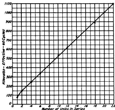
Fig. 22. Spark-over of Suspension Insulators
