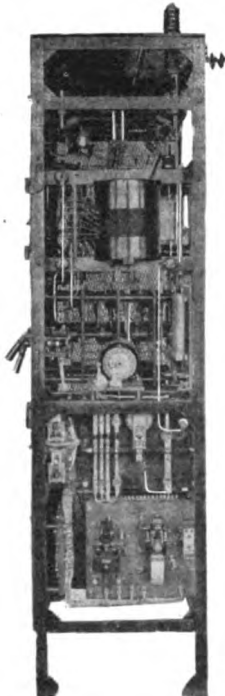
Fig. 7. Side View of Transmitter (Fig. 4) showing Starting Equipment and Sending and Receiving Relay
