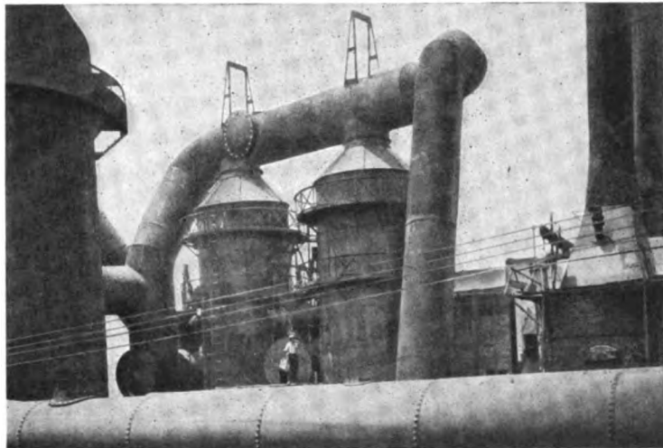
Fig. 7. Two Precipitator Units Handling Blast Furnace Gases
