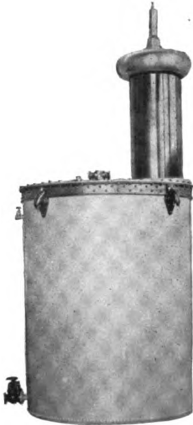
Fig. 3. Exterior View of the Main Transformer, 578,000 Volts. A similar unit stripped of cover, tank, and terminal is used as the line transformer
