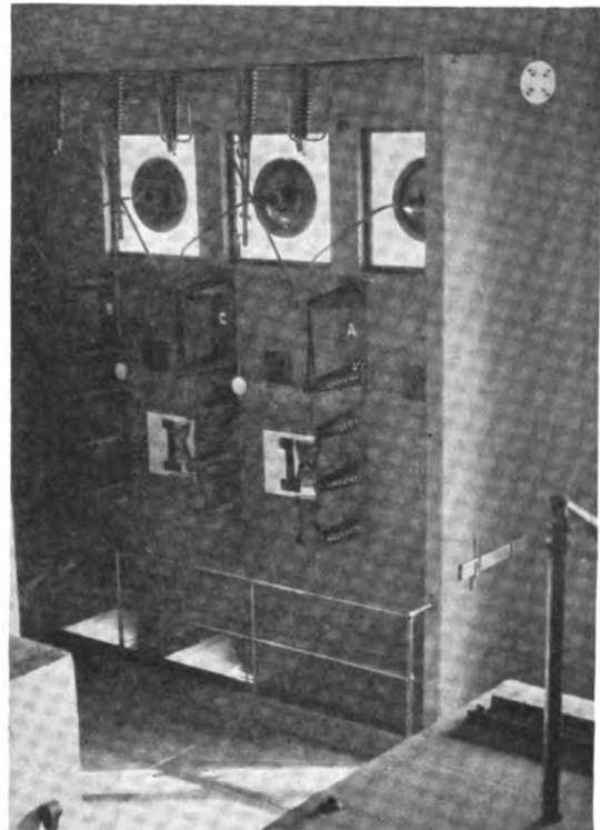
Fig. 3. Sleet Prevention Facilities at Receiving Station. The upper disconnectors serve to short circuit the transmission line when heating current is to be circulated. The disc in the upper right-hand corner carries eight 8-volt lamps in parallel connected to a series transformer in the short circuiting connections and indicates when the heating current is on.
