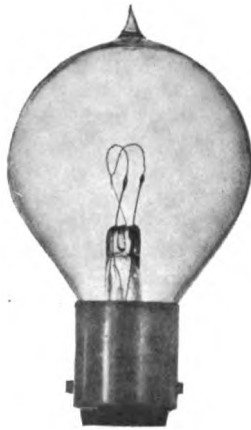
Fig. 1. 8 and 10-volt, 0.25-amp., C-3 Filament, S-11 Bulb, Mazda Lamp for Railroad Signal Service
