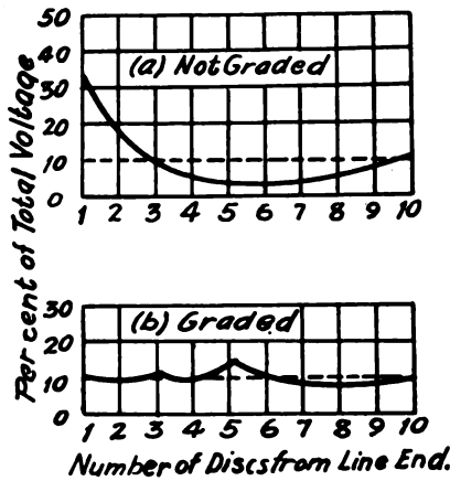
Fig. 6. Distribution of Voltage Over String of 10 Insulator Disks (a) Not graded; (b) Graded by means of metal caps placed on insulator disks. Dotted line shows even distribution of voltage.
