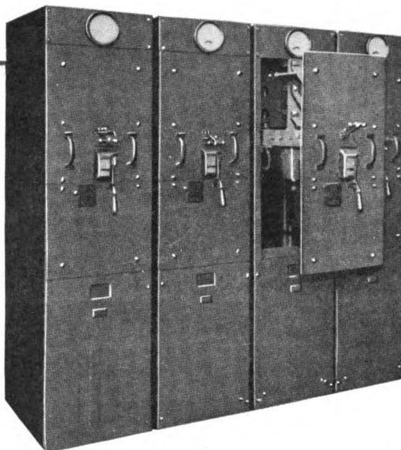
Safety Enclosed Standard Unit Switchboard made up of Type FK-20 Oil Circuit Breakers as Draw-outs
