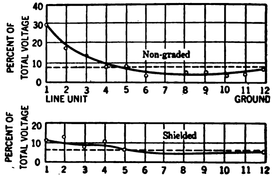
Fig. 10. Voltage Distribution on a String of Twelve Insulators
