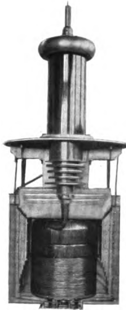
Fig. 4. Main Transformer Removed from its Tank; Front View, Showing the Tapered Major Insulation and the Extra-heavy Coil Insulation at the Top or Line End
