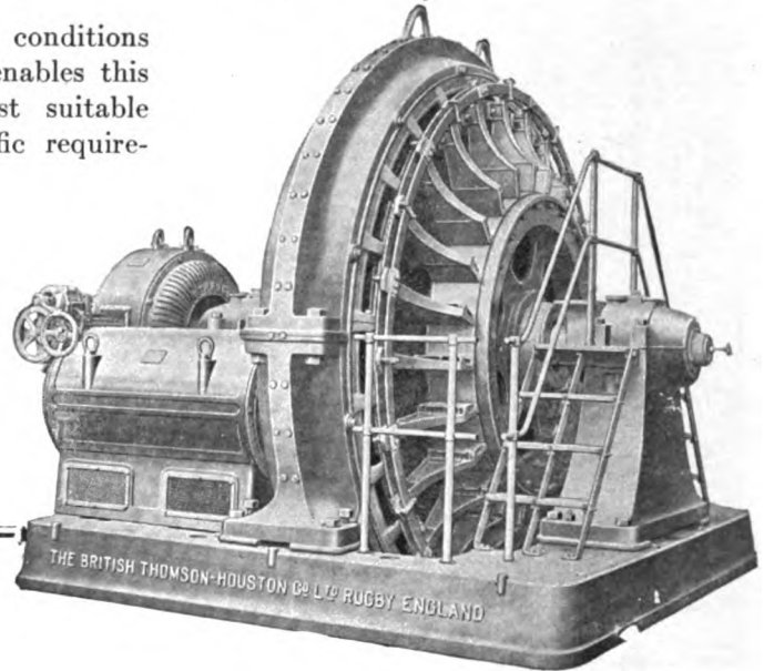
3,000-kw. Rotary Converter, one of seven similar machines supplied for electrolytic work.
