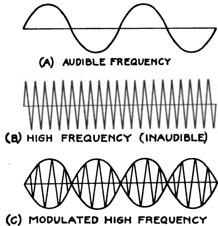
Fig. 13. Diagrams of the Voice Wave to be Transmitted, the Carrier Wave, and the Modulated Carrier Wave
