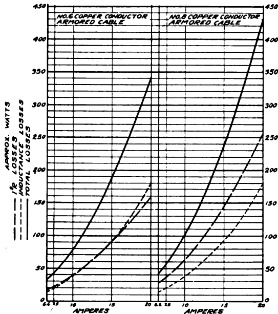
Fig. 16. The Relative I^2R and Inductance Losses in the Line for No. 6 and No. 8 Copper Conductor, Based on 1000 ft. Single-conductor Cable, \frac{1}{4} -in. Overall, Insulation of Lead and Steel Grounded Armor
