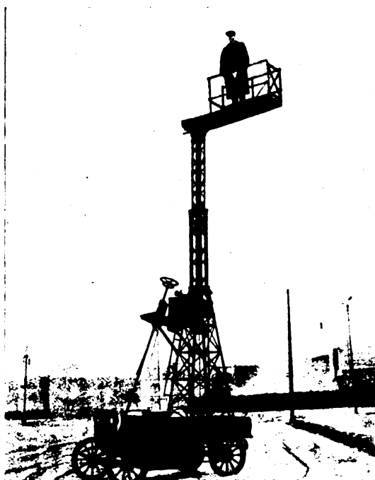
Fig. 5. An Electric Lamp Trimmer's Wagon with Center of Gravity so Low as to be Perfectly Stable When the Bridge is Raised and Offset. (Commercial Truck Company)
