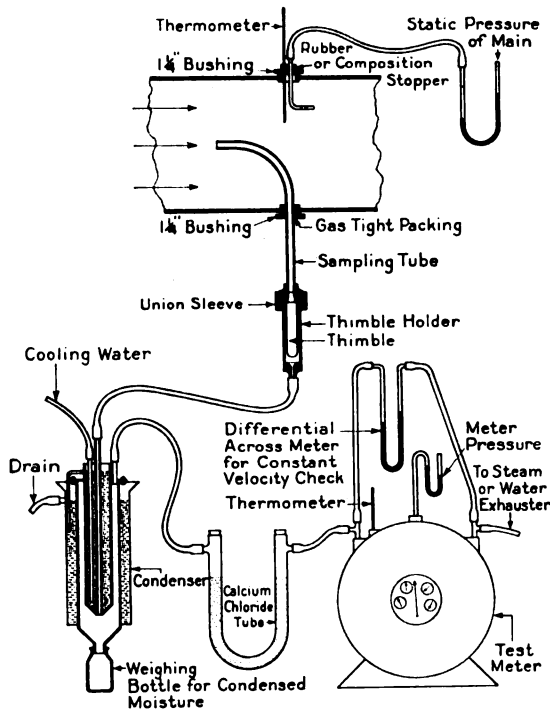
Fig. 2. Method of Sampling Gas
