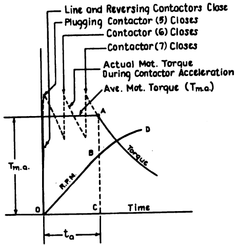
Fig. 15. Curves of Contactor Acceleration Period
