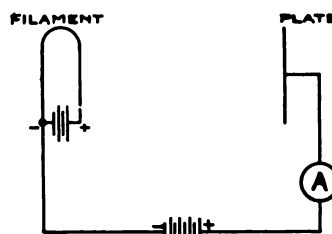
Fig. 5. Diagram of the Kenotron Circuit
