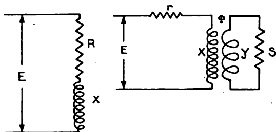
Fig. 2a and 2b. Electrical equivalents of furnace circuits
