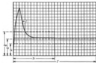
Fig. 8. Variable-current Duty Cycle
