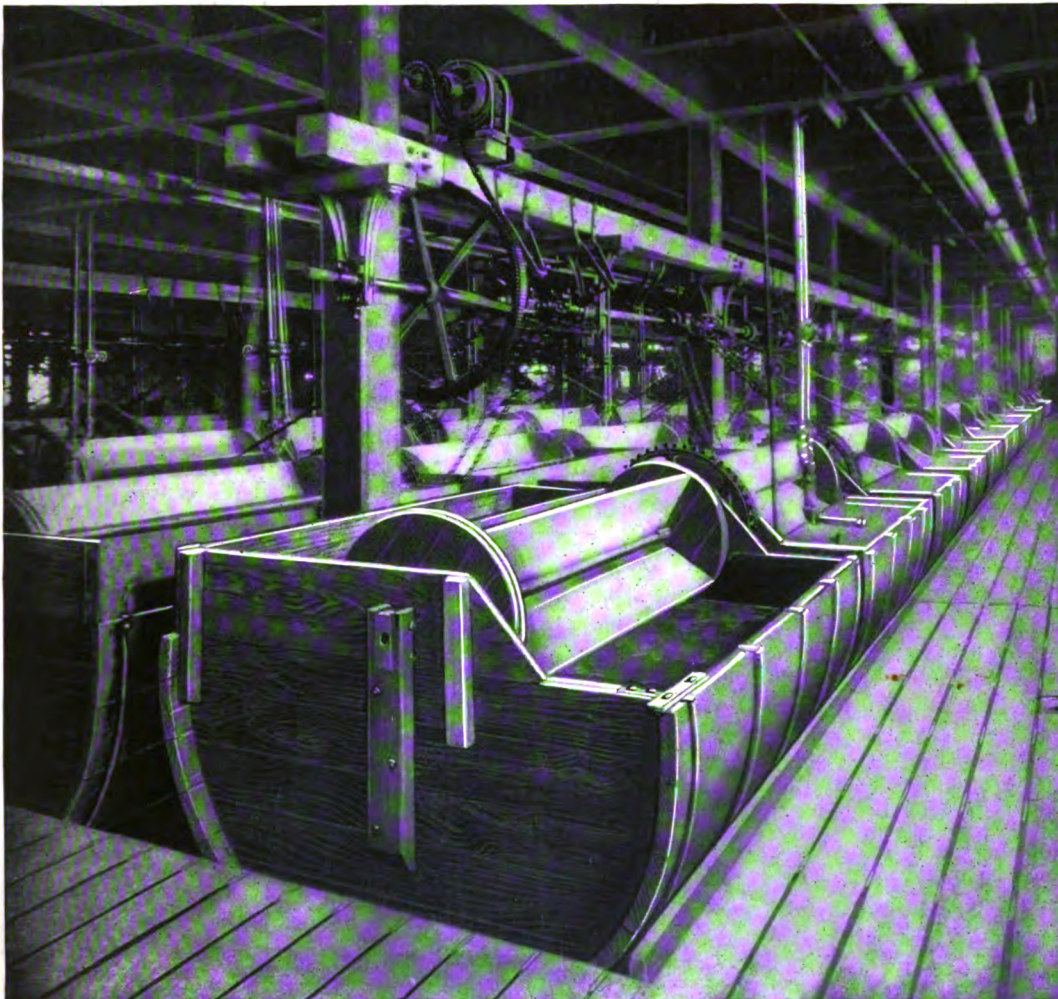
View of the lime yard of a recently electrified chrome tannery (John R. Evans Co., Camden, N. J.) It contains 164 lime reels, group driven by twelve 7½-h.p. induction motors, and has a capacity of 12,000 skins a day. Statistics now available after nine months of operation clearly indicate a saving of two-thirds the cost of the manual operation formerly used.
