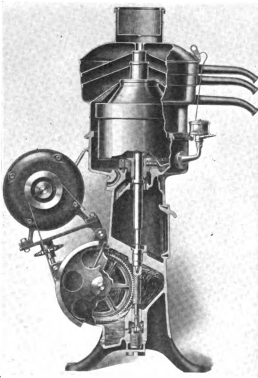
Fig. 5. Cross-sectional View of a Disc-type Motor-driven Centrifugal Oil Purifier
