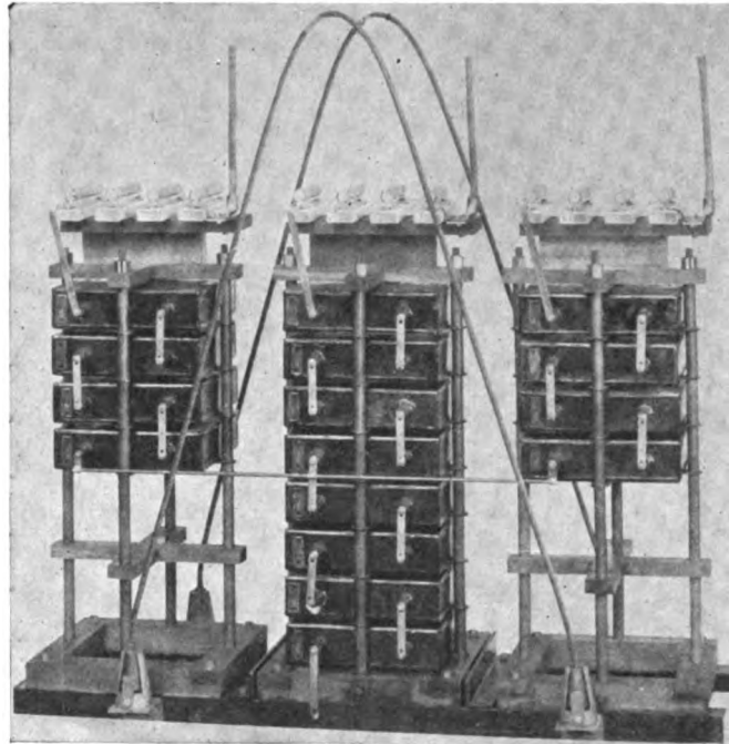
Fig. 20. Interior View of High Frequency Absorber
