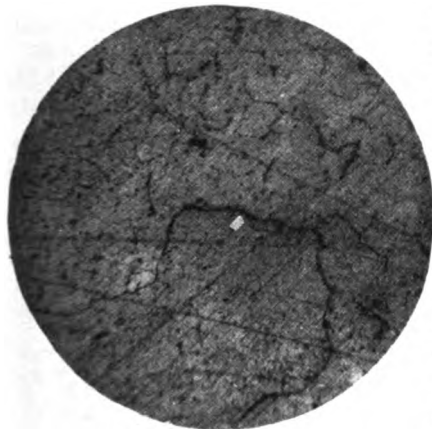
Fig. 3. Ordinary Copper Packed in Sea Sand in an Iron Pipe and Heated in Air to 800 Deg. C. for One Hour. 200 times magnification
