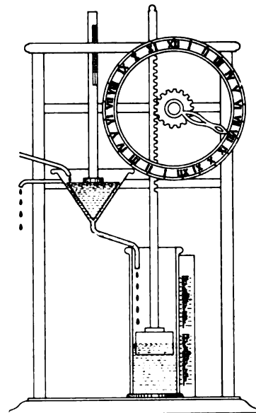
Fig. 2. Clepsydra or Water Clock
