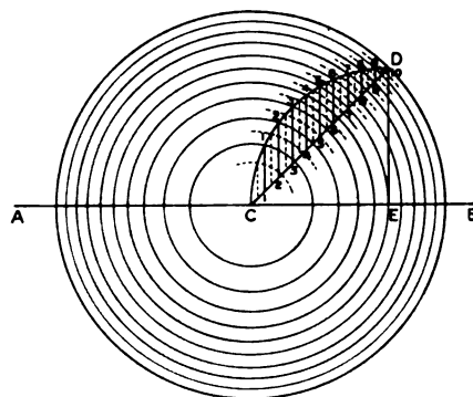
Fig. 1. Graphical Method for Dividing a Pipe into Annular Rings of Equal Areas
