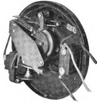
Fig. 11. Elapsed Time Switch (Open View)
