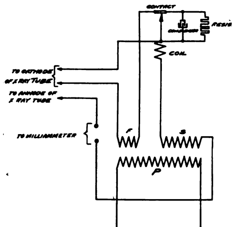
Fig. 4. Diagram of Connections. When the tube current exceeds a predetermined value, the solenoid of the Kearsley stabiliser opens the contact, thereby inserting additional resistance in the filament circuit
