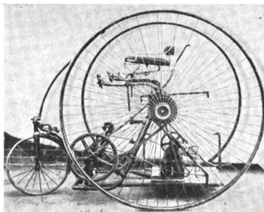
Fig. 1. The First Electric Vehicle Constructed by Fred M. Kimball, 1888
