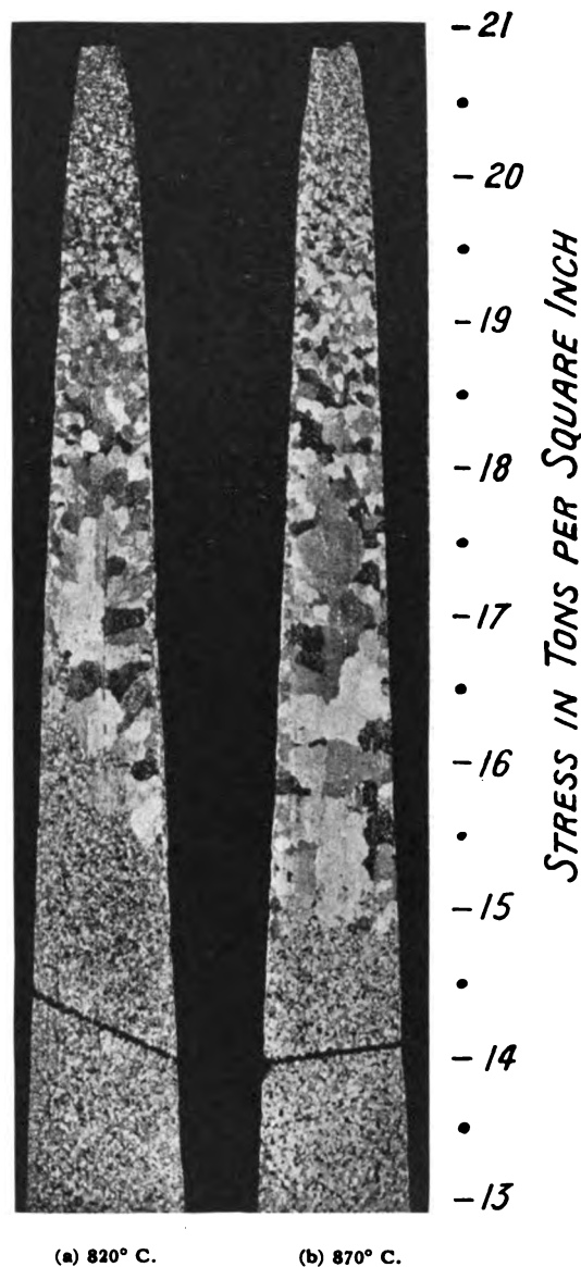
(a) 820° C. (b) 870° C. Fig. 6. Crystal Growth in Iron Rod After Tensile Test Followed by Anneal. Magnification 4.75 dia. (From Recrystallization of Deformed Iron, by Chappell. Jour. Iron and Steel Inst. Vol. 89, p. 496, Plate XLVI, 1914)
