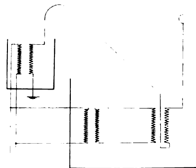
Fig. 2. Simplified Diagram of Connections of the Million-volt Set Shown in Fig. 1
