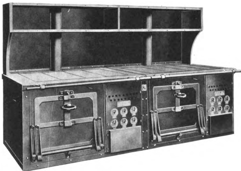
Fig. 1. A Typical Bank of Two Hotel Ranges. Separate cutouts for each unit are mounted below the switches. The cover over the cutouts is open at the bottom to permit air from the floor to circulate about the cutouts, up through the switches, and out through perforations at the top of the switchbox cover
