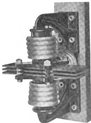
Fig. 67. Bracket Type Bus Bar Insulator
