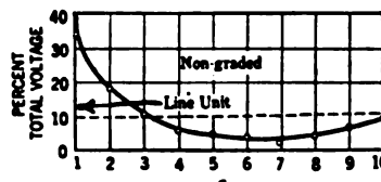
Fig. 6. Voltage Distribution on String of Ten Insulators
