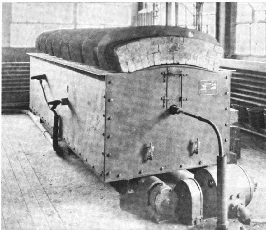
Fig. 4. 100-kw. Experimental Powder Calorizing Furnace
