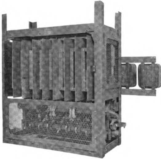
Fig. 5. Field Contactor Control Group
