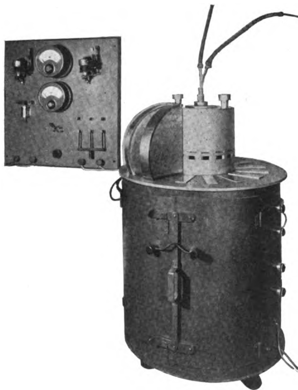
Fig. 1. X-ray Diffraction Apparatus (Doors Closed)
