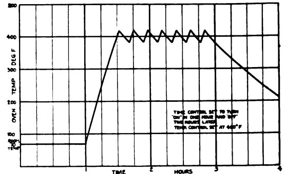
Fig. 14. Graphic Chart Showing Automatic Time and Temperature Control of Super-Automatic Range Oven
