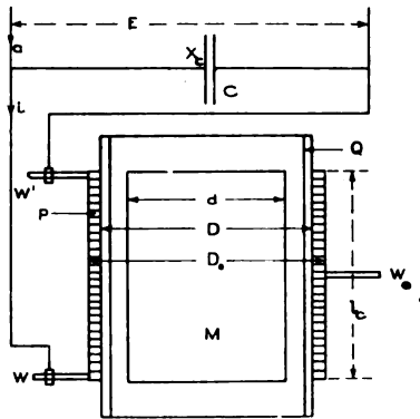
Fig. 1a. Vertical cross section of furnace
