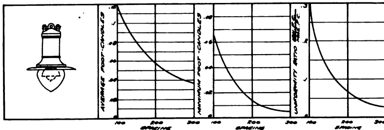
B: Novalux Pendant Unit, Dome Refractor, Clear Rippled Glass Globe with 2500-Lumen (250-c.p.) 6.6-amp. Mazda C Series Lamp. Height of Unit 25 Ft.
