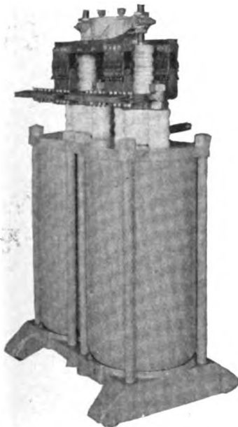
Fig. 54. Removable Single Pole Unit for Isolated Phase Arrangement
