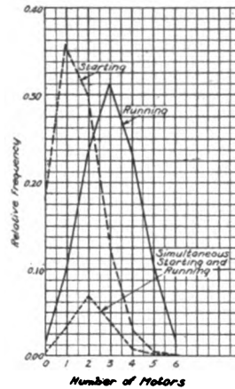
Fig. 5. Frequency Curves for Six Motors, p=0.5, p_s=0.25
