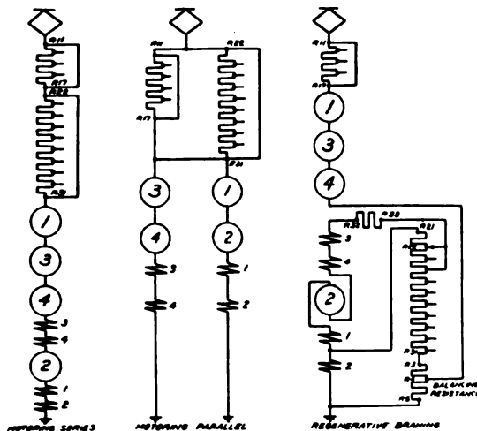
Fig. 5. Simplified Diagram Motoring and Regenerative Braking
