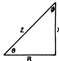
Fig. 4. Vectorial Representation of Simple Alternating-current Circuit
