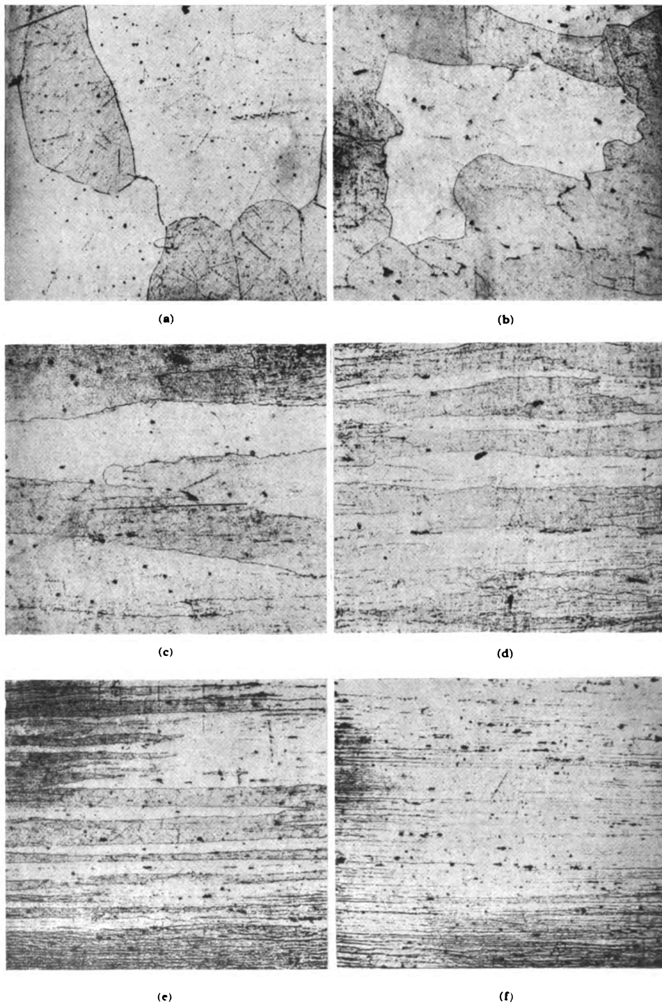
Fig. 2. Flattening of Crystals in Aluminium Sheets During Rolling. Magnification 100 dia. Reduced by \frac{1}{6} . (From Recrystallization of Aluminium Sheet on Heating, by Carpenter and Elam. Jour. Inst. Metals, Vol. 25, p. 272, Plate XIV, 1921)
