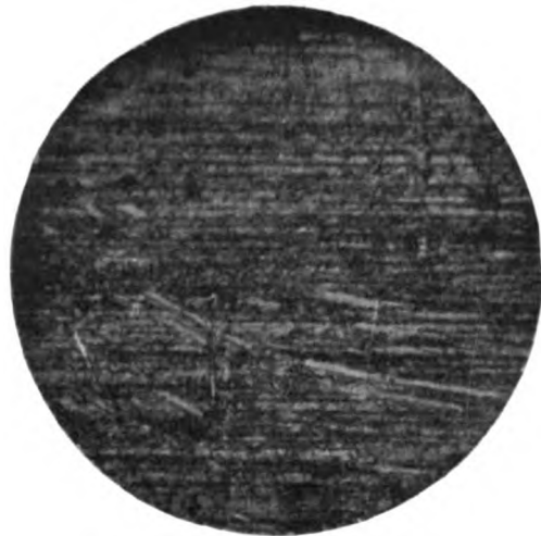
Fig. 2. Photomicrograph Showing Structure of Material in a Spring of High Fatigue
