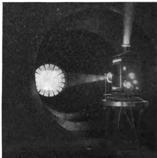
Fig. 2. Measuring the Effective Light Output of a Motion-picture Projector Lamp
