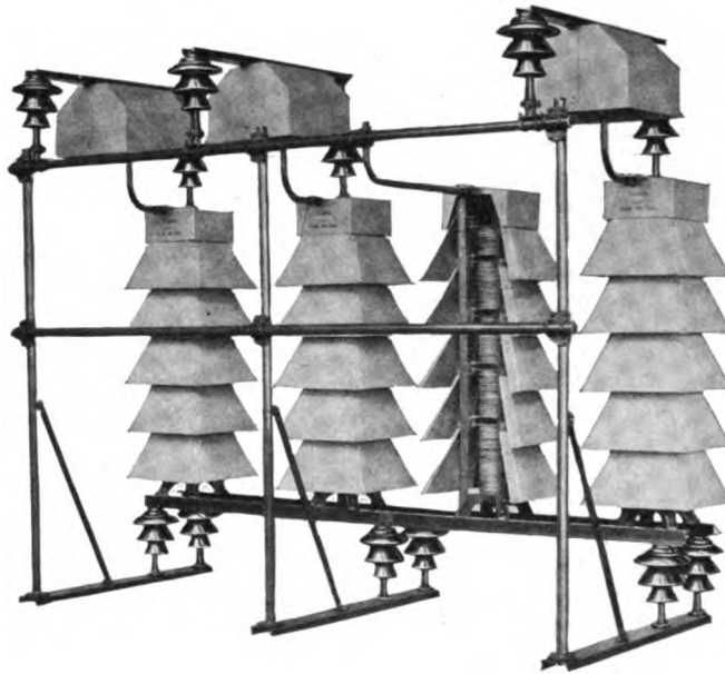
Fig. 19. Oxide Film Lightning Arrester
