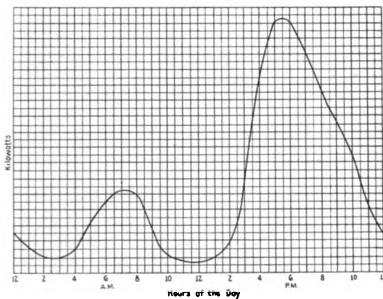
Fig. 1. General Shape of Winter Lighting Load Curve
