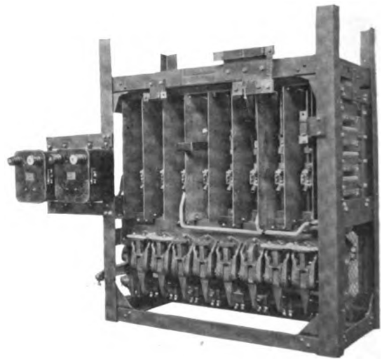
Fig. 6. Field Contactor Control Group, Back View
