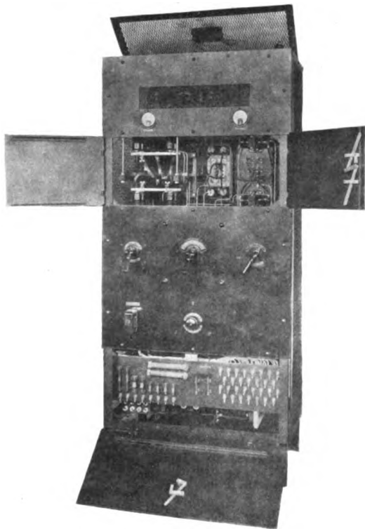
Fig. 5. Same as Fig. 4, showing Doors Open for Adjusting Transmitter
