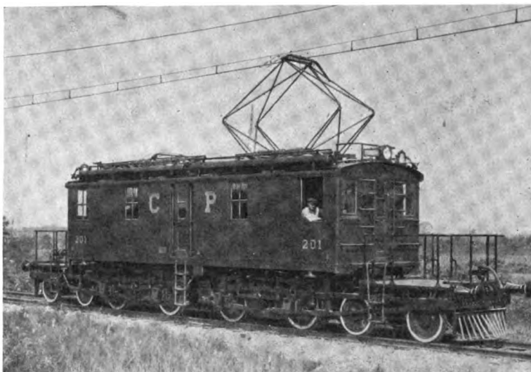
Fig. 11. 3000-volt Passenger Locomotive for the Paulista Railway
