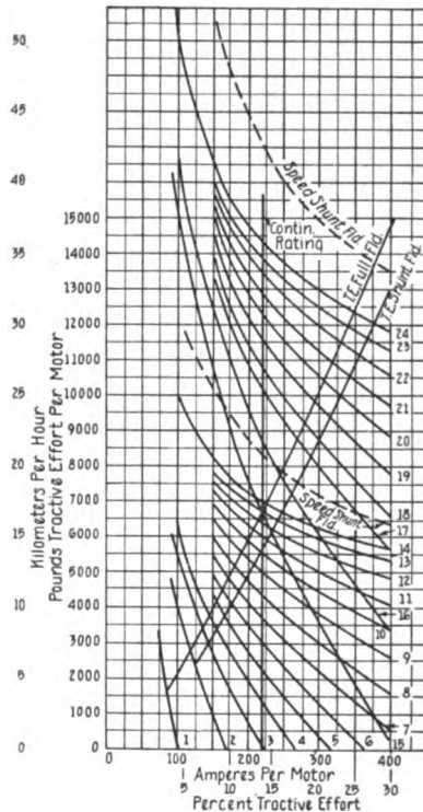
Fig. 3. Accelerating Characteristics of Freight Locomotive
