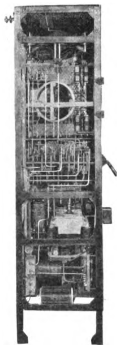
Fig. 8. Side View of Transmitter (Fig. 4) showing Arrangement of Signal Switch
