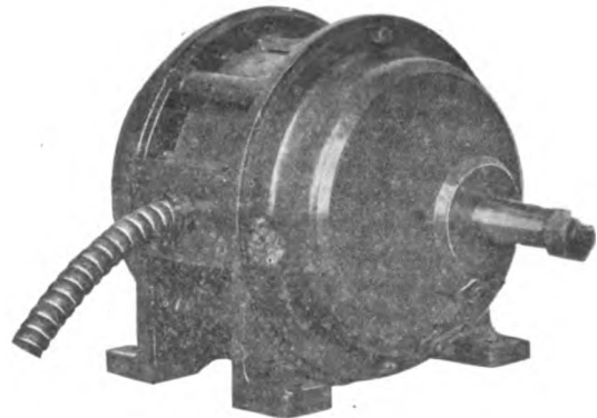
Fig. 9. Textile Type Motor for Spinning Frames
