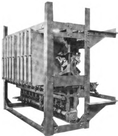
Fig. 3. Alternating-current Control Group
