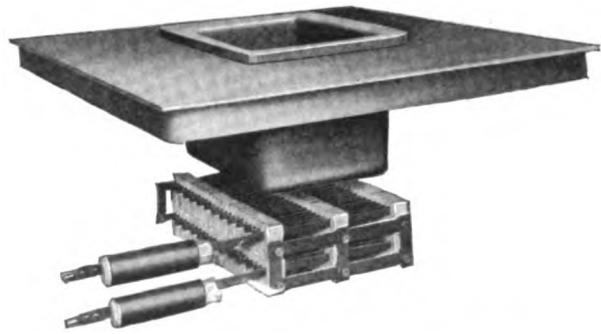
Fig. 30. Details of 1000-lb. High Temperature Melting Pot Not Bricked Up
