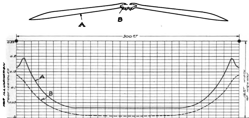
A: Novalux Highway Unit, Parabolic Nest Reflector. Height of Unit 30 Ft. B: Novalux Pendent Unit, Dome Refractor, Clear Rippled Glass Globe. Height of Unit 30 Ft. Fig. 9. Chart Showing the Relative Candle-power and Horizontal Illumination on a Road by the Novalux Highway Unit and the Dome Refractor and Clear Rippled Glass Highway Unit, Both Equipped with 2500-Lumen (250-c-p.) 6.6-amp. Mazda C Series Lamps. Illumination Calculated on Surface of Highway Along the Center Line
