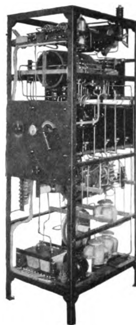
Fig. 8. Radio Panel Used in the Duplex Radio Telephone Tests
