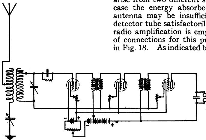
Fig. 19. Diagram of Connections for Audio Amplification
