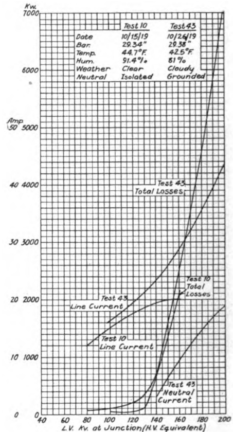
Fig. 8. Comparison of Corona Loss, Isolated Neutral (Test 10) and Grounded Neutral (Test 43). Line from Junction to Grand Rapids. No transformers at Grand Rapids. System of Consumers' Power Company
