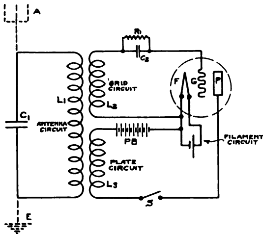
Fig. 12. Diagram of Transmitter Circuit
