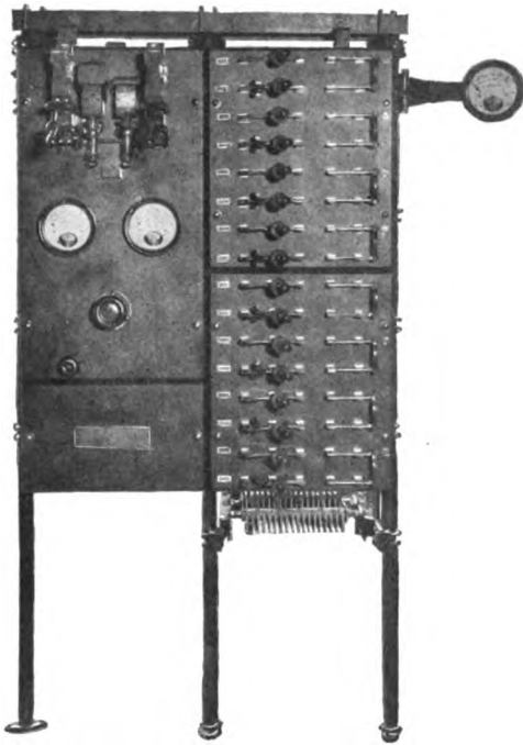
Fig. 10. Modified Constant-potential Charging Switchboard with Eight Circuits
