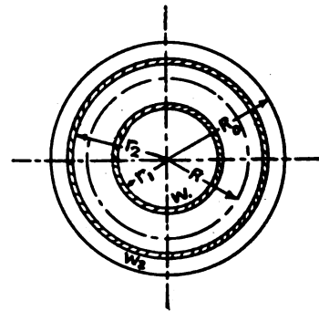
Fig. 6. Inertia of a Disc Wheel
