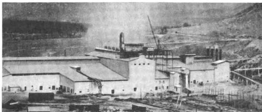
Fig. 2. Photograph Taken Before the Installation of Cottrell Precipitators at the Plant of the Riverside Portland Cement Company, California; compare with Fig. 3
