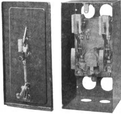
Fig. 51. 100-amp. Safety Enclosed Overload Air Circuit Breaker
