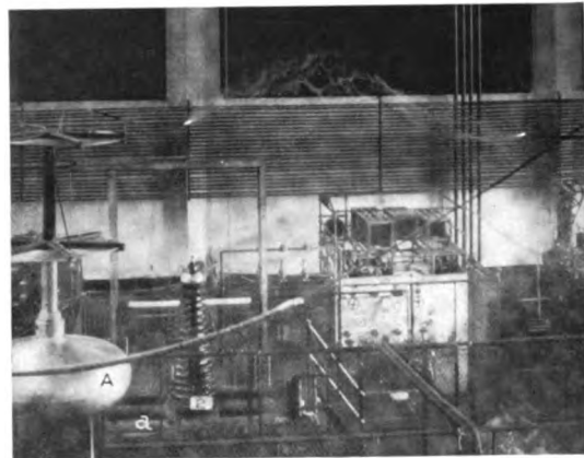
Fig. 13. Million-volt Nine-foot Arc Between Sharp Terminals. The arc shows faintly, due to second exposure of the photographic plate in daylight, and to poor focus. The letter A on the high-voltage terminal cap and letter a on the enclosing iron fence locate the ends of the arc shown in the bottom left-hand corner of Fig. 12
