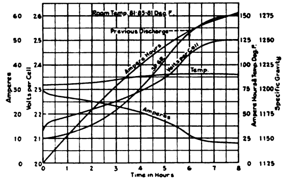
Fig. 3. Charging the Same Battery as in Fig. 2 in 8 Hours with Same Bus Voltage but Resistance Increased to 0.0665 Ohms (0.0166 Ohms per Cell). Data for these curves furnished by The Electric Storage Battery Company
