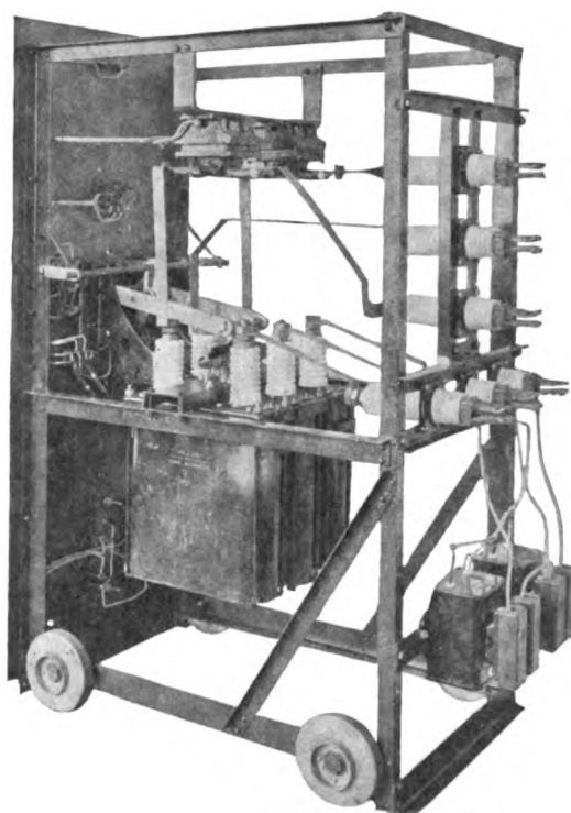
Fig. 62. Interior View of Removable Truck Switchboard Panel
