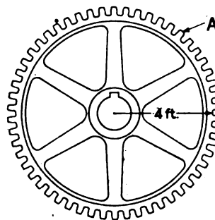
Fig. 7. Single Gear
