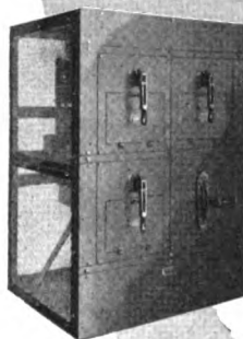
Enclosed Dead-Front Stationary Panels, especially applicable where inexperienced or unskilled employees have access to the switchboard.
