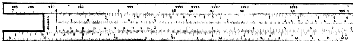
Fig. 3. Setting of Rule to Obtain Power-factor (0.80 on N Scale When R Equals 3.6 and X Equals 2.7)
