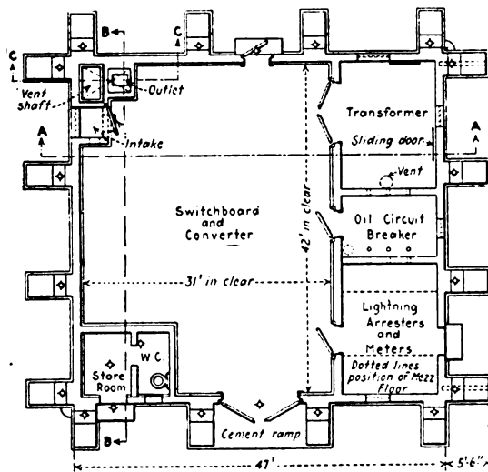
Fig. 4. Plan of Noiseless Substation
