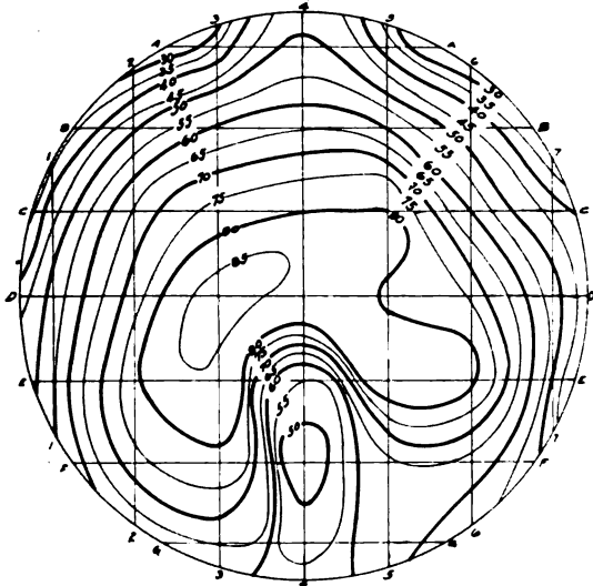
Fig. 6. Isotherms after 1 hr. 4 min. showing Rise of the Mirror Temperature above that of the Room. The test station locations are as shown in Fig. 4
