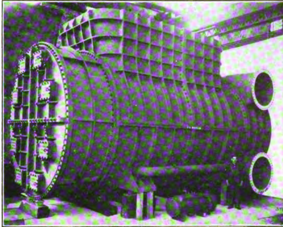
30,000 KW. SURFACE CONDENSER
