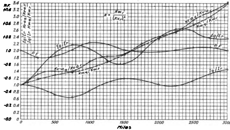
Fig. 26. 60 Cycles. Line Loaded. K=5 , Unity Power-factor
