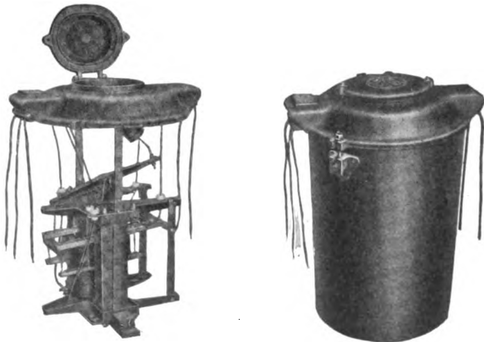
Fig. 19. Pole-type Constant-current Transformer Equipment and Its Application
