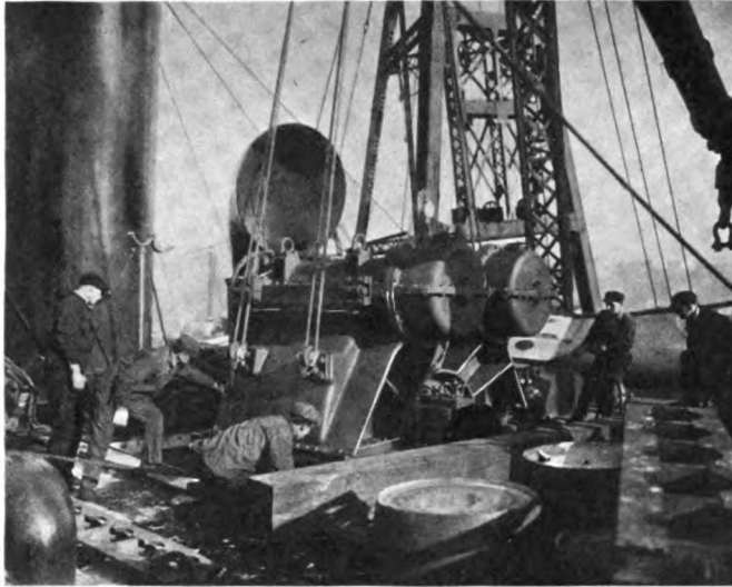
Fig. 9. Replacing a Set of One-plane Reduction Gears by the Two-plane Type in the Record Time of Ten Days
