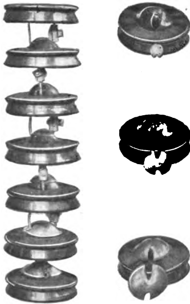
Fig. 9. Suspension Insulators Graded with Caps or Plates
