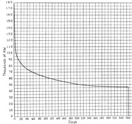
Fig. 2. Annual Load Curve
