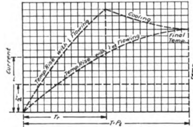
Fig. 10. Temperature conditions during a single duty cycle
