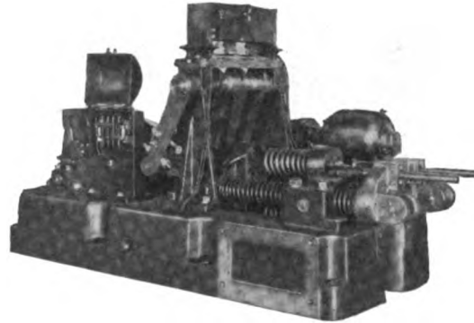
Fig. 55. Motor Operated Mechanism for Oil Circuit Breaker for Isolated Phase Arrangement
