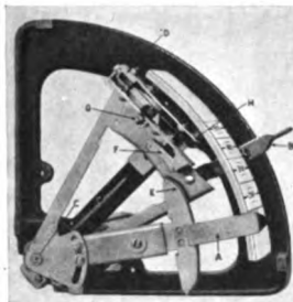
Fig. 8. Temperature Control Mechanism for Automatic Range (Open View)
