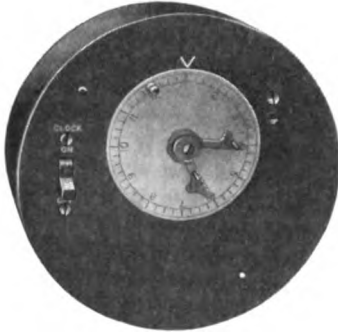
Fig. 13. Elapsed Time Switch (Front View)
