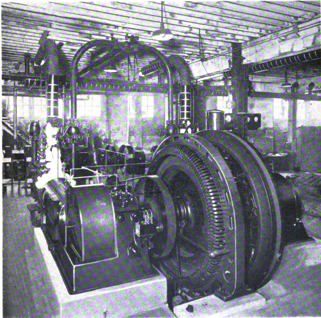
Synchronous Motor-driven Ammonia Compressor at the New Colonial Ice Corporation, New York City. This picture shows the large flywheel which was proved to be unnecessary by the tests described in the article on page 690
