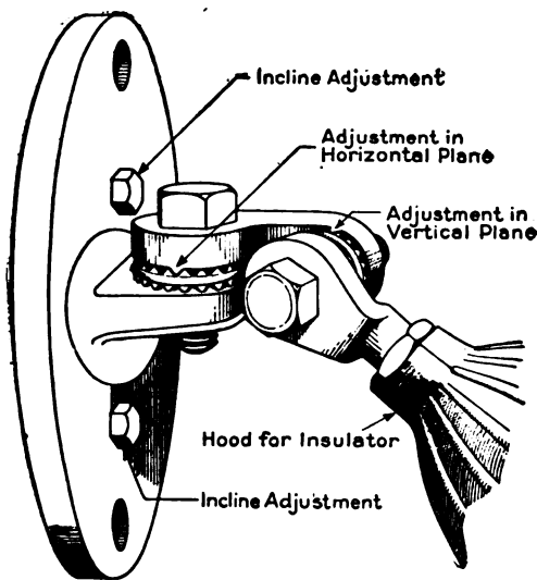
Fig. 14. Sketch of the Universal Adjustable Bracket for Novalux Highway Units
