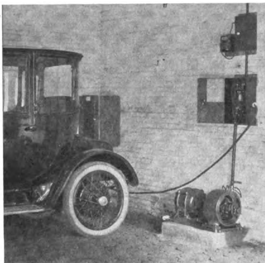
Fig. 4. Taper or Modified Constant-potential Charging Motor-generator Set in Home Garage
