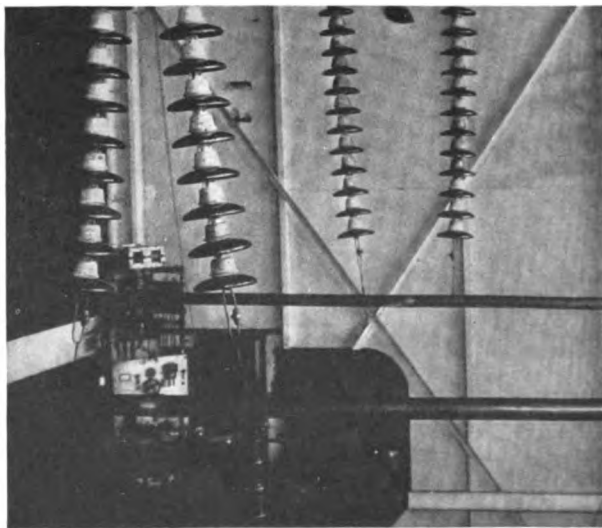
Fig. 23. Lines Insulated for One Million Volts
