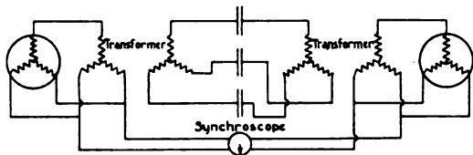
Fig. 4. Series Operation of Two Three-phase Alternators Connected with Condensive Load Through Transformers
