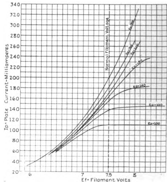
Fig. 8. Plate-current Filament-voltage Characteristic of Kenotron (UV-216)
