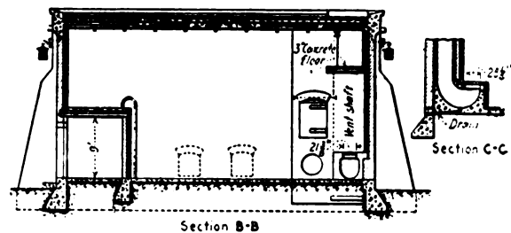
Fig. 3. Cross Sections of Noiseless Substation showing Construction of Walls and Roof
