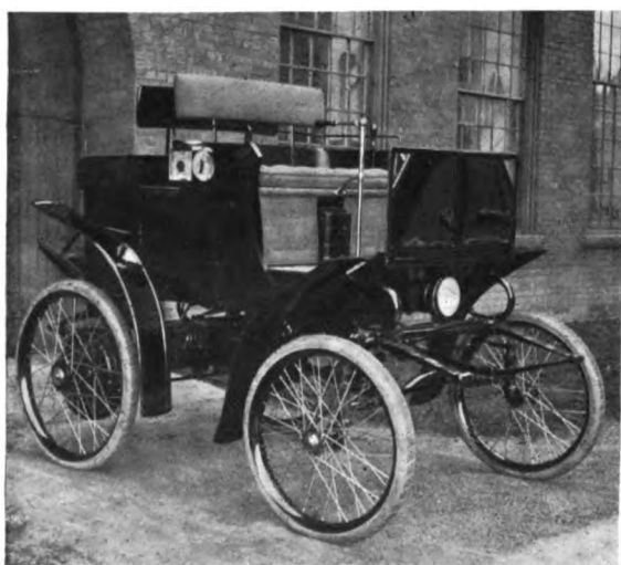
Fig. 1. Typical Four-passenger Runabout of 1898 (Columbia Electric Vehicle Company)
