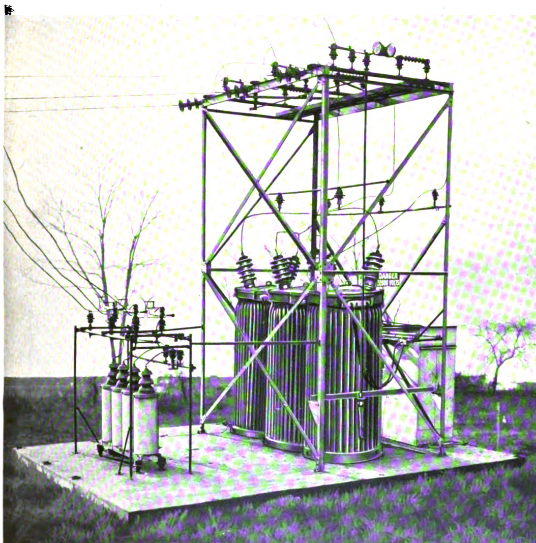
A TYPICAL SMALL CAPACITY OUTDOOR SUBSTATION
