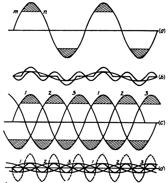
Fig. 12. Illustrating Manner of Formation of Triple Frequency Current due to Corona, Y-connected Grounded Neutral System
