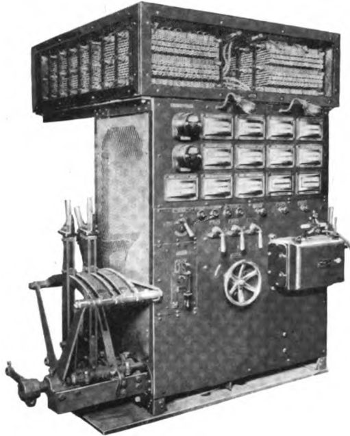
Fig. 1. Control Panel, Front View
