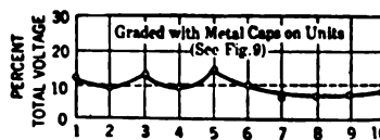
Fig. 8. Voltage Distribution on String of Ten Insulators
