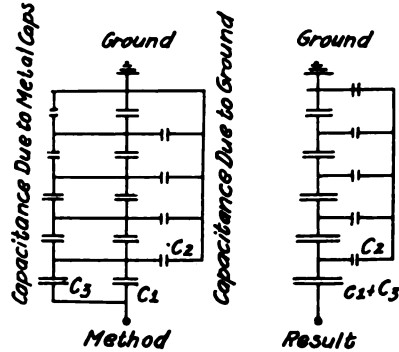
Fig. 4. Grading by Increasing Capacitance C_1 in Proportion to Current Distribution. This may be done by using varying sizes of disks and hardware or by metal caps on the disks, or by a combination of both methods
