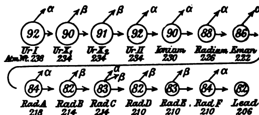
Fig. 1. Uranium Disintegration Series
