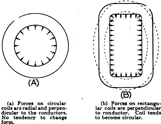
Fig. 35. Mechanical Forces on Coils. Coils carrying current tend to take form that will enclose the maximum flux
