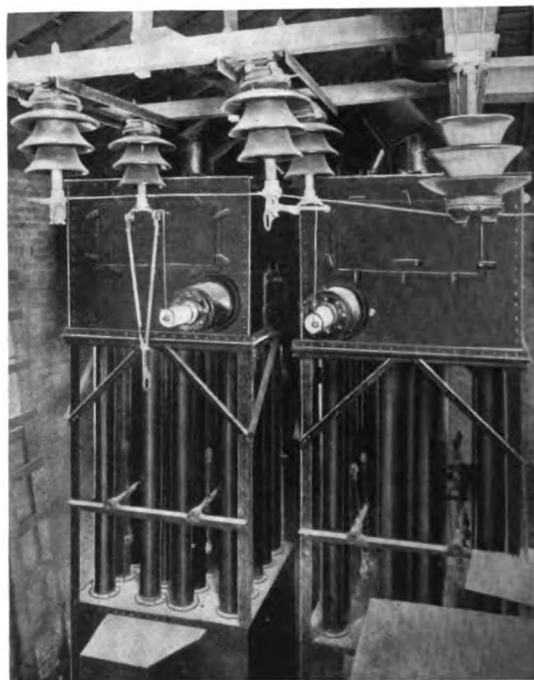
Fig. 2. Cottrell Precipitators Used in Large Scale Tests
