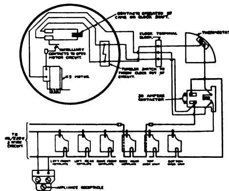
Fig. 12. Wiring Diagram of Complete Range
