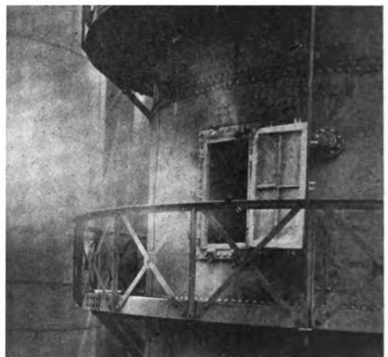
Fig. 6. Gas Issuing from Blast Furnace Precipitator When the Current is On
