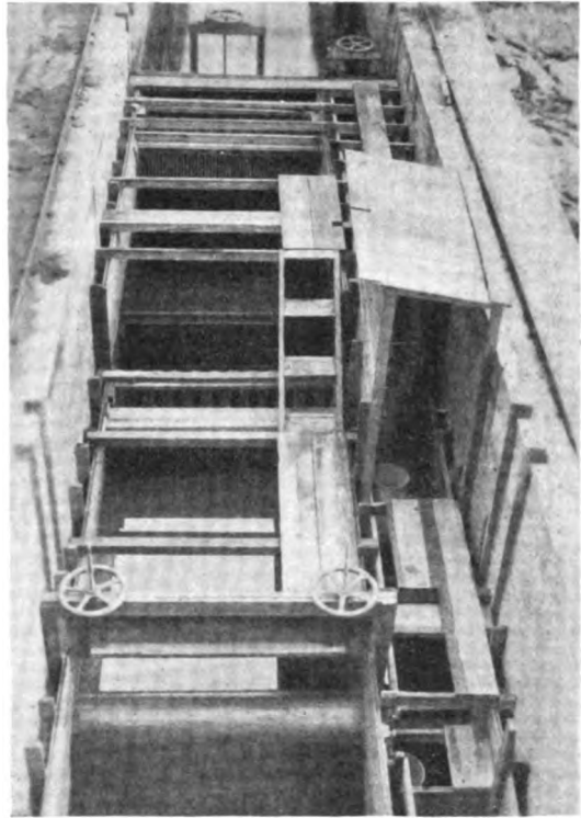
Fig. 2. General Arrangement of the Test Apparatus. The standard weirs are shown in the upper part of the illustration while the model dam (with no power-house section) can be seen in the foreground
