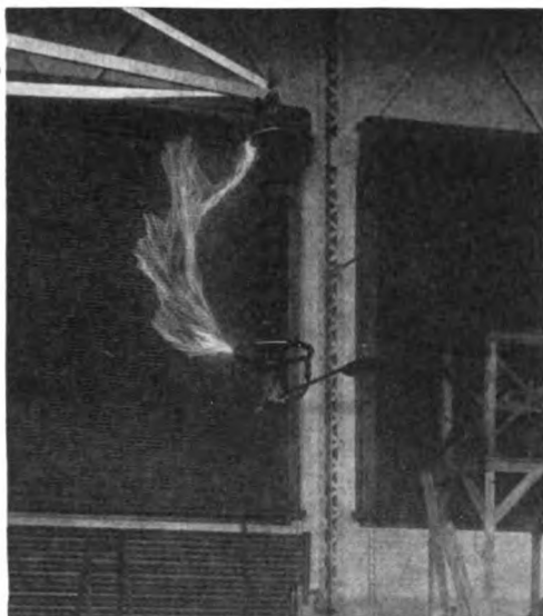
Fig. 37. Shield for Equalization of Voltage on Insulators Showing Dry 60-cycle Arc-over on a Shielded String
