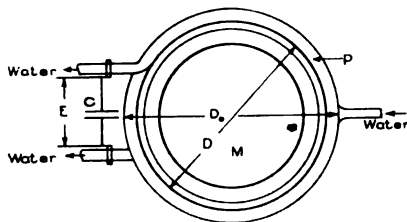
Fig. 1b. Horizontal cross section of furnace
