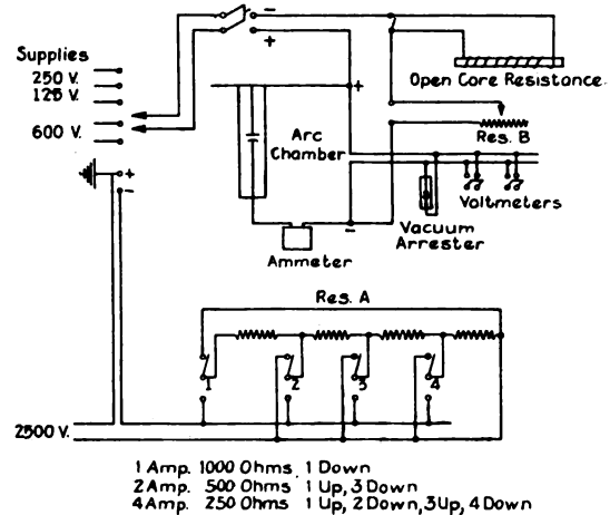
Fig. 2. Diagram of Electrical Testing Connections
