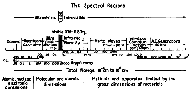
Fig. 2. The spectrum of electromagnetic waves showing the various regions and wavelengths (logarithm of wavelength is given rather than actual wavelength)
