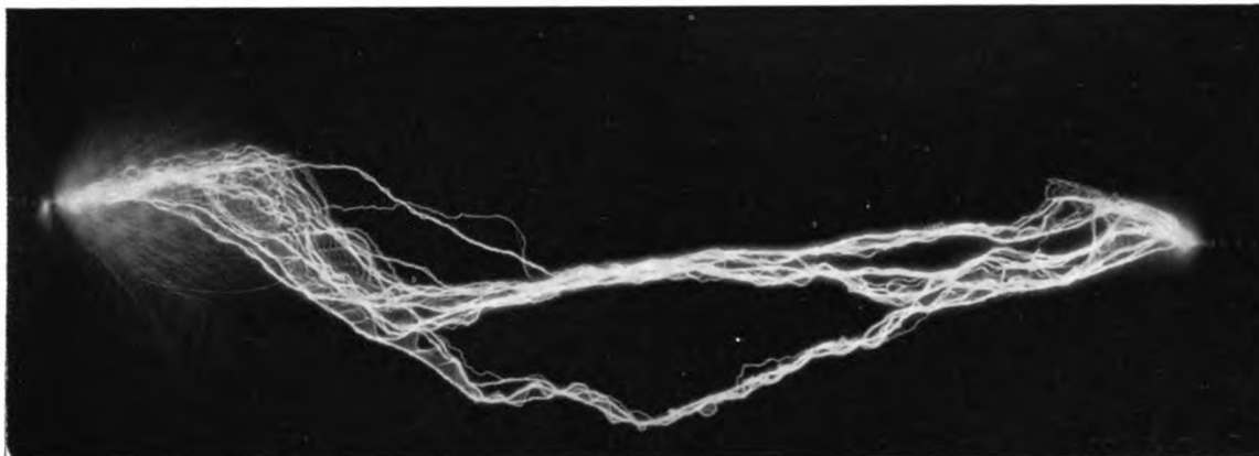
Fig. 17. Successive 1,500,000-volt Arcs over a 14-ft. Gap. The brush discharge before the spark took place shows particularly strong on the left terminal
