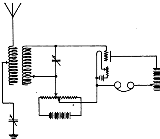
Fig. 15. Diagram of Receiver Circuit
