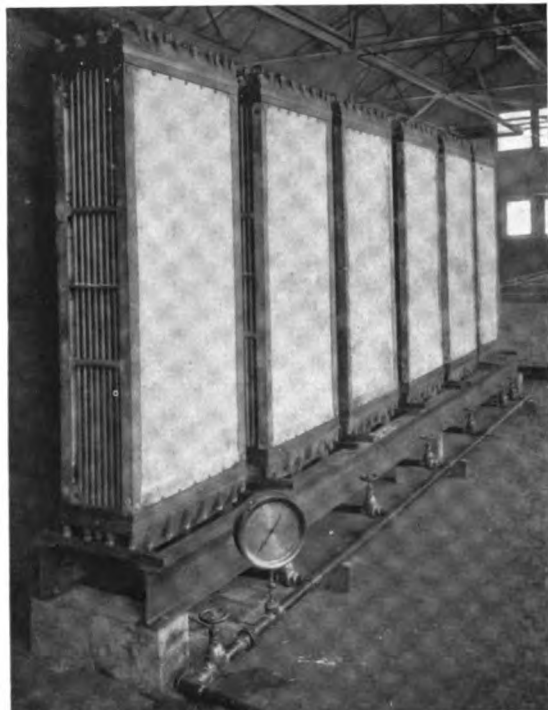
Fig. 3. Group of Surface Coolers on a Hydraulic Test Stand
