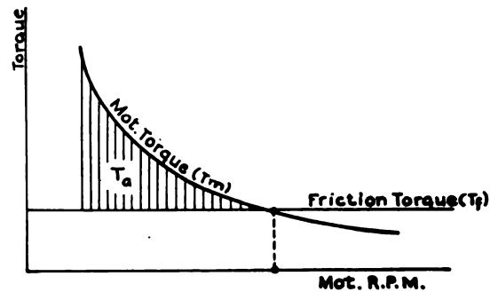
Fig. 16. Curve of Series Acceleration Period
