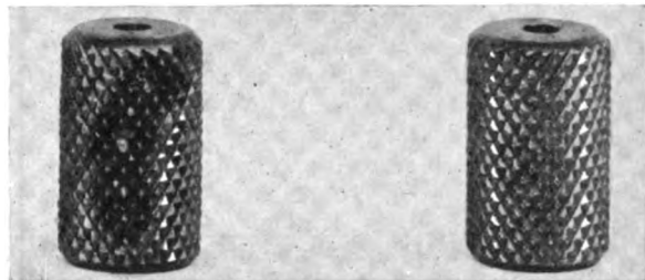
Fig. 5. After Ten Shots, Reduced Impulse and Dynamic
