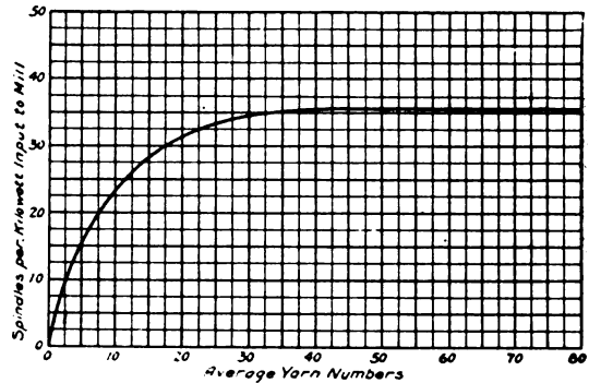
Fig. 7. Curve Showing Average Indicated Power Input to Cotton Mills
