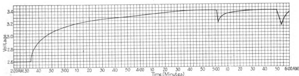
Fig. 3 and 4. Curves Showing Fluctuation of Battery Voltage as Affected by Traffic Conditions
