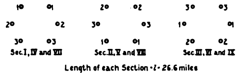
Fig. 12. The Relative Position of the Conductors in Each Section of the Southern Sierras System
