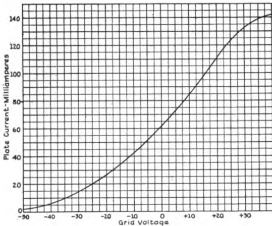
Fig. 11. Plate-current and Grid-voltage Characteristic of a Radiotron
