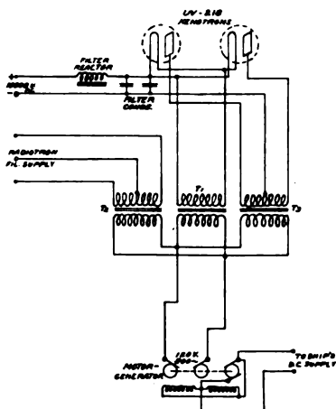
Fig. 7. Circuit Diagram of Kenotron Panel
