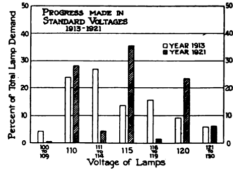
Fig. 4. Demand for Standard Voltage Lamps, 1913 and 1921
