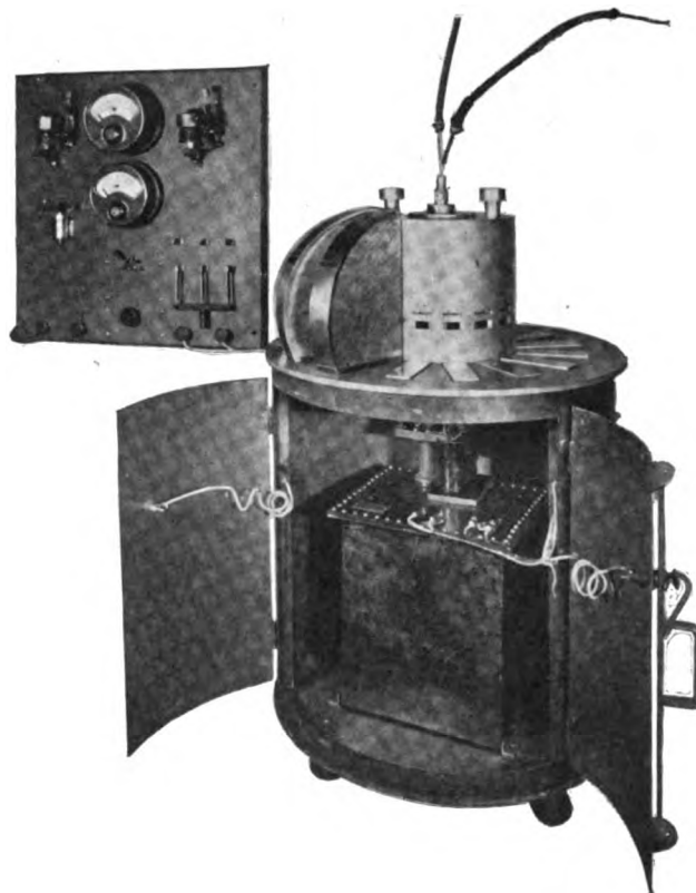
Fig. 2. X-ray Diffraction Apparatus (Doors Open)
