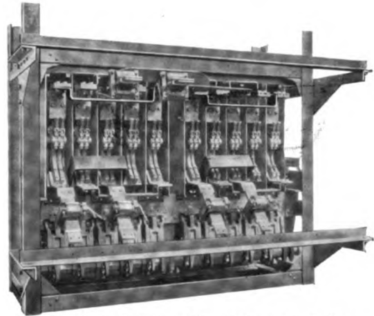
Fig. 4. Alternating-current Control Group, Back View
