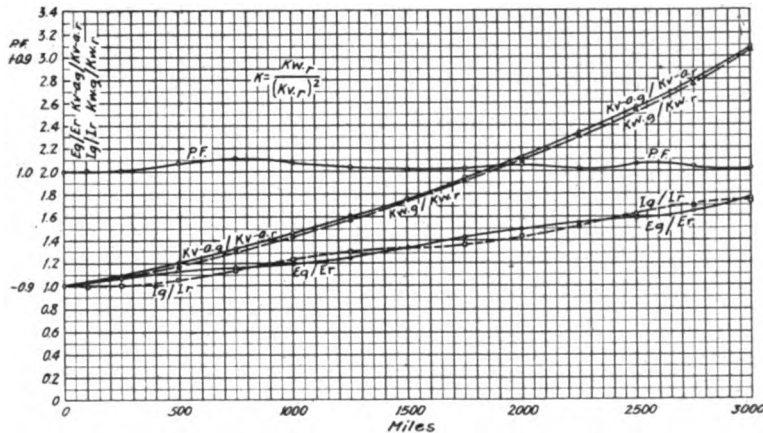
Fig. 25. 60 Cycles. Line loaded. K = 2.5 at Unity Power-factor. K = kw. rec. / (kv. rec.)^2
