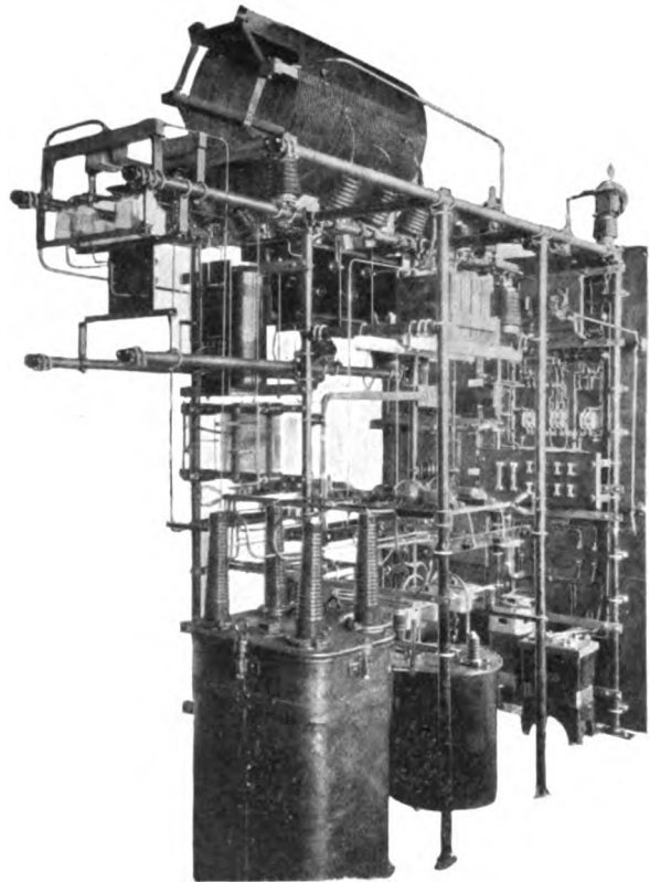
Fig. 42. 2-kw. Radio Telegraph Transmitter for "Almirante"
