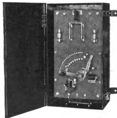
Fig. 3. Panel with Controller Segments, Switch and Fuses, Flush Mounted and Enclosed in Cabinet
