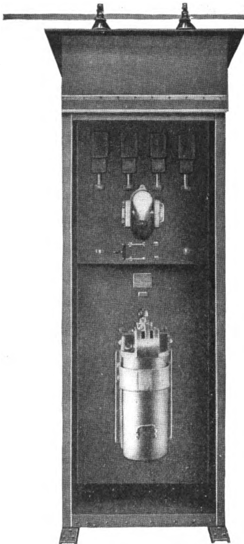
Automatic Reclosing Outdoor Substation (door removed) including oil circuit breaker, centrifugal operating mechanism, and necessary relays and instruments. Can be furnished for service on circuits from 2300 to 13,200 volts
