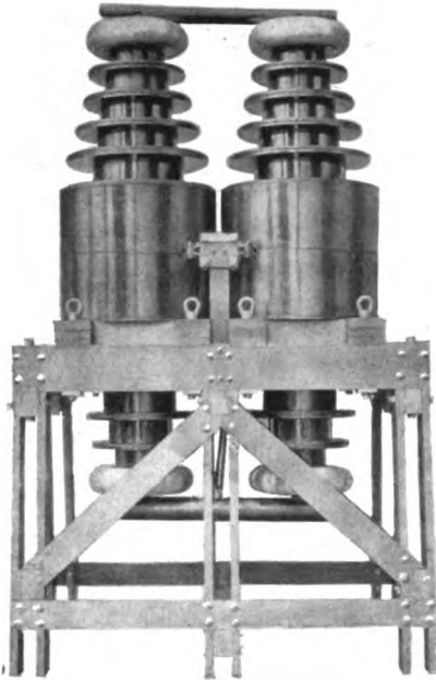
Fig. 11. Insulating Transformer Used to Excite the Line Transformer for Tests above 578,000 Volts
