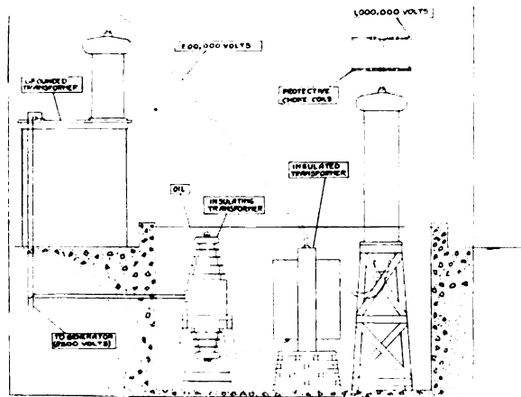
Fig. 1. General Arrangement of the Million-volt Testing Set, Showing the Main Transformer, Insulating Transformer, Line Transformer, and High-tension Bushing; the Latter Three Components Standing on Wooden Supports in a Tank of Oil
