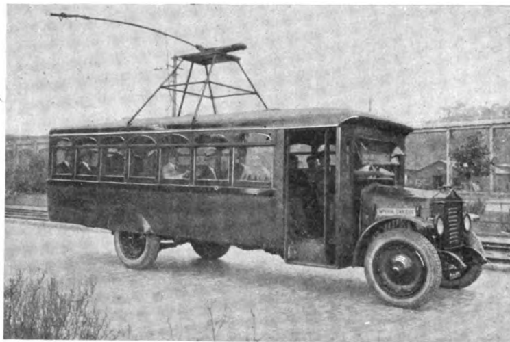
Fig. 10. Trackless Trolley Equipped with Railway Motors, Foot Control and Special Form of Collector
