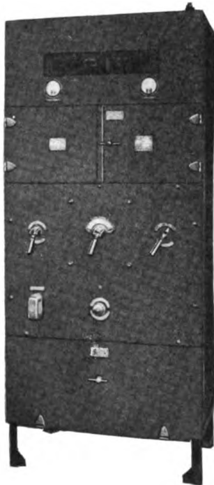
Fig. 4. 1-kw. Commercial Transmitter for Telephony, Interrupted-continuous-wave Telegraphy and Continuous-wave Telegraphy
