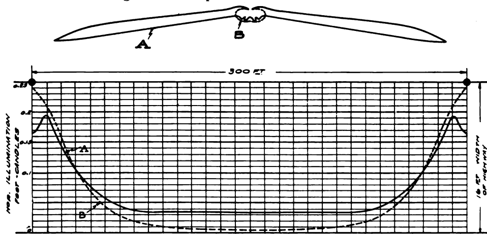
A: Novalux Highway Unit, Parabolic Nest Reflector. Height of Unit 30 ft. B: 20-in. Dome Radial-Wave Reflector, Street Hood (Steel Reflector). Height of Unit 30 Ft. Fig. 8. Chart Showing the Relative Candle-power and Horizontal Illumination on a Road by the Novalux Highway Unit and the Radial-Wave Reflector, Both Equipped with 2500-Lumen (250-c-p.) 6.6-amp. Mazda C Series Lamps. Illumination Calculated on Surface of Highway Along the Center Line
