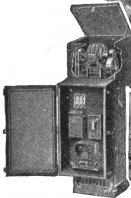
5- to 70-kv-a., 2300-volt, Automatic Regulator for Outdoor Installation
