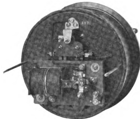
Fig. 60. Temperature Relay for Protection of Waterwheel Generators
