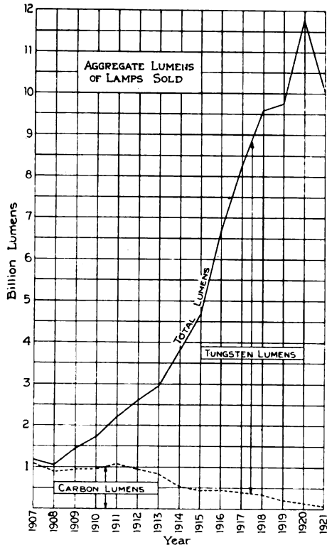
Fig. 3. Total Lumens of Lamps Sold, 1907-1921
