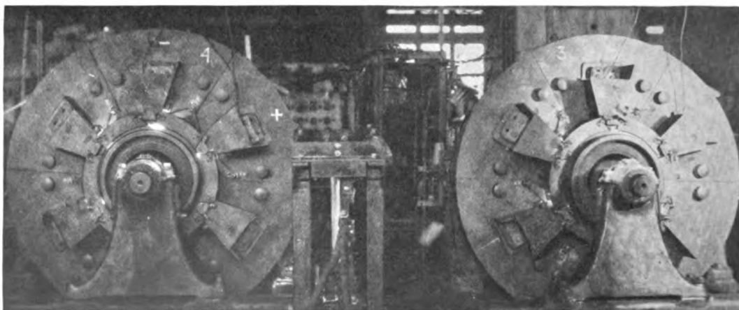
Fig. 5. Maximum Short Circuit of Two 750-volt, 60-cycle Converters Connected in Series for 1500 Volts. Machine equipped with radial brush rigging and high reluctance commutating poles and protected by flash barriers and high-speed breaker
