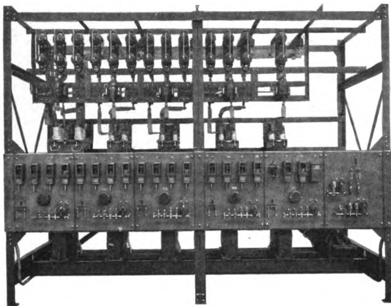
Fig. 16. 4000-volt, 60-cycle Automatic Reclosing Feeder Station
