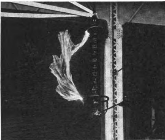
Fig. 3. Suspension Insulator String with Antenna or Shielding Ring of the Peek Type for Equalizing the Voltage
