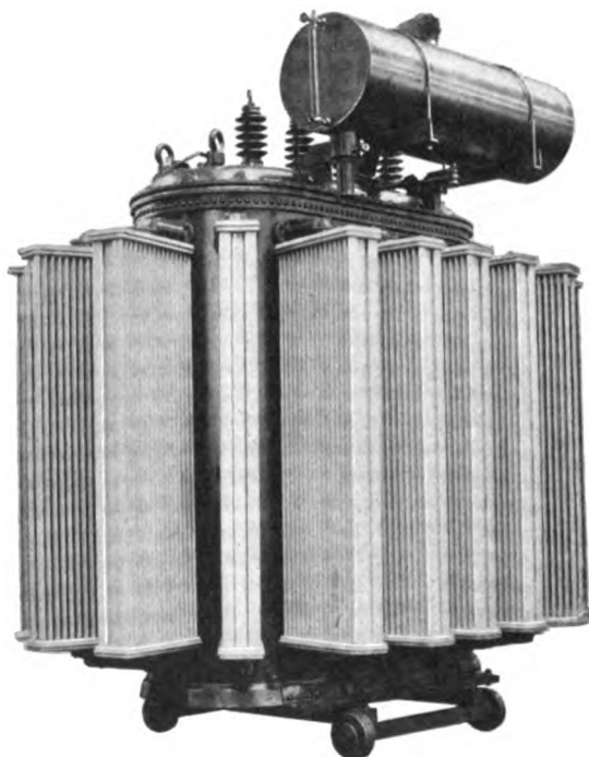
Fig. 34. Arrangement of Radiators on 10,000-kv-a. Self-cooled Transformer
