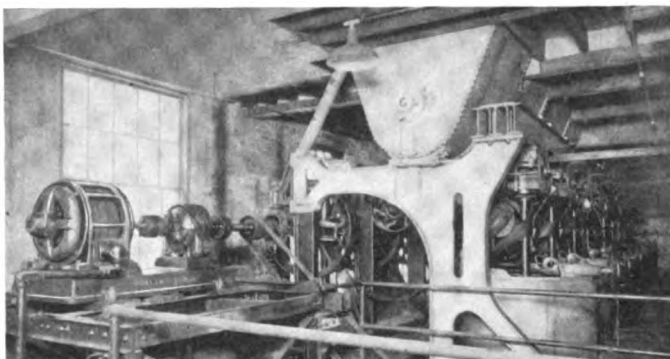
Fig. 1. Centrifugals Driven by a 50-h.p. Induction Motor Through a Reduction Gear
