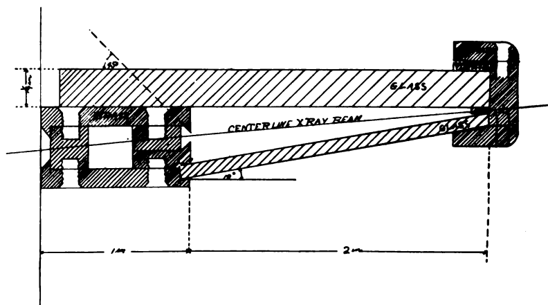
Fig. 5. Diagram of Slit System
