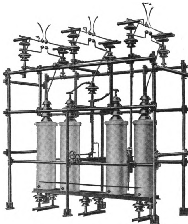
Fig. 18. Aluminum Cell Lightning Arrester
