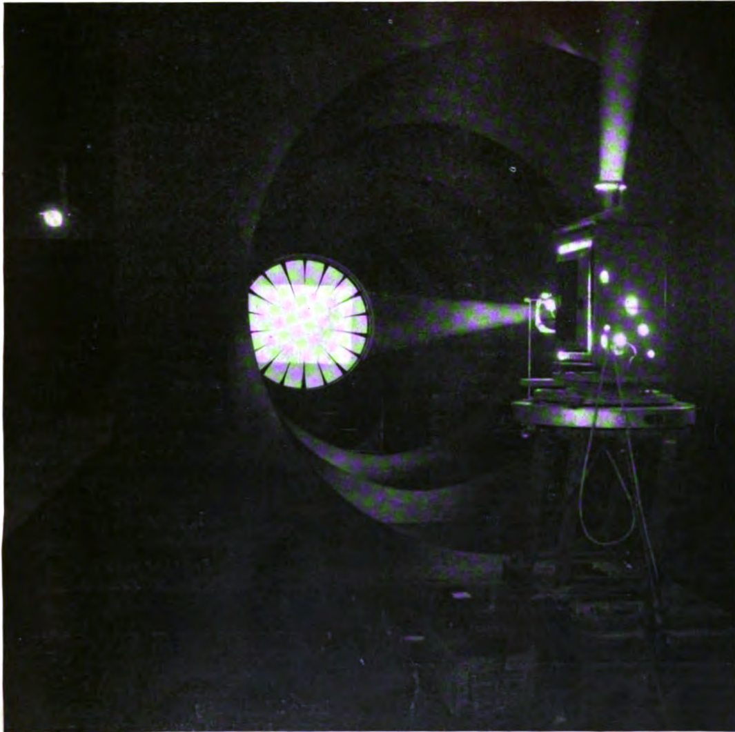
Testing a Motion-picture Projector Equipped with 120-ampere High-intensity Carbons. The light tunnel has a maximum length of 150 feet, and the 110-inch hollow white hemispherical photometer is arranged to measure the total light of the beam or that of any circular section
