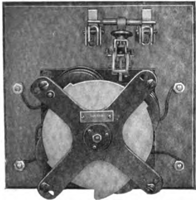
Fig. 48. Open-phase and Phase Reversal Relay
