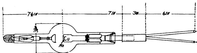
Fig. 3. Diagram of Water-cooled Coolidge Tube
