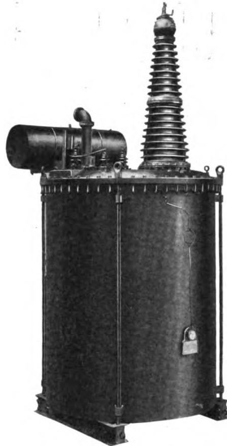
Fig. 38. Large High Voltage Transformer Equipped with Conservator
