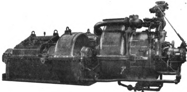
Fig. 5. Marine Geared Turbine of 2500 h.p. of the One-plane War Emergency Type
