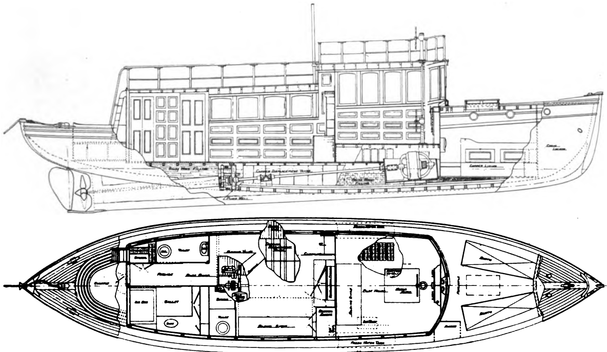
Fig. 2. General Plan of the New Era
