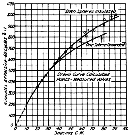
Fig. 15. Spark-over 75 cm. Spheres
