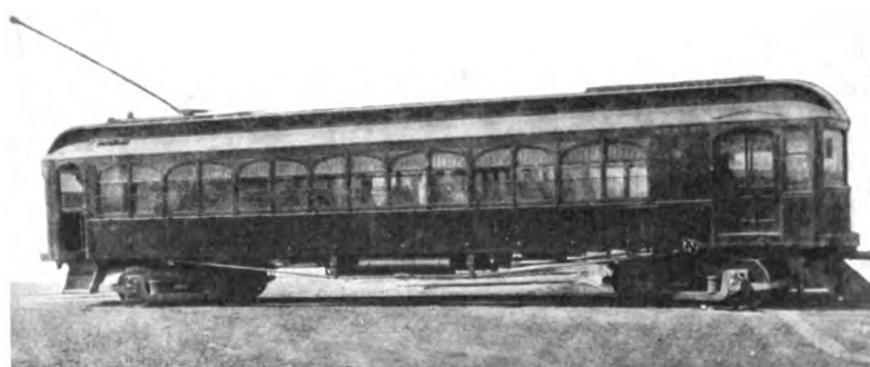
Fig. 8. Single End, 2-man, 52-passenger, 3-compartment, 36-ton Car of Kentucky Traction & Terminal Company, Replaced by 12.5-ton, 1-man Car, Shown in Fig. 6
