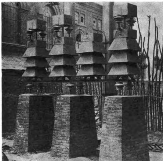
Fig. 3. 37,000-volt, 3-phase, Outdoor Type Oxide Film Lightning Arrester, Chee Hsin Cement Company, Ltd., Tongshan, North China
