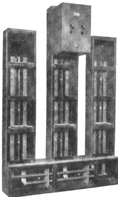
Fig. 65. Enclosed Sectional Switchboard with Front Plates Removed Showing Arrangement of Bus Bars
