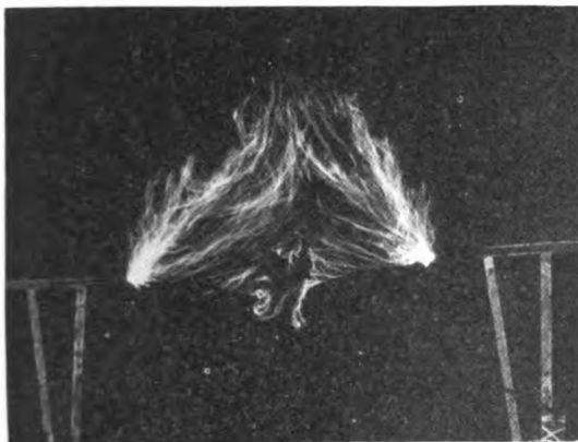
Fig. 18. Spark-over Between Needle Points at One Million Volts. Distance about nine feet
