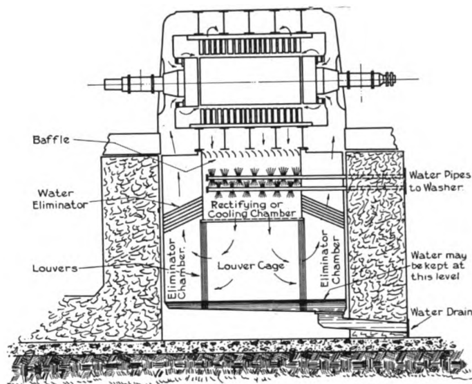
Fig. 1. Diagram Illustrating the Closed Air Circuit System of Ventilation, for Cooling Steam Turbine Generators
