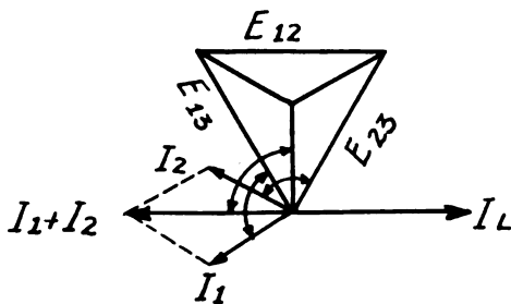
Fig. 16. Vector Relation of Currents in Circuit of Fig. 15, Angles Marked by Arrows=90°
