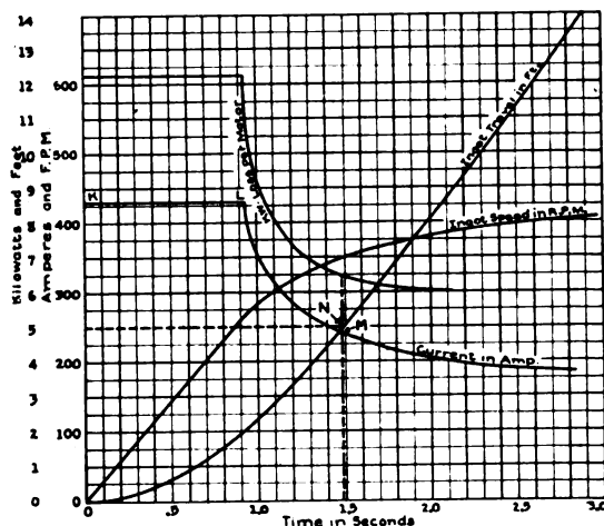
Fig. 19. Performance Curves of the Live Table Drive
