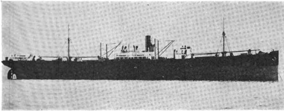
Fig. 11. S. S. Eclipse , 15,000 Tons Displacement, the First Electrically Driven Cargo Vessel. Her War Emergency Gears Having Been Replaced by General Electric, Electric Drive Machinery
