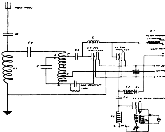
Fig. 10. Circuit Diagram of the Radio Panel
