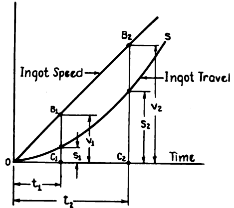
Fig. 17. Distance-time Curve for Contactor Acceleration Period
