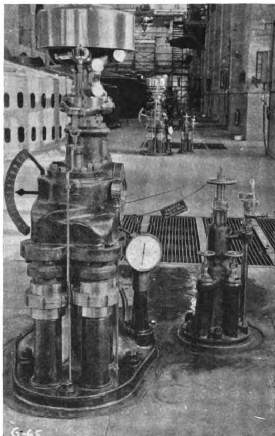
Fig. 8. A Hold-off Sign, Chain, and Lock which prevent the operation of either the governor or the hand controls. The turbine gates are half-way open to prevent the formation of an accumulation of headgate leakage that might move the rotating element
