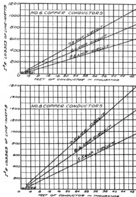
Fig. 15. Line Loss of No. 6 and No. 8 Conductor for 5.5-, 6.5-, and 7.5-amp. Circuits of Various Lengths
