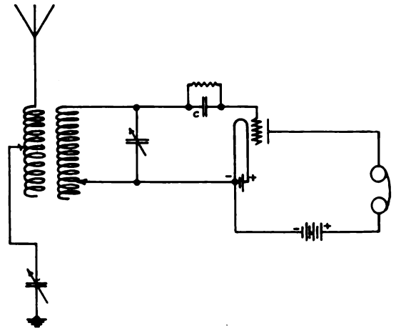
Fig. 17. Diagram of Connections for Rectification by Grid Condenser
