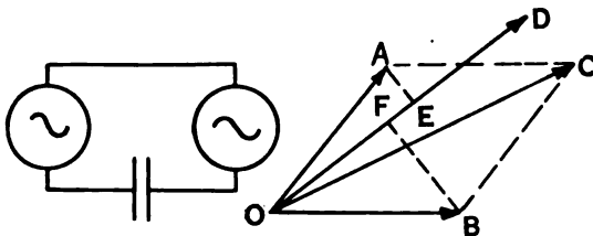
Fig. 1. (Left) Series Operation of Two Single-phase Alternators with Condensive Load
