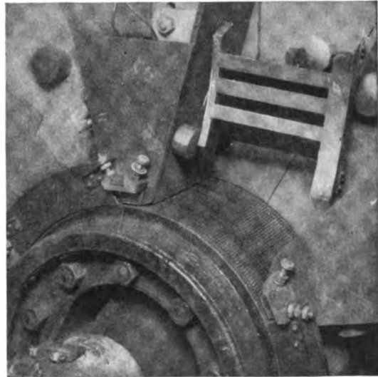
Fig. 6. Barrier Removed for Inspection After 50 Maximum Short Circuits as Shown in Fig. 5
