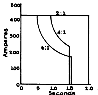
Fig. 21. Motor Current During Acceleration Period as Affected by the Gear Ratio
