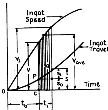
Fig. 18. Distance-time Curve for Series Acceleration Period
