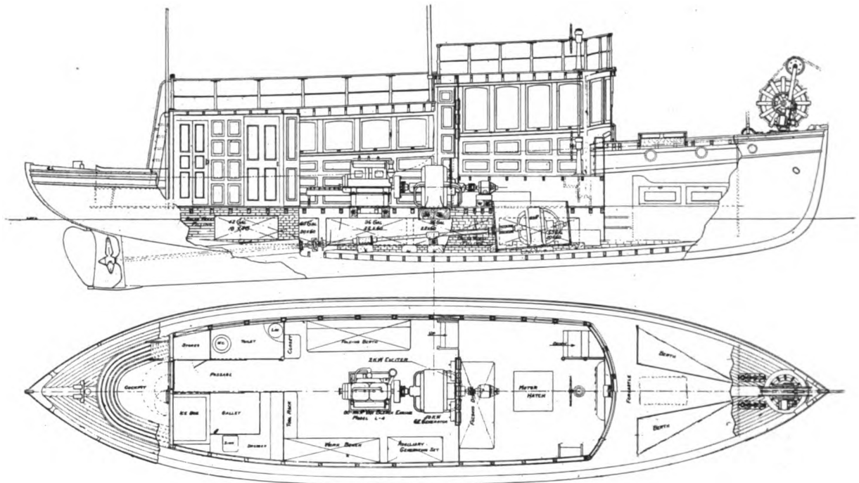
Fig. 1. Construction and Accommodation Plan of the Dawn
