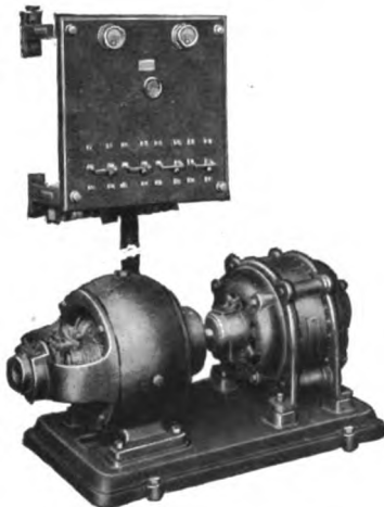
AC to DC battery charging motor-generator set with four circuit panel
