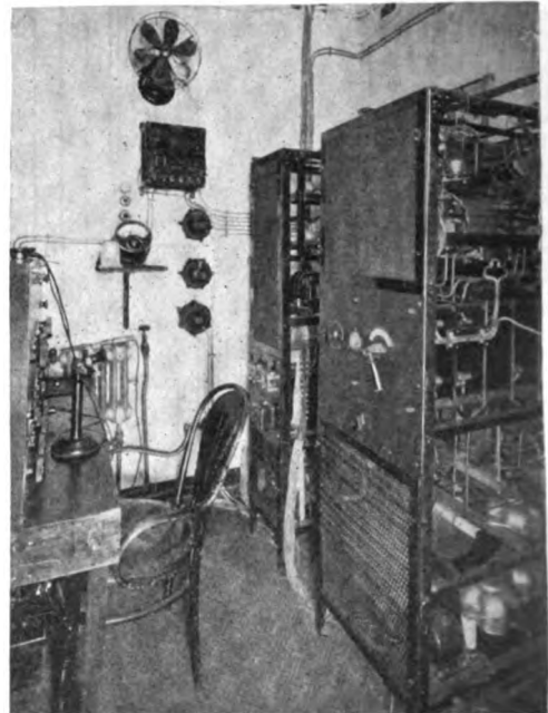
Fig. 3. Installation of Duplex Radio Apparatus on Board the S. S. America
