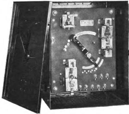
Fig. 5. Direct-current Remote-control Self-starting Speed Regulator for Blowers, Combined Armature and Field Control. Automatic self-starting type for remote operation by push buttons. Controller arm can be set for any desired predetermined speed
