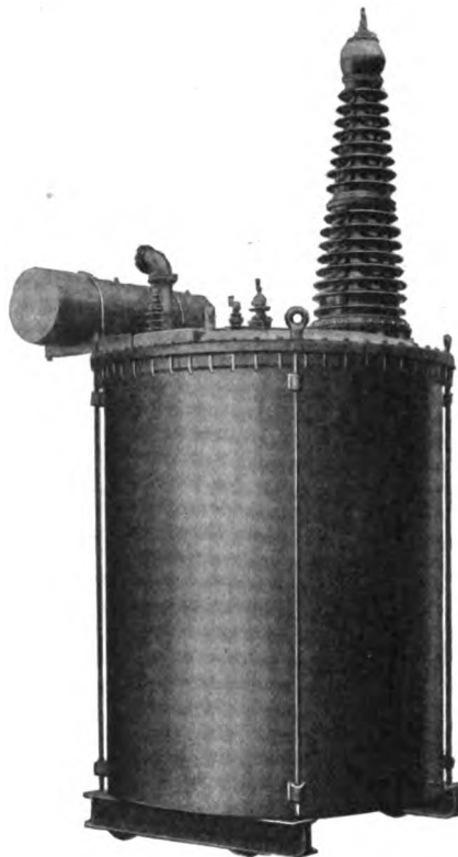
Fig. 32. High Voltage Side of 220,000-volt Transformer
