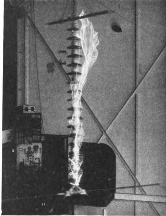
Fig. 24. Insulator Spark-over at About 900-kv.
