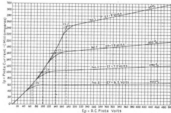
Fig. 7. Plate-current Plate-voltage Characteristic of Kenotron (UV-216)
