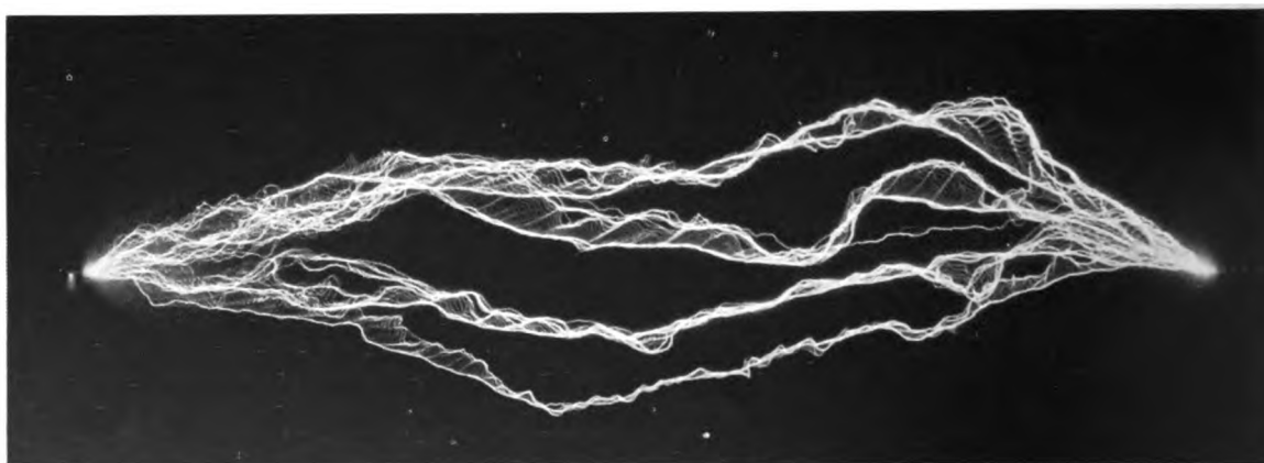
Fig. 16. A Record of Successive 1,500,000-volt Arcs Over a 14-ft. Gap
