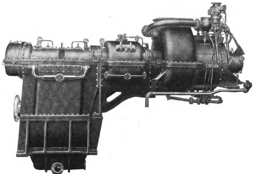
Fig. 7. Latest Type of G-E Marine Geared Turbine with Two-plane Type Reduction Gears
