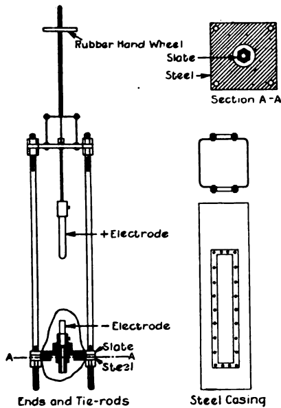
Fig. 1. Arc Chamber Used for Tests
