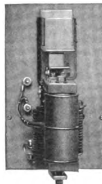
Fig. 47. 300-amp. Gap Adjusted Plunger Type Series Contactor
