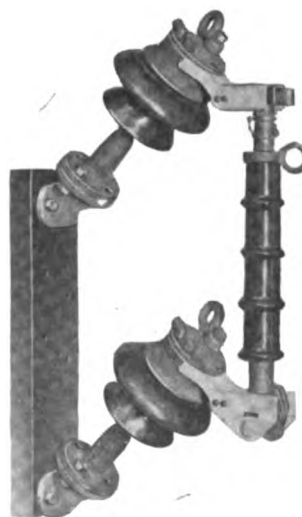
Fig. 68. Fuse Cutout, 15,000-volt 50-ampere
