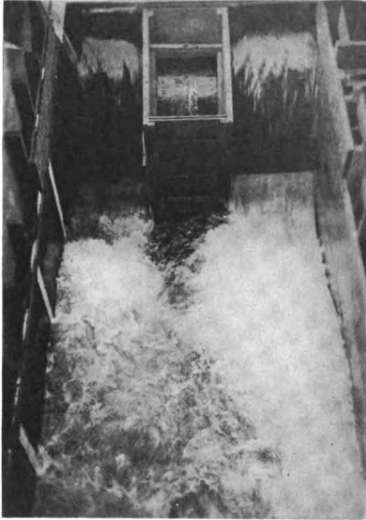
Fig. 3. A View of the Model in Operation showing the draft tube in the center at the end of the section
