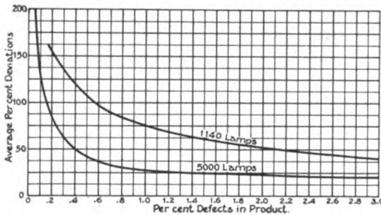
Fig. 5. Average per cent deviations resulting from 10 per cent samplings of two groups of lamps having varying proportions of individual defects
