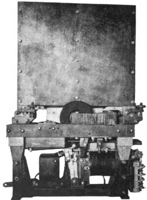
Fig. 11. Locomotive High Speed Circuit Breaker
