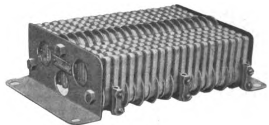
Fig. 10. Standard Cast Grid Resistance Box
