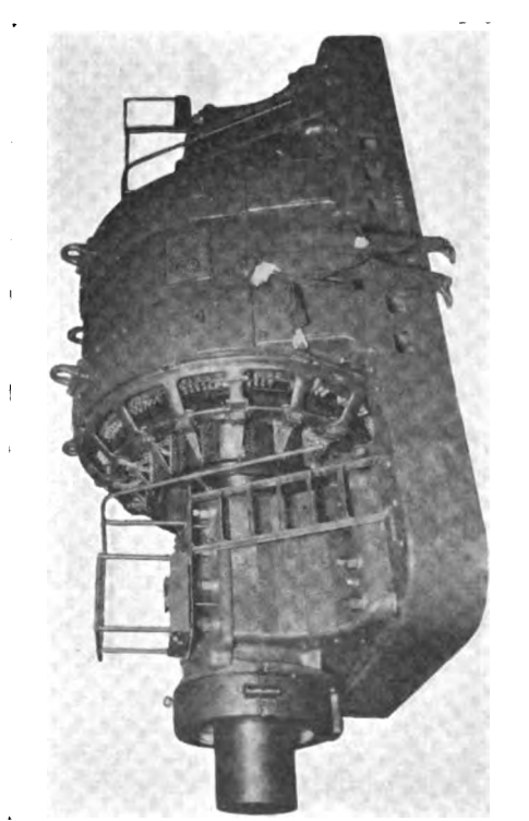
Fig. 18. 200-kw. Synchronous Converter with Automatic Control in Drifton Colliery of Lehigh Valley Coal Company
