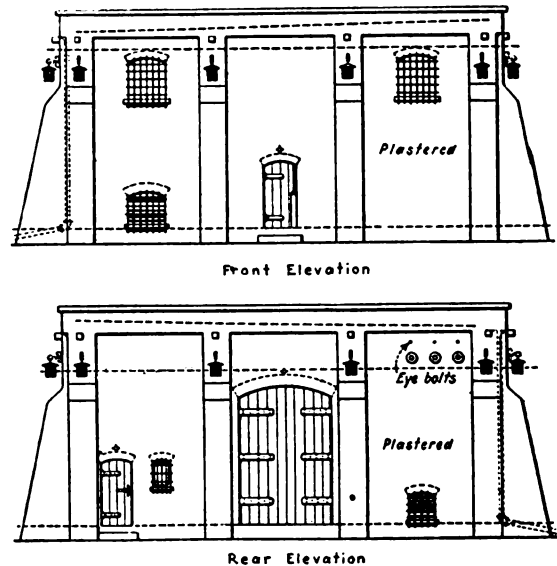
Fig. 5. Elevations of Noiseless Substation showing Heavy Buttresses and Doors
