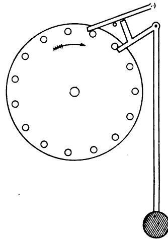
Fig. 4. Pin Wheel Escapement (Galileo)
