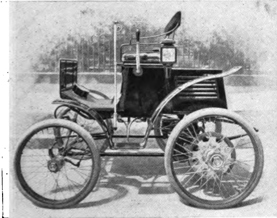
Fig. 2. Runabout of 1900 (The Riker Electric Vehicle Company)
