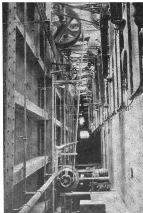
Fig. 3 50-h.p. Induction Motor Driving 33 Staking or Softening Machines
