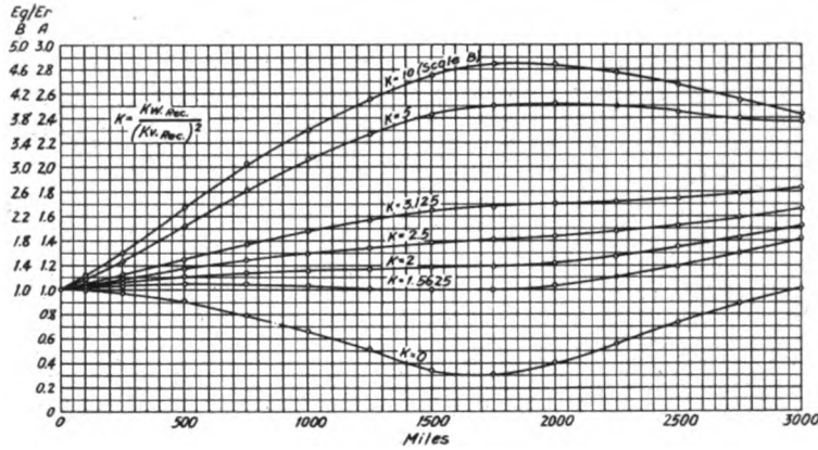
Fig. 32. 25 Cycles. Summary of Ratio E_g/E_r for Loads from Zero to K = 10
