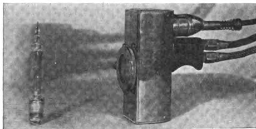
Fig. 70. Water-cooled Quartz Arc Outfit and Burner
