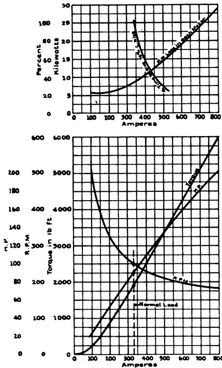
Fig. 13. Performance Curves of Two 90-h.p., 500-r.p.m., 230-volt Series-wound Motors Connected in Series and Operating on One Shaft
