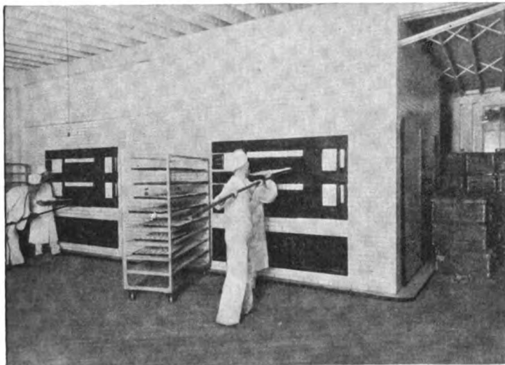
Fig. 14. A Typical Installation of Electric Brick Ovens. This bank has a total capacity of approximately 1200 one-pound loaves per hour
