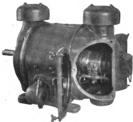
Fig. 6. 10-h.p., 1700-r.p.m. Enclosed Self-ventilated Marine Motor
