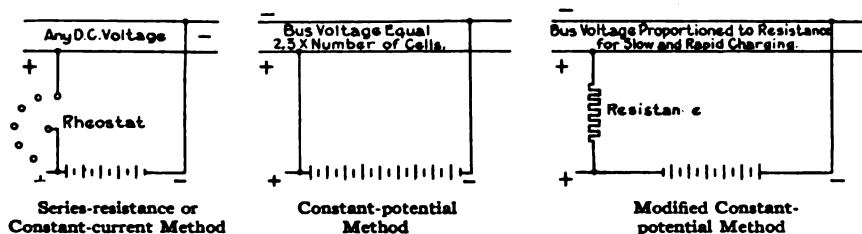
Fig. 1. Elementary Diagram of the Three Prominent Charging Methods
