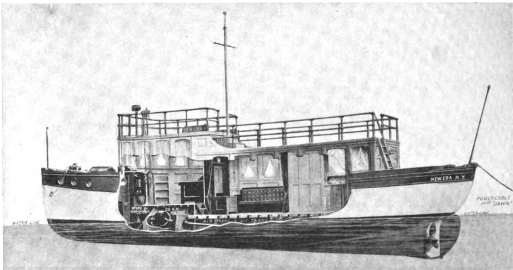
Fig. 3. Propelling Machinery of the New Era
