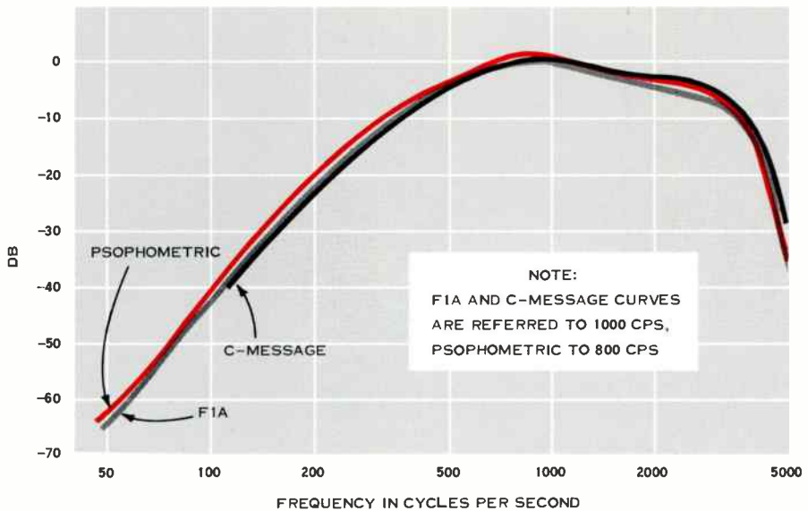
Figure 5. Weighting curves in common use indicate how noise at the band edges affects unweighted measurements out of proportion to its actual interfering effect.
