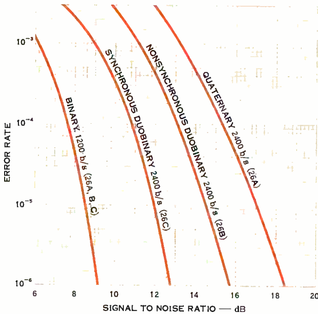
Figure 4. Comparison of error rate versus signal-to-noise ratio. Without normalization synchronous Duobinary has a noise penalty of about 3.4 dB compared to binary. This is a marked increase in performance over nonsynchronous Duobinary and quaternary.
