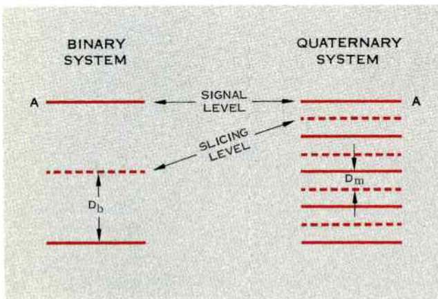
Figure 3. Determining noise penalty compared to binary. Because multilevel systems require more slicing points than binary systems, they are more susceptible to errors caused by noise.
