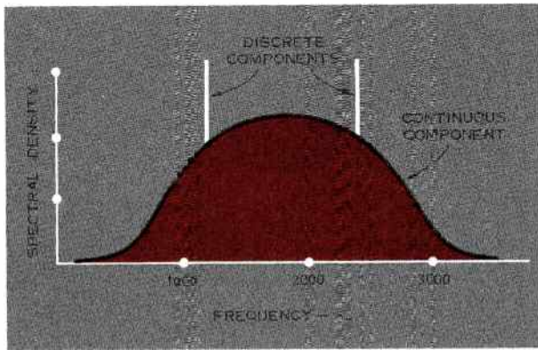
Figure 5. Spectral distribution of a binary FM signal. Discrete components present in the binary signal represent wasted power; these are not present in the synchronous Duobinary signal.
