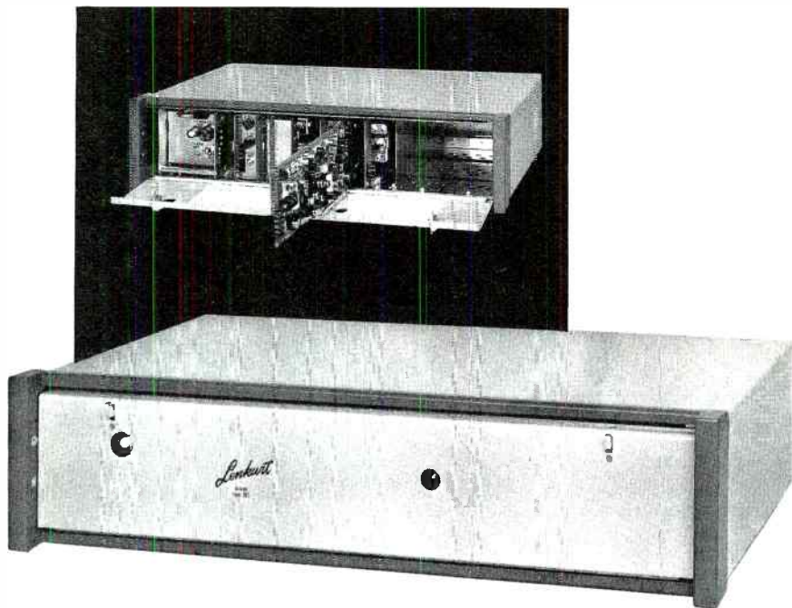
Figure 6. A typical data set shown here is Lenkurt's 26C which transmits serial digital data over standard 3-kHz voice channels at 1200 or 2400 bits per second. Other practical applications include telemetry, digitized voice or facsimile data transmission, and air-to-ground data communications over UHF or VHF radio links. Transmission at 2400 bits per second is achieved through the use of the Lenkurt synchronous Duobinary coding technique. Low error rate coupled with automatic error detection are added features of the Duobinary technique.
