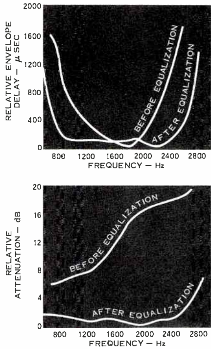
Figure 1. Both delay and amplitude distortion affect the quality of data transmission. Top panel shows the relative envelope delay of a typical voice channel both before and after equalization. The result of amplitude equalization is shown in bottom panel.
