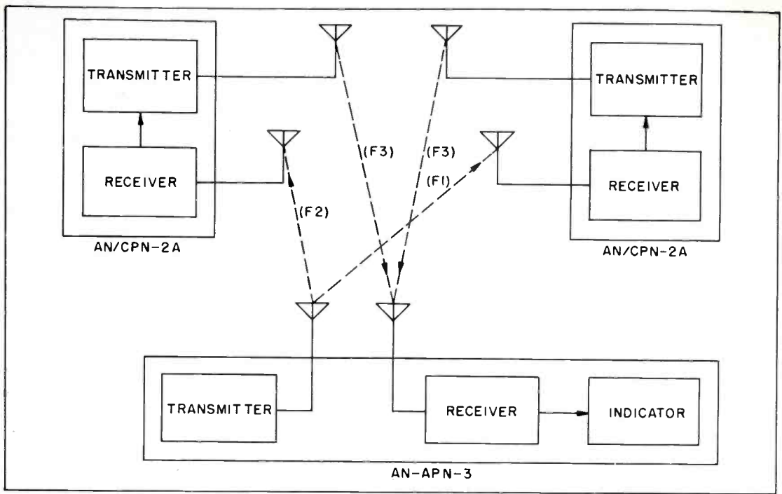
Figure 1. Basic Elements of the Shoran System
