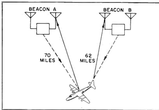
Figure 2. Example of Distance Measurements, Using Shoran Equipment
