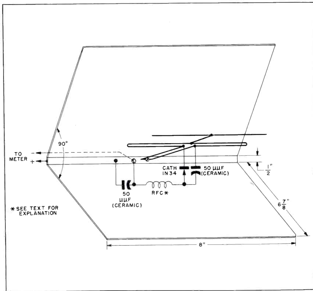
Figure 4. Detailed Construction Drawing of Field-Strength Meter Antenna
