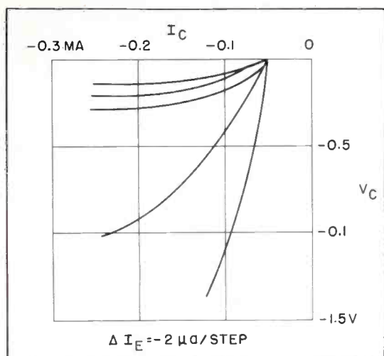
Figure 2. Collector Characteristics of Grounded-Base Point-Contact Transistor
