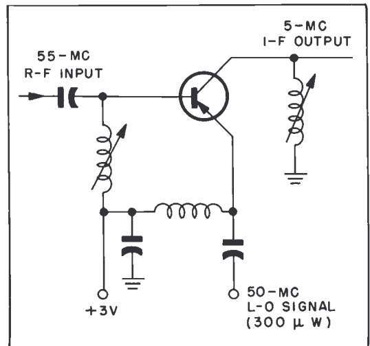
Figure 5. V-H-F Mixer Using a Surface-Barrier Transistor
