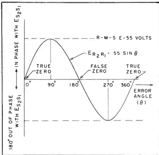
Figure 3. Graph Showing Voltage Induced into a Synchro Control Transformer Rotor as a Function of Error Angle
