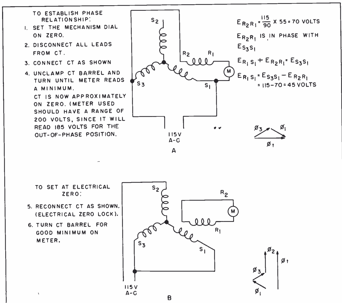
Figure 2. Jumper Method of Zeroing a Synchro Control Transformer A. Phase-Determining Connections B. Zeroing Connections
