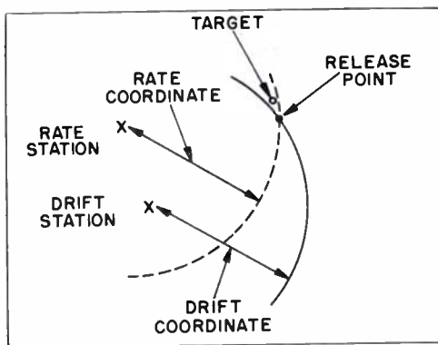
Figure 6. Method of Bombing with Shoran Equipment
