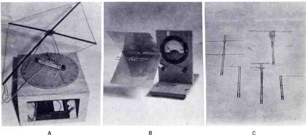
Figure 1. The Complete Antenna Demonstrator
