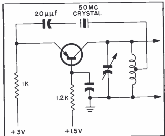
Figure 4. Crystal-Controlled Oscillator Using a Surface-Barrier Transistor
