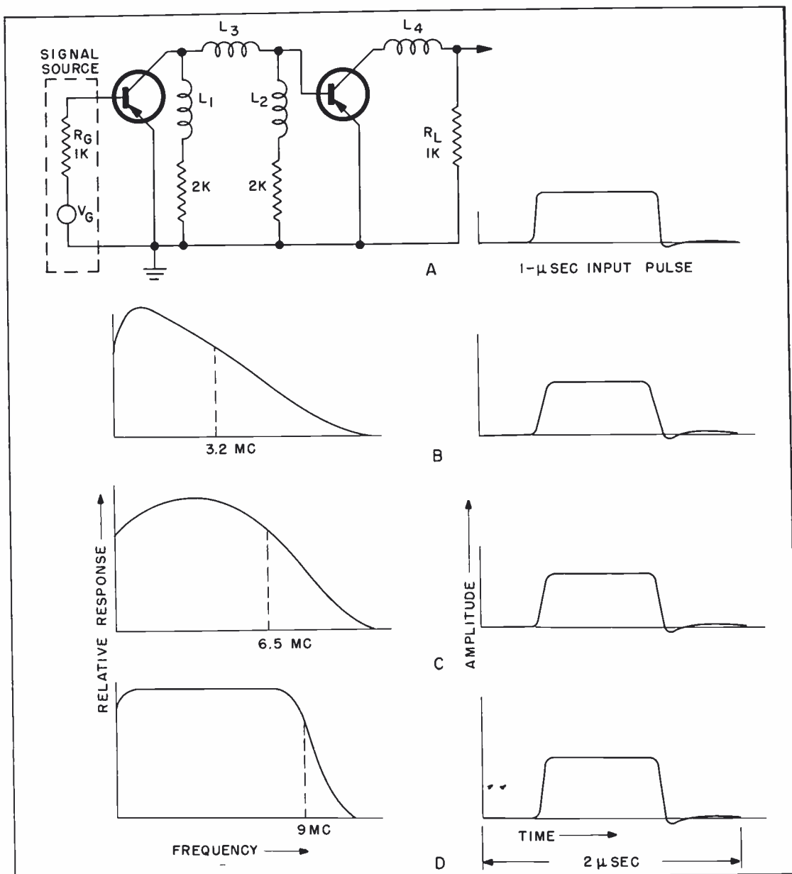
Figure 6. Two-Stage Video Amplifier Using Surface-Barrier Transistors
