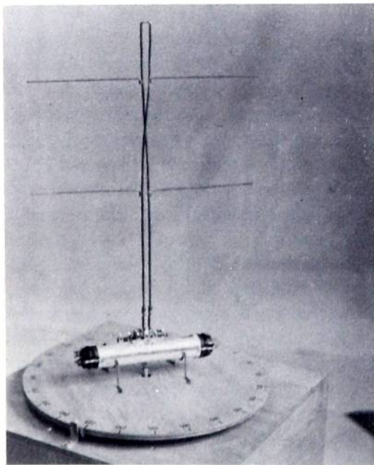
Figure 5. Antenna Demonstrator with Lazy-H Antenna in Operation
