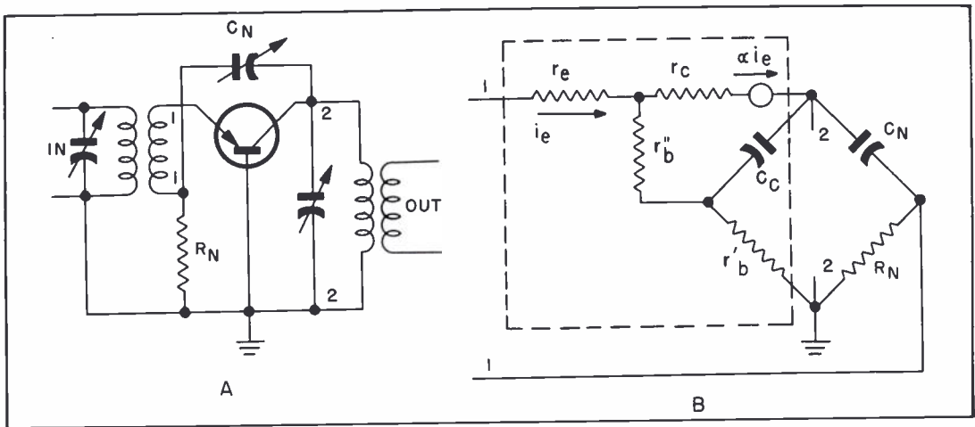
Figure 3. Neutralized Tuned Transistor Amplifier
