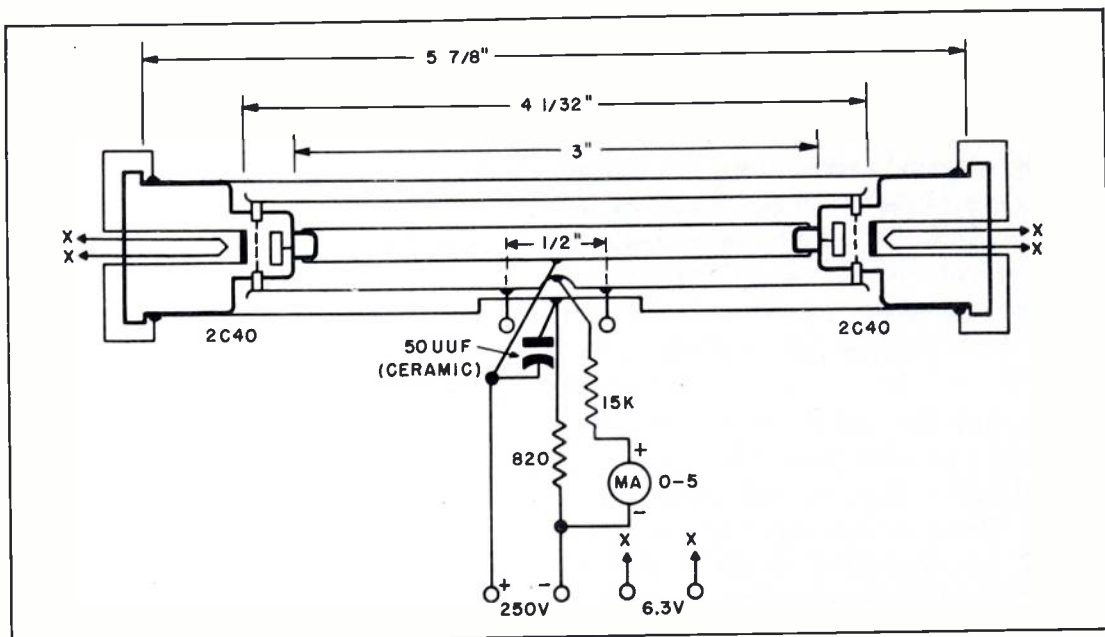
Figure 2. Diagram of Transmitter, Showing Critical Dimensions
