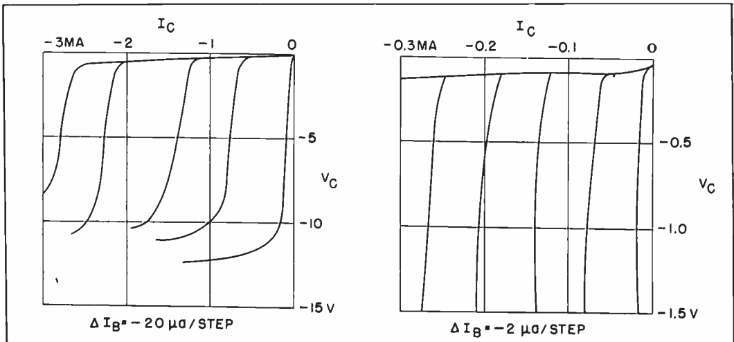
Figure 1. Collector Characteristics of Grounded-Emitter Surface-Barrier Transistor
