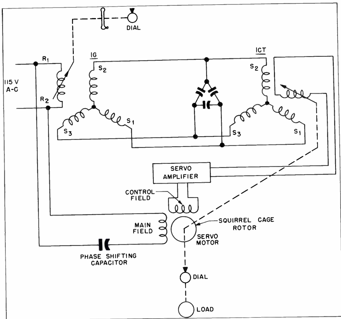
Figure 4. Typical Positioning Servomechanism, Showing the Use Synchro Capacitors on the Synchro Control Transformer
