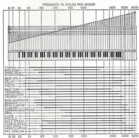
Fig. 3.—Frequency range required for the reproduction of musical instruments, voice, and noise without noticeable distortion. Reprinted from "Radio Engineering Handbook" (McGraw-Hill Book Company)
