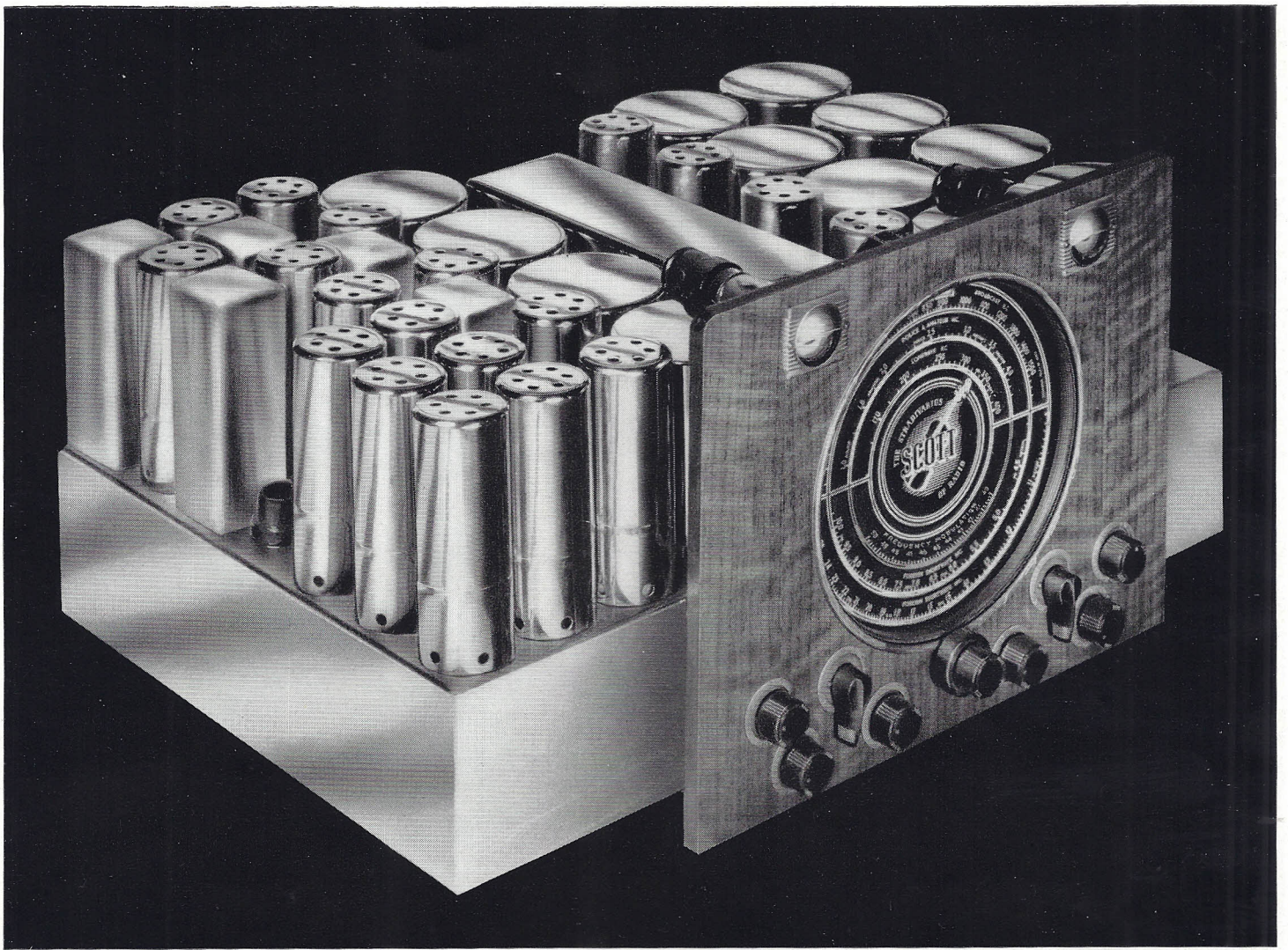
Tuning Chassis of Scott FM-AM Philharmonic
