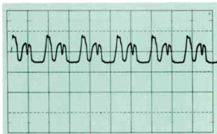
Figure 1. Typical oscillation waveform, caused by conditions described in text, displayed on a Type 547 Oscilloscope. Sweep rate 0.1 \mu s/cm. Waveform will be different on Type 545 (A), (B) Oscilloscopes but fundamental frequency will still be about 10 MHz.
