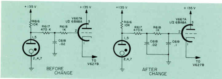
Figure 4. Before and After schematics showing installation of 0.1 discop in the +135 V supply of the Type 125.
