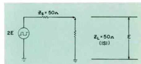
Figure 3. Simplified equivalent circuit representing the Amplitude Calibrator of a Type 544, Type 546, or Type 547 Oscilloscope and a Type 1S1 Sampling Unit.
