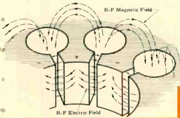
Fig. 3—Configurations of electric and magnetic fields.
