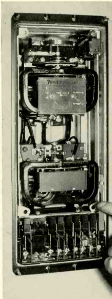
Fig. 1—A single-phase relay that includes a directional element and an induction voltage timing element is suitable for protection of a-c generators against reverse flow.
