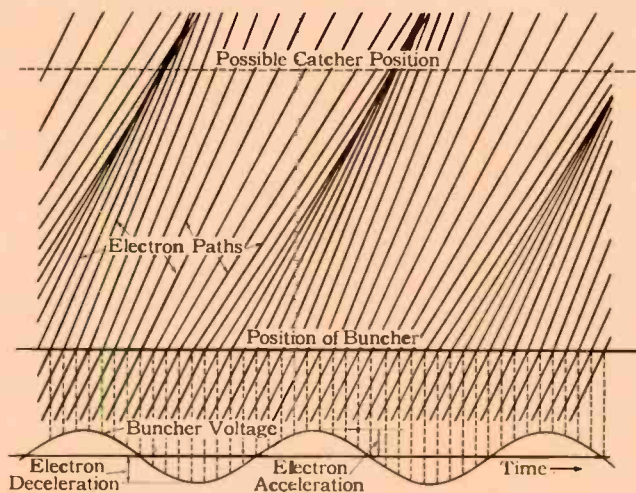
Fig. 3—The bunching process.
