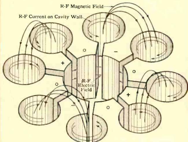
Fig. 5—One possible mode of magnetron oscillation.
