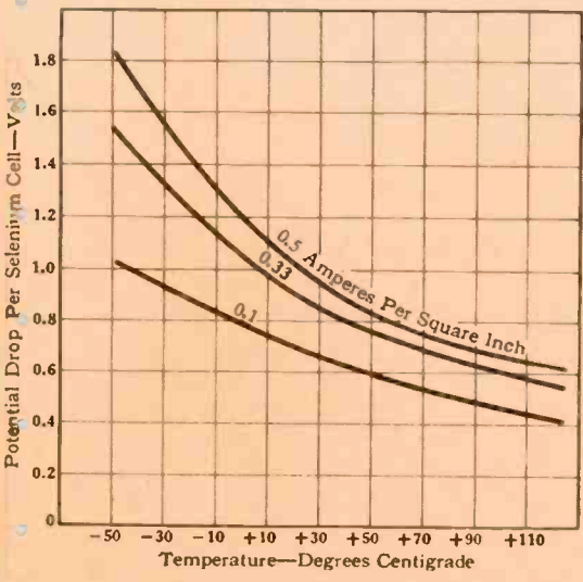
Fig. 3—These curves show the effect of temperature on voltage drop per cell. This repeats in a different form the information given in Fig. 2.
