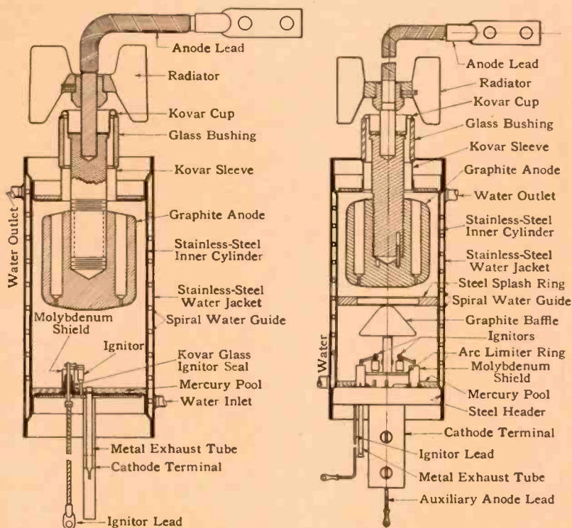
Figs. 1 and 2—The sealed ignitron for resistance-welding service (left above) is somewhat simpler than a rectifier tube (right above). The rectifier, shown in cutaway at the right, has two ignitors and has additional arc shielding.
