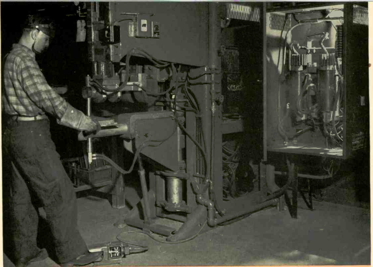
A typical resistance-welding control set-up, with the ignitron cabinet door open and tubes illuminated for purposes of the picture.
