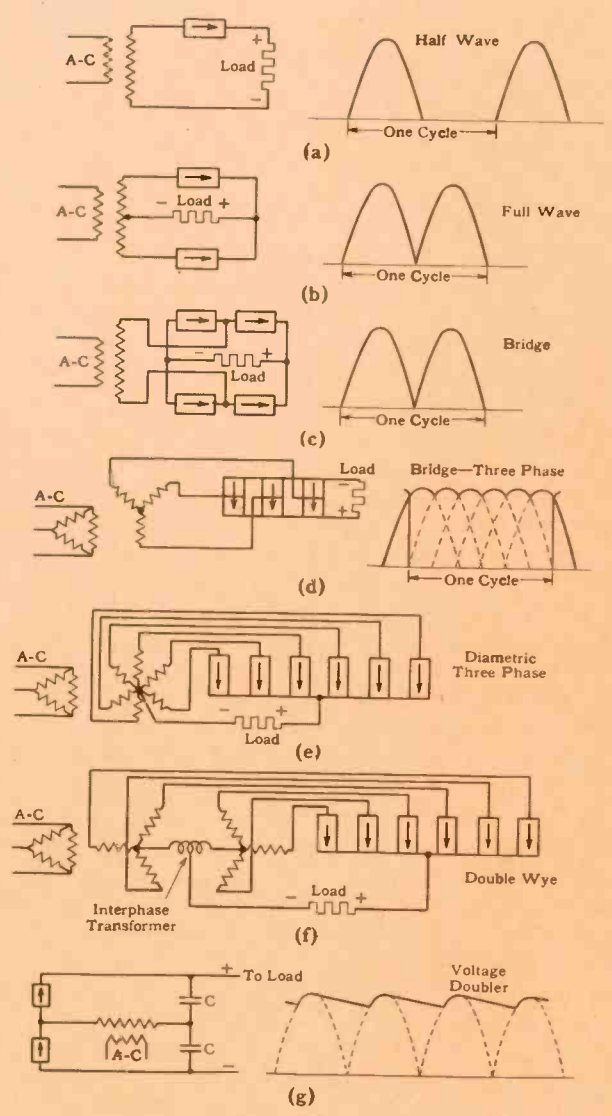
Fig. 5—The more common metal-rectifier circuits.
