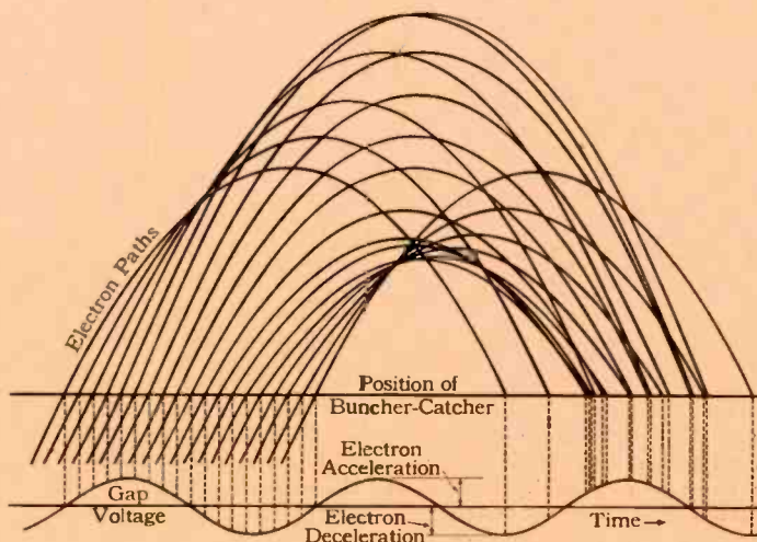
Fig. 4—An Applegate diagram for the reflex klystron.—>
