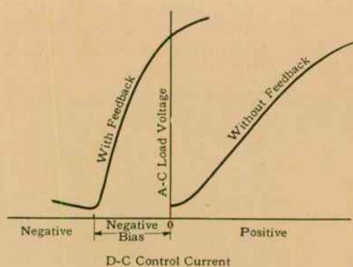
Fig. 4—Transfer curves for magnetic amplifiers with and without feedback. To obtain minimum output of a feedback amplifier with zero input, the load-voltage axis must be shifted to the left. This is accomplished by a bias through an auxiliary winding.
