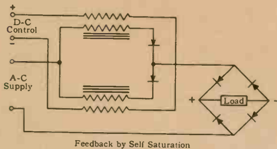
Fig. 3—Amplification of a magnetic amplifier can be increased by two schemes of feedback.
