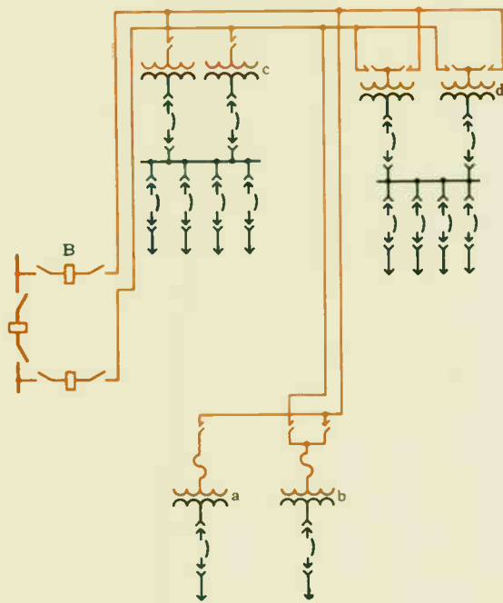
Fig. 6—Radial subtransmission circuits supplying modern distribution substations.
