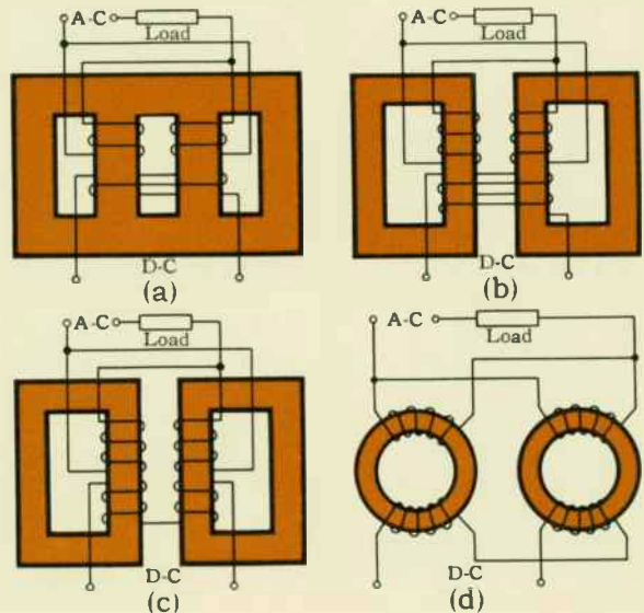
Fig. 12—Some of the many different types of core construction and circuits employed in magnetic amplifiers.
