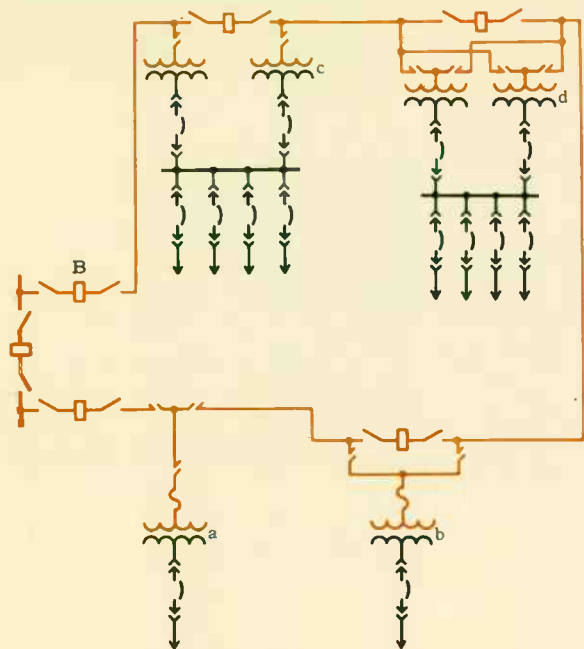
Fig. 8—Distribution substations supplied from an automatically sectionalized subtransmission loop.
