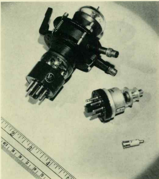
Fig. 1—Microwave communication borrows heavily from apparatus developed for radar and kindred wartime electronic systems. At left is a klystron tube for generating small amounts of power at megacycle frequencies, center is a lighthouse tube used at somewhat lower frequencies, and, right, a modern, synthetic crystal.
