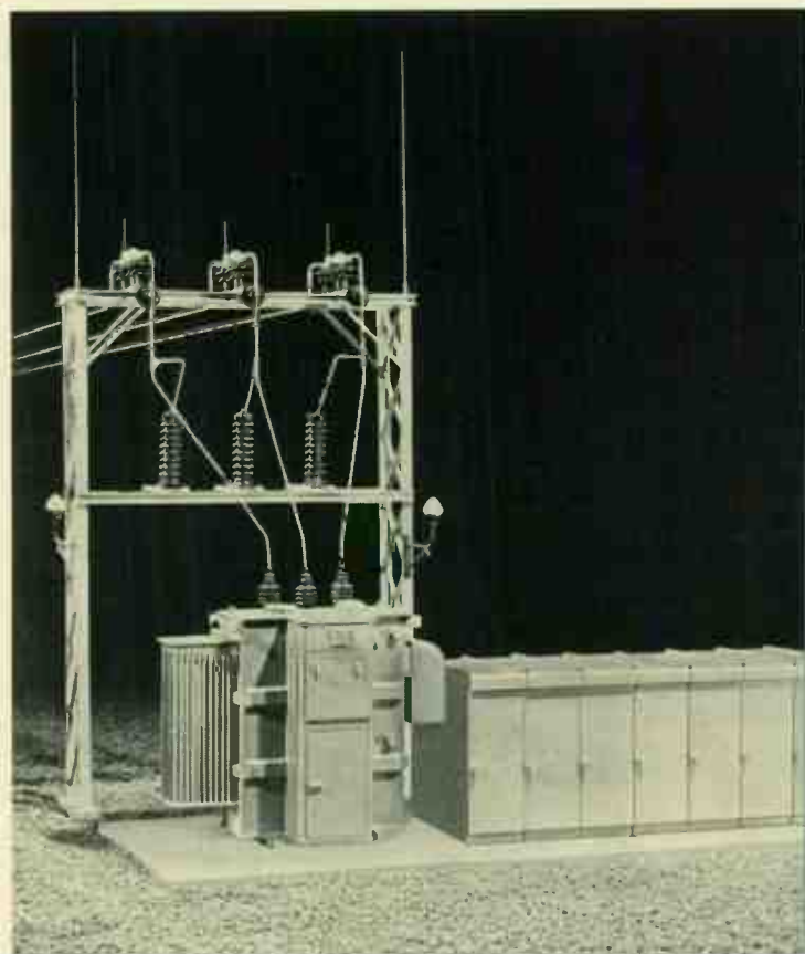
Fig. 2—The usual primary-network type of distribution substation; it can also be used in radial systems.
