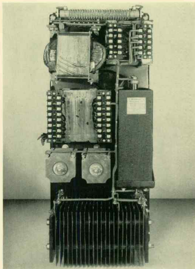
Fig. 10—The excitation panel of an ignitron rectifier uses a magnetic amplifier to control the ignition point by adjusting the bias voltage. The reactor is located above the capacitor at the right.
