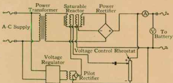
Fig. 5—The wiring diagram of the Rectomatic charger for floating service.
