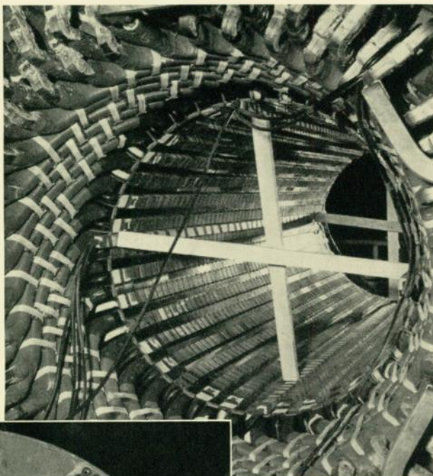
Fig. 7—Two surge-inducing coils are shown in position in the bore of a 3600 rpm generator adjacent to two machine coils for detecting short-circuited conductors.
