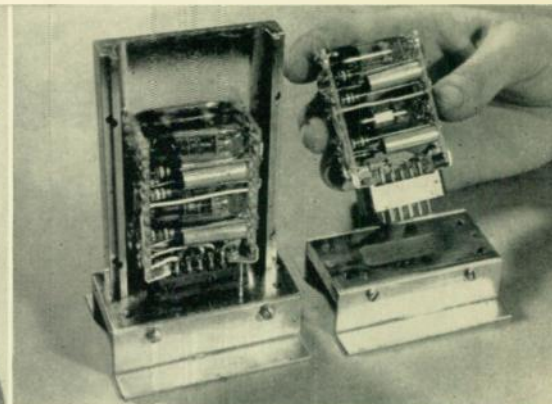
Fig. 3—Following assembly, the electronic circuit is tested for operation and is then prepared for the molding process that makes it a complete unit. The connector-base of the circuit assembly is placed in a wax plug in the baseplate of the mold. This holds the unit rigid while the liquid filler is being poured and also prevents the connector points from becoming fouled in the plastic. At left, the unit and one half of the mold is in place for pouring; the mold is held by a C-clamp.
