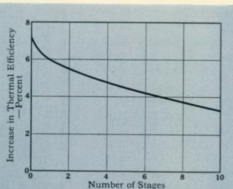
Fig. 5—The effect of several stages of feed heating on efficiency gain due to reheat at the optimum reheat pressure is shown.
