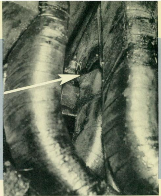
Fig. 3—The binding tape of several coils shows surface deterioration due to slot-discharge effects produced in the laboratory.
