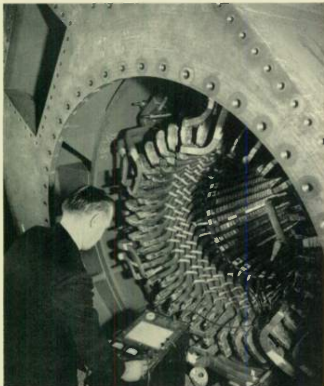
Fig. 6—High-voltage equipment for the d-c overpotential test shown attached to coils of a medium-sized 3600-rpm generator.
