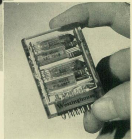
Fig. 6—In production models, instead of using the clear plastic, another inert filler is used that makes the final product opaque. The silhouette shows the relationship of the tiny components of the finished electronic circuit.
