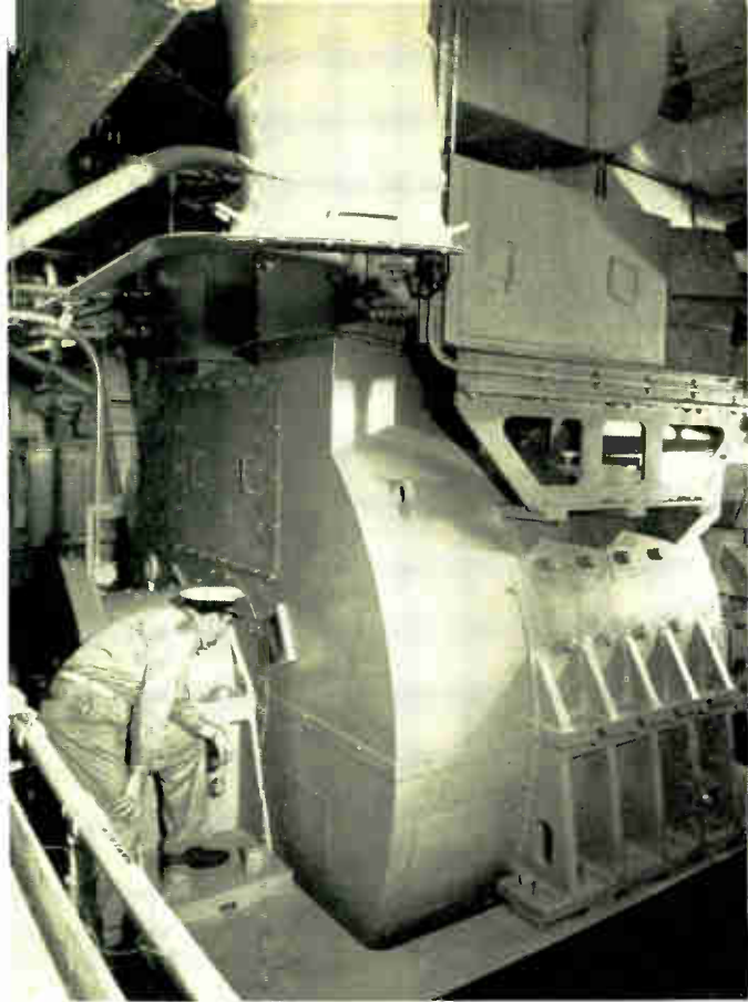
Each of the dredge's two 4000-hp propulsion motors is solidly connected electrically to its respective generator.
