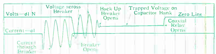
Fig. 3—An oscillogram of a simulated line-dropping test, in which a capacitor bank was the "stand-in" for the open line. A circuit similar to Fig. 2 was used, with two capacitance dividers and an amplifier.
