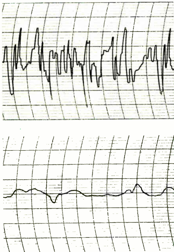
Fig. 6—Surface profiles of the washing-machine door before (above) and after (below) PR plating.
