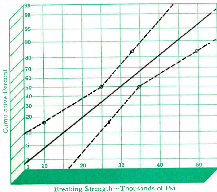
Fig. 1—Points on the 50-percent line are 4.8 units on either side of the curve; on the 16- and 84-percent lines, 8.2 units away.
