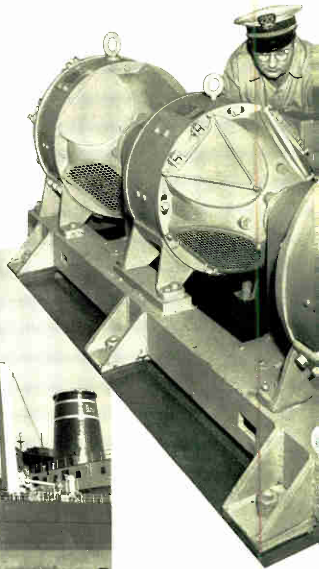
This Rotrotrol control automatically maintains constant horsepower at any speed setting and prevents motor overload.
