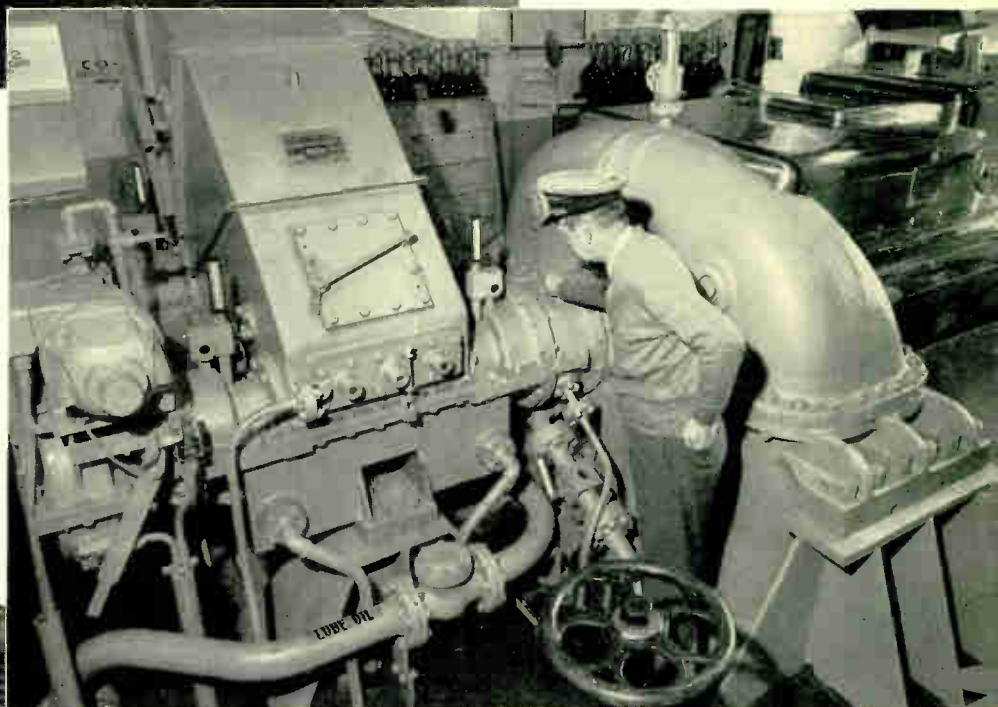
Two of these 3800-kw turbines furnish all propulsion, pumping, and auxiliary power for this seagoing dredge.
