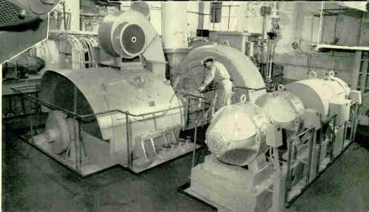
dge pump motors are d at 1850 hp each. At it, a draghoist m-g set.
