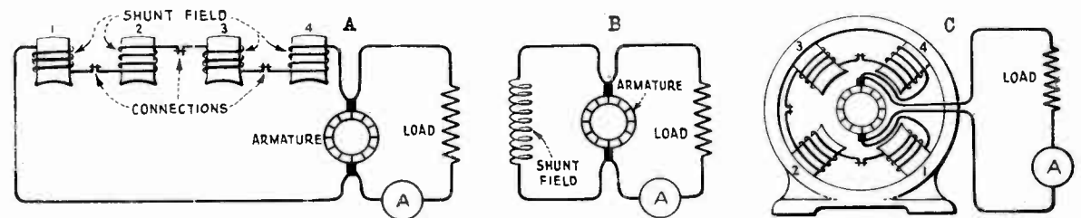
Fig.12-Diagrams illustrating shunt wound field coil connections
