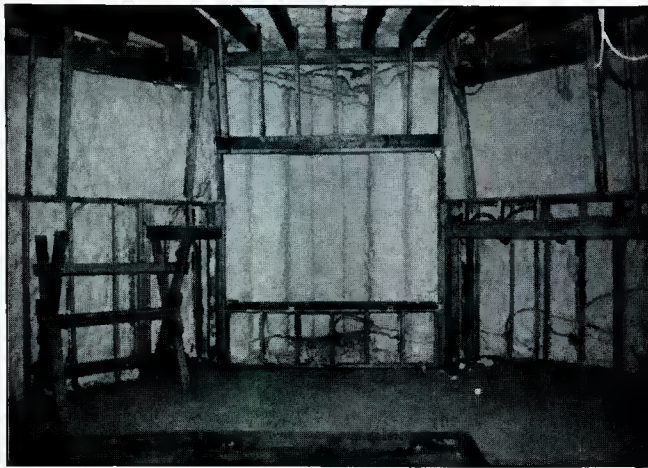
Figure 8B. Wall framing for broad-bandwidth RPG diffusors in front of LFD covered with absorbent material.
