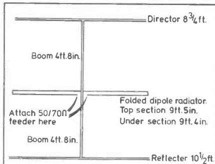
FIG. 3b. Yagi antenna for 50MHz
