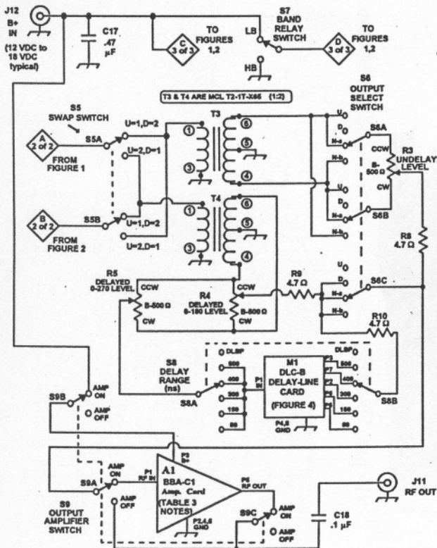
DCP-2 DUAL CONTROLLER / PHASER FIGURE 3: OUTPUT SECTION
