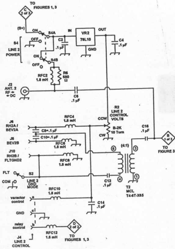
FIGURE 4: DLC-B DELAY-LINE CARD
