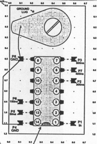
DCP-2 DUAL CONTROLLER / PHASER FIGURE 6: LEFT SIDE, RIGHT SIDE PICTORIALS
