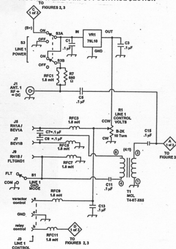
FIGURE 1: LINE 1 INPUT / CONTROL SECTION
