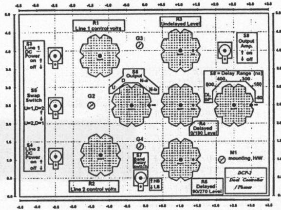
FIGURE 5: TOP SIDE PICTORIAL
