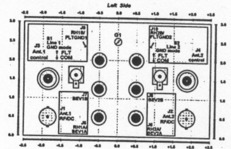
DCP-2 DUAL CONTROLLER / PHASER FIGURE 6: LEFT SIDE, RIGHT SIDE PICTORIALS
