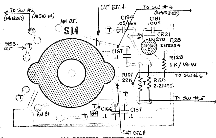
AM DETECTOR CIRCUIT BOARD Figure 36
