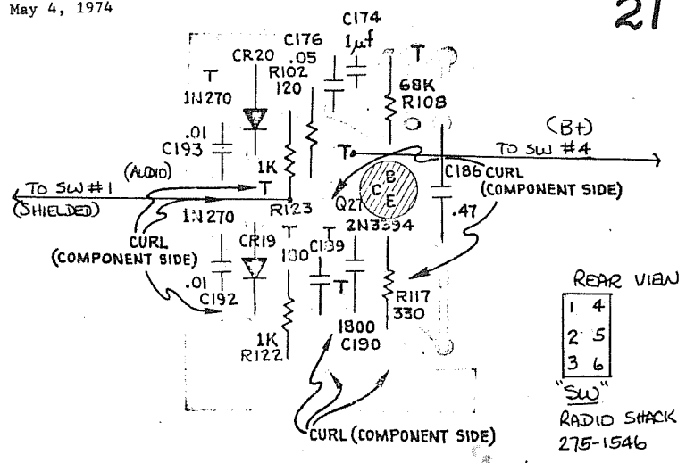
BFO CIRCUIT BOARD Figure 35
