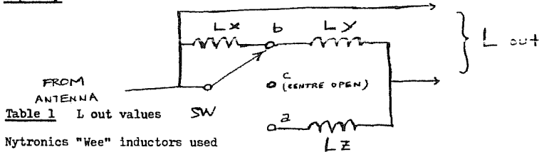
Figure 3: three-value inductance unit
