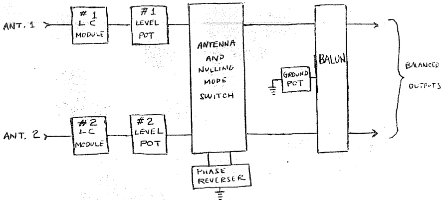
Figure 2 block diagram of conventional phasing unit
