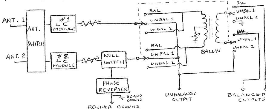
Figure 9 versatile approach to unbalanced output
