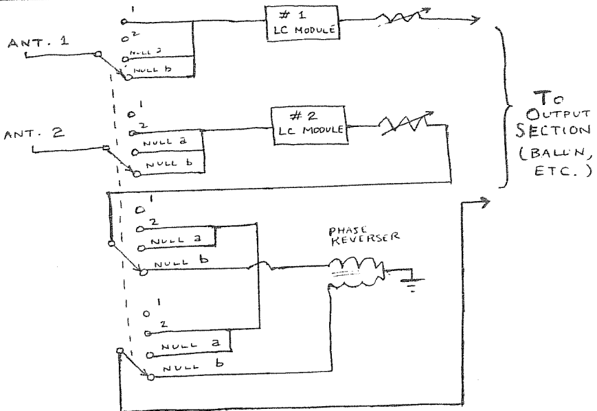
Figure 6 single antenna/null mode switch configured to reduce crosstalk
