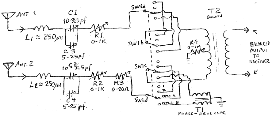
Figure 1 a conventional phasing unit
