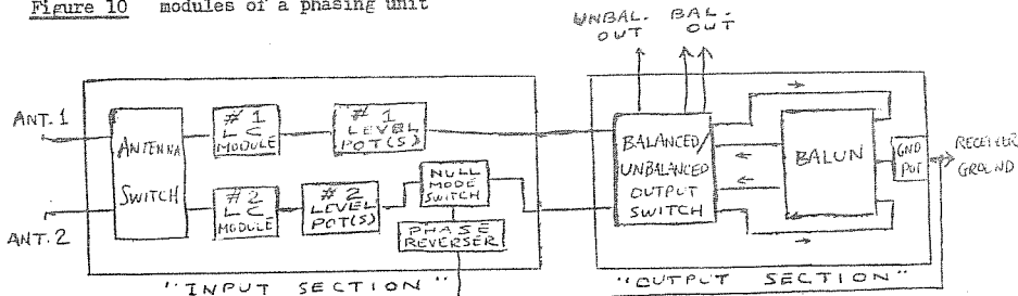
Figure 10 modules of a phasing unit
