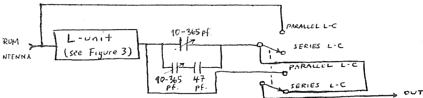
Figure 4 schematic of LC module (2 per phasing unit)
