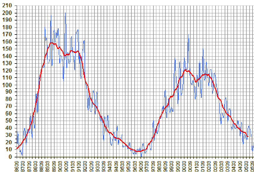
Solar Cycles 22-23
