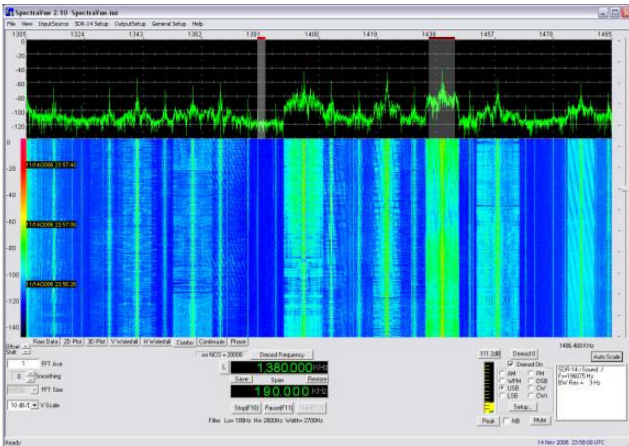
Above: The SDR-14 provides various display options – here we have a basic spectrum graph above and a waterfall display below. Two separate frequencies are being received independently, one in AM and the other in USB.
