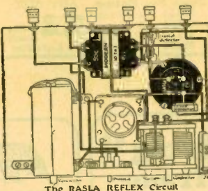
The RASLA REFLEX Circuit
