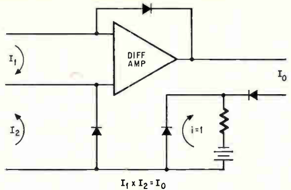
Commonality. With a differential amplifier in the adder, the input and offset diodes have the same terminal.
