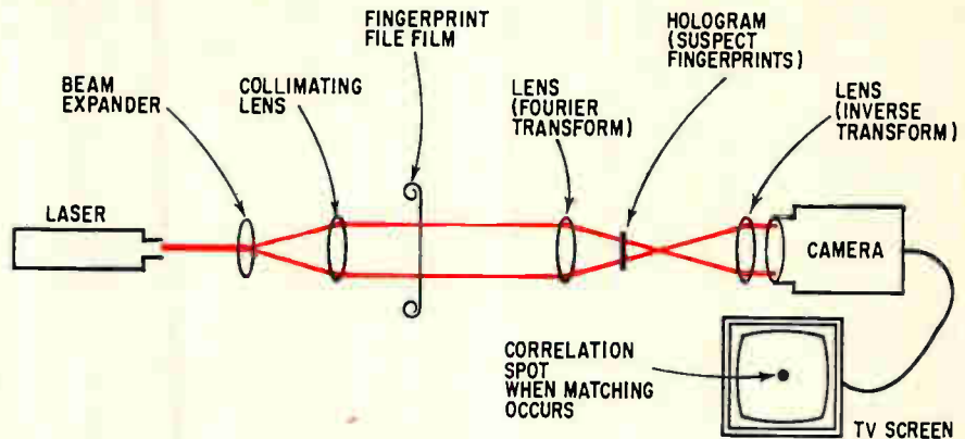
Fingerprint matching. Optical correlator bench in Conducon's Confess system. When file print matches sample, reference beam is seen as spot on crt.
