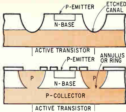
Encircled. Ring-shaped barrier, bottom, is compared to mesa transistor.
