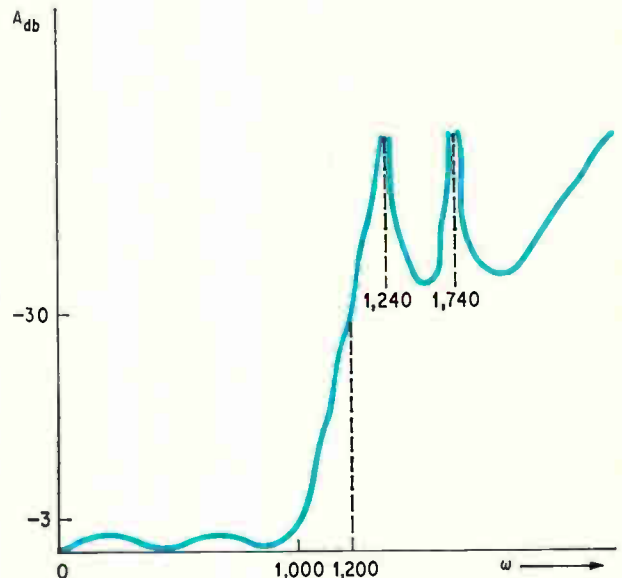
Cauer filter. The fifth order arrangement at top produces the low-pass response specified. At lower left is the filter's pole-zero location, and at lower right is its over-all response curve.
