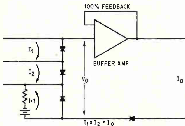
Adder. A complete adding circuit employs an operational amplifier and an antilog diode.
