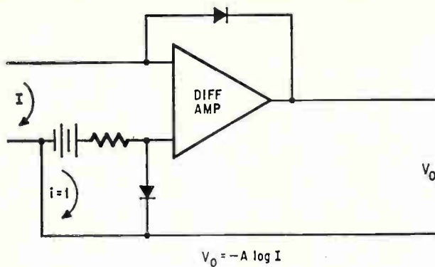
No offset. By adding another diode to the differential amplifier circuit, the constant C is eliminated.
