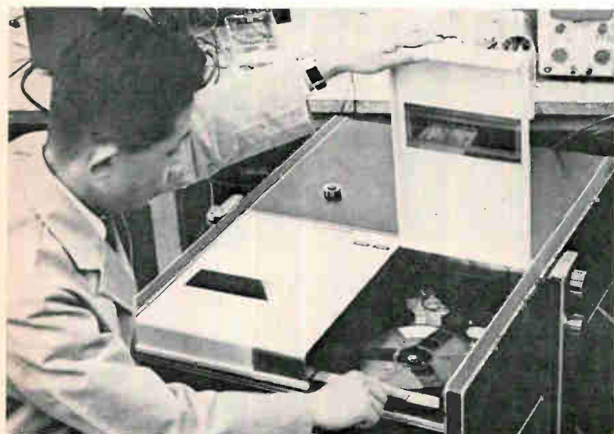
Fast whirl. Matsushita video tape copying equipment can duplicate a 2,400-foot reel of master tape in just two minutes. Bifilar winding of master and slave tapes on the same reel is what makes machine a speedster.
