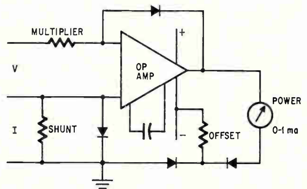
Instrumental. Besides doing arithmetic, the log diodes can be used in such things as a wattmeter.
