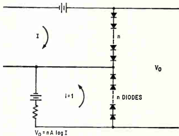
Chain reaction. With n diodes connected in series, the exponent of the output is increased by n .
