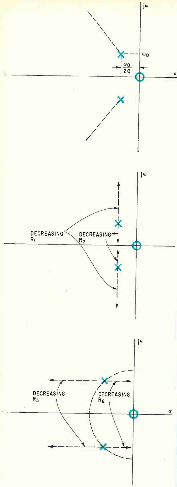
Three routes. Graph at top shows path of the poles of D(s) as a function of decreasing R_7 and R_8 for a band-pass output. At center is the path as a function of R_1 and R_2 , and at bottom is the path as a function of R_5 and R_6 .
