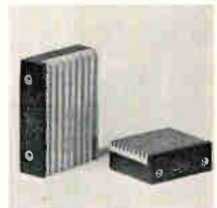
High voltage, medium power rectifier modules J531 and J532 dissipate 10 w and 20 w respectively in free air. Size of the 10-w module is 1 7/8 x 2 x 3/4 in.; the 20-w module, 2 1/8 x 3 x 3/4 in. Major uses are in general industry, particularly in heavy equipment and transmitting equipment, and in many r-f generating systems. Solitron Devices Inc., 256 Oak Tree Road, Tappan, N.Y. [443]
