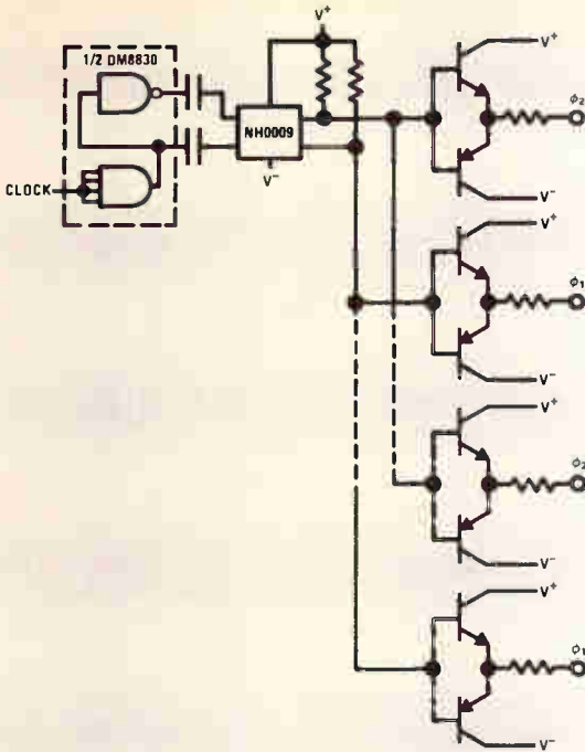
FIGURE 3. Remote Buffers Redistribute Clock Signals
