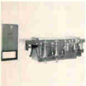
Conveyorized circuit board stripper model CBS automatically removes silk screen and photo sensitive resists after etching. Special powered nylon brushes convey p c boards through the machine at any speed from 2 to 14 ft a minute. At the same time, both sides of the boards are flooded with solvents. Baron-Blakeslee Inc., 1620 S. Laramie Ave., Chicago 60650. [421]
