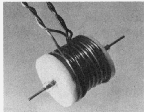
The basic relay is as tiny as many commercial sub-miniature units, a whole lot cheaper, can be designed with greater versatility, and is a lot of fun to build. The basic relay, shown here, is nothing more than a coil of wire wound around a magnetic relay switch.
