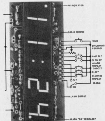
Additional optional functions diagrammed at left in schematic are shown above connected to the module.
