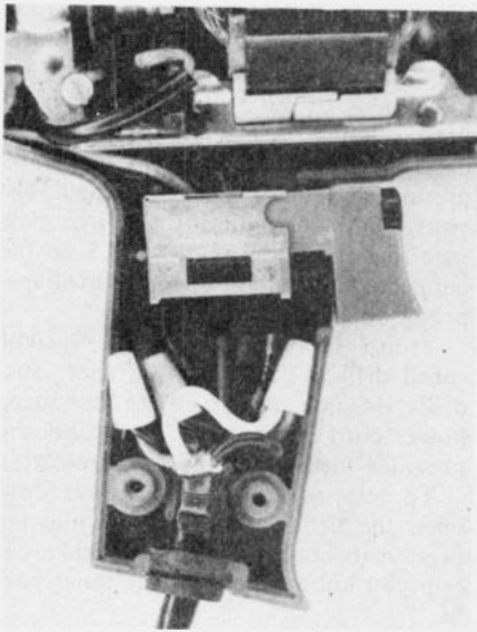
Trigger of a variable speed power drill contains a silicon-controlled rectifier (SCR) to convert incoming AC current to DC current, and a slide resistor to vary the voltage and thus vary speed of the drill motor. If malfunction is traced to this component, replace with a new trigger unit.
