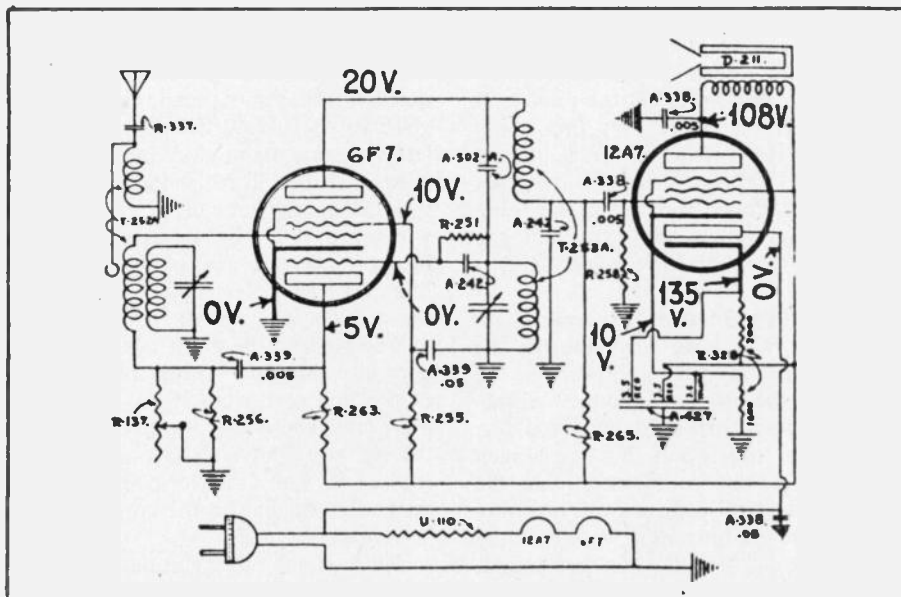
The Kadette, Jr. was one of the first AC-DC receivers made. The tube filaments are in series.
