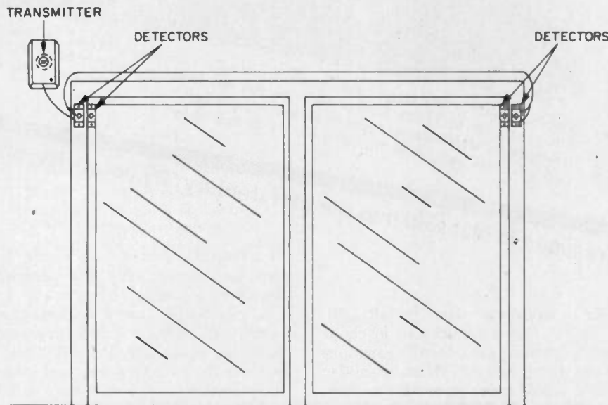
Sliding glass doors can be protected by installing detectors on both end doors. Use double stick adhesive—not screws—on metal frames and glass.
