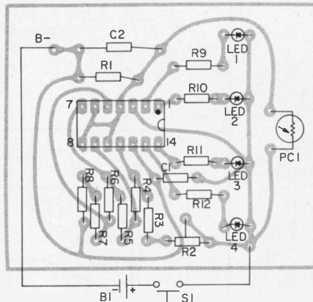
Placement of parts on Lone Ranger's printed circuit board. If you use perf board instead you can put the parts wherever you want, but you'll find this general arrangement most convenient.
