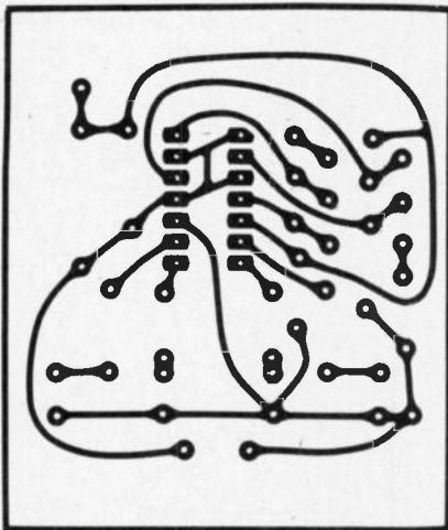
This is a full-size template for the printed circuit board, if you want to make yours just like the author's. See the text for suggestions on making printed circuit boards if this is your first.
