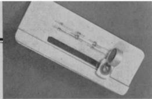
The ceramic magnet of this sliding switch passes over five 1 1/8" size reed switches to provide double-pole, single-pole sequencing. Separate diagram shows a simple mechanism which permits locking the magnet "on" or any "off" position.
