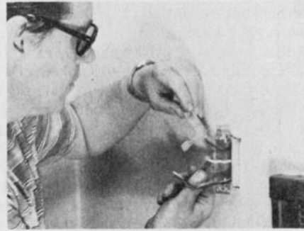
Fig. 6. Before cutting the outer wall and mounting the fan unit, install all the necessary electrical wiring. While you can use a simple on-off switch, a multi-speed selector switch or variable speed control can be a great help when you want to move air slowly, in small quantities.
