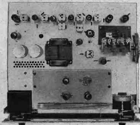
Top view of T250 with MA250 adapter-installed.
