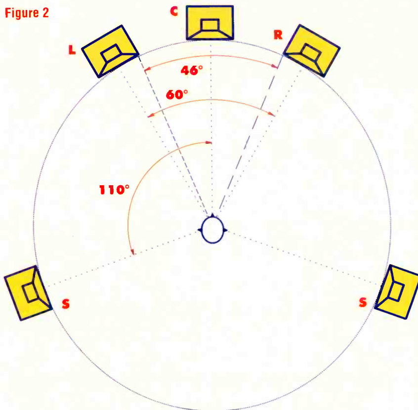
This speaker layout, with a 60-degree left/right spread, has been recommended for use in surround-sound tests for high-definition TV (HDTV).
