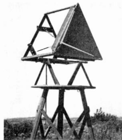
Fig. 7—One of the largest corner reflectors used during the tests with a 2-foot free edge. The sides can be deviated manually or by means of a motor-driven device and readings taken of the response in the receiver.
