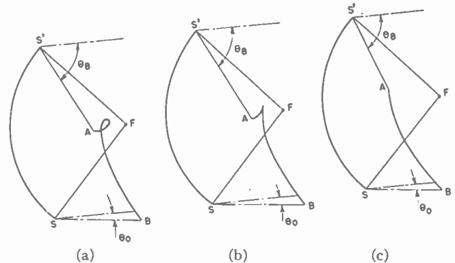
Fig. 8—Typical examples of curves for testing single-valuedness of the surface.
