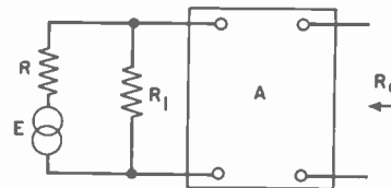
Fig. 3—Shunted signal generator feeding an amplifier.
