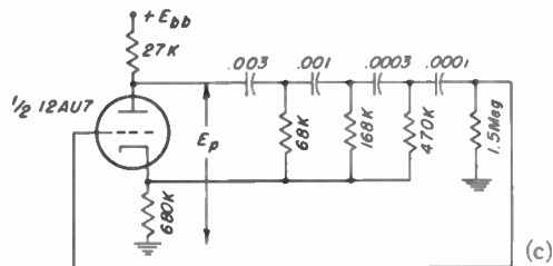
Fig. 1—Phase-shift oscillator.
