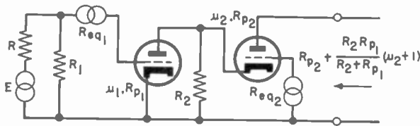
Fig. 12—Shunted generator feeding a Wallman low-noise amplifier.
