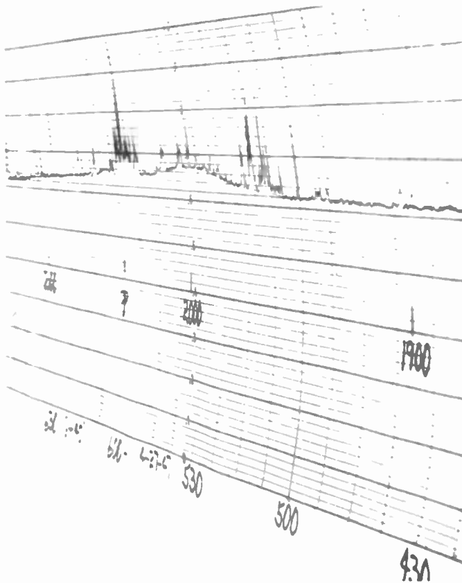
Fig. 5—Sample trace showing cosmic static at declination +40^\circ in Cygnus.
