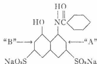
Benzoyl H Acid (Disodium Salt) or (1-Benzoylamino-8-hydroxy-naphthalene-3,6-disulfonic acid)
