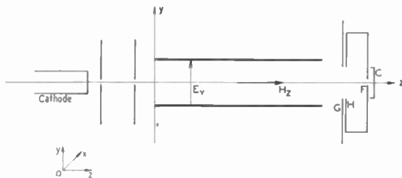
Fig. 1—Arrangement of electron gun, region on high-frequency field, and the electron collector system.
