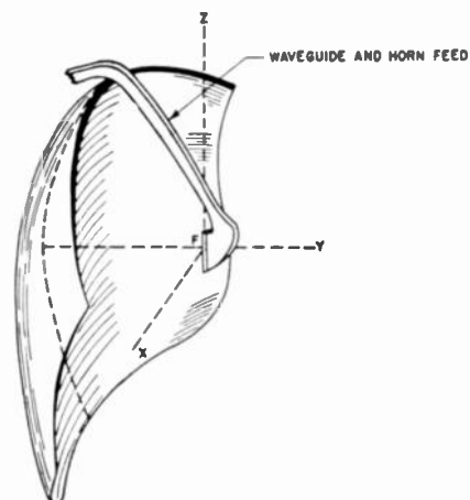
Fig. 6—A sketch of the shaped-reflector antenna.
