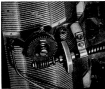
Close-up of flexible shaft connection to a variable resistor through simple worm gearing. With arrangements like this you can get smooth, accurate fingertip control.
