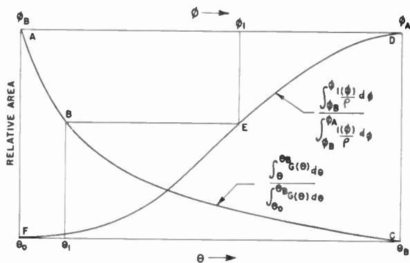
Fig. 4—Graph for the determination of \theta = F(\phi) .
