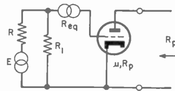
Fig. 8—Shunted generator feeding a conventional (cathode-separation) amplifier.
