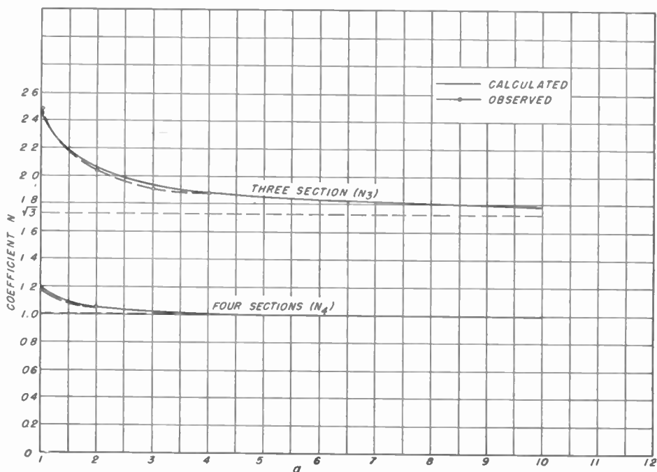
Fig. 3—Coefficient N versus a .
