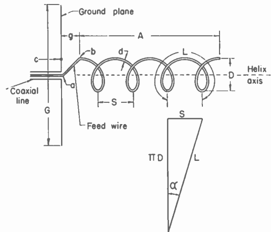
Fig. 1—Helix and associated dimensions.
