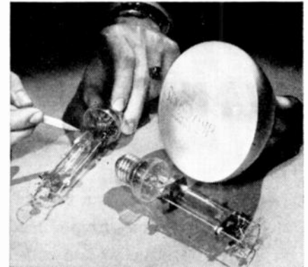
Westinghouse Sun Lamp uses "Z" Nickel springs to support quartz tube inside the lamp. Temperatures up to 750°.
