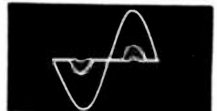
Triple exposure made with Type 271-A while varying constants of peak-clipping circuit.
