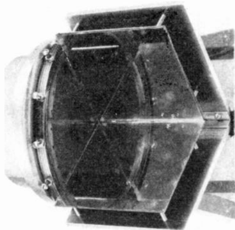
Fig. 10—One of the voice-powered reflectors used during the measurements. Two sides of the corner reflector are glass mirrors, while the third side is a metal diaphragm, excited by the human voice (size of each mirror, 4 \times 4 inches).
