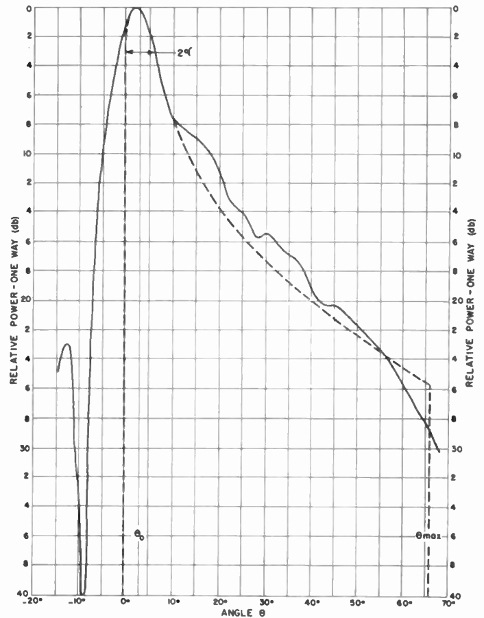
Fig. 10—The pattern of the antenna, computed for
