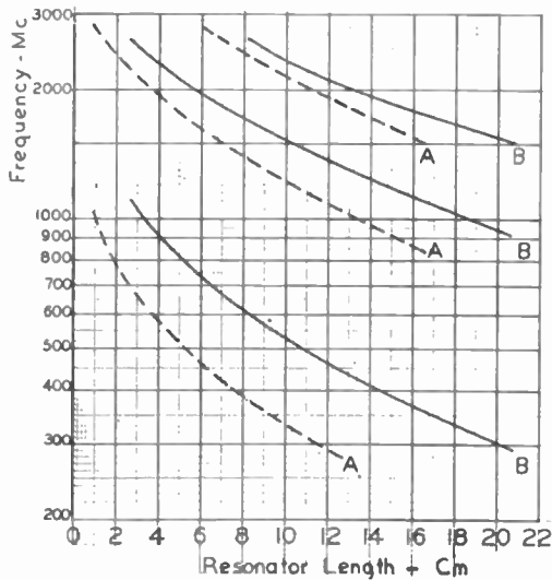
Fig. 5—Experimental tuning curves. For resonator A, C = 6.5 \times 10^{-12} farad, Z_0 = 57 ohms, and CZ_0 = 3.7 \times 10^{-10} ohm-farad; for resonator B, C = 2.0 \times 10^{-12} farad, Z_0 = 32 ohms, and CZ_0 = 6.4 \times 10^{-11} ohm-farad.
