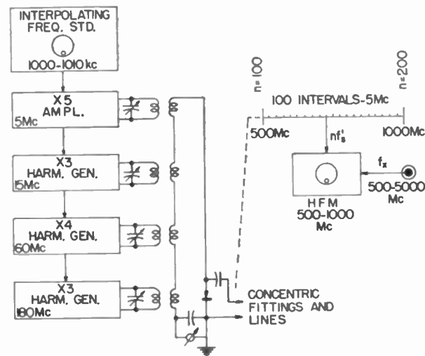
Fig. 5—A method of extending the range of measurement of a particular interpolating frequency standard.
