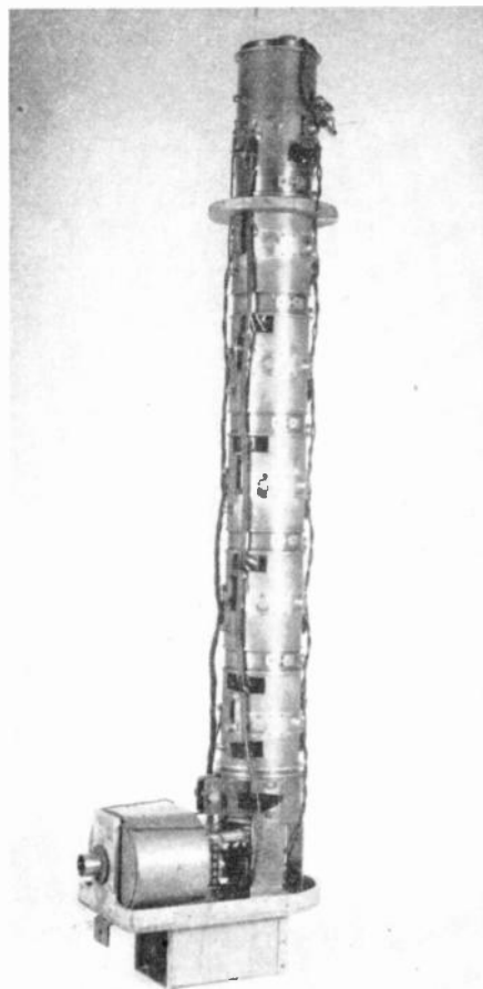
Fig. 2—A seven-stage rf amplifier at 480 Mc, using lighthouse tubes.
