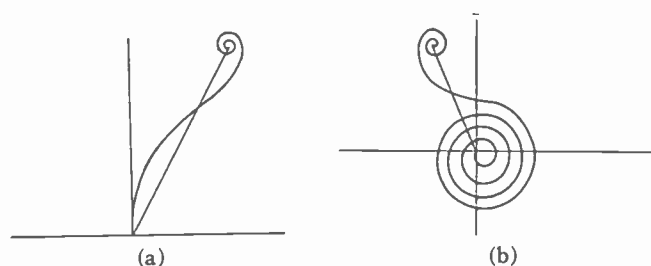
Fig. 14—Spirals resulting from vector addition of amplitude contributions from elements of the reflector surface. (a) Spiral for \theta nearly equal to \theta_0 . (b) Spiral for large \theta .
