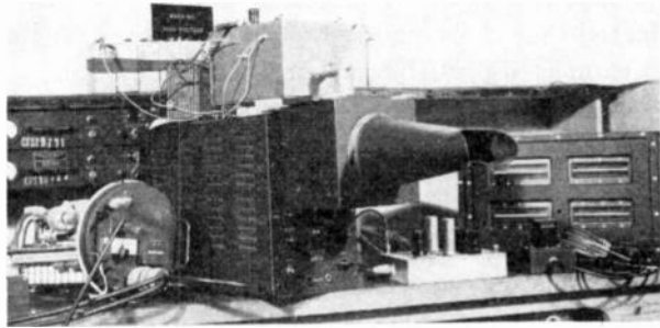
Fig. 6—A photograph of the measuring setup in Fig. 5, showing to the right a Frahm frequency meter used for identification of reflectors modulated with a complex wave. (The NIT system of identification.)
