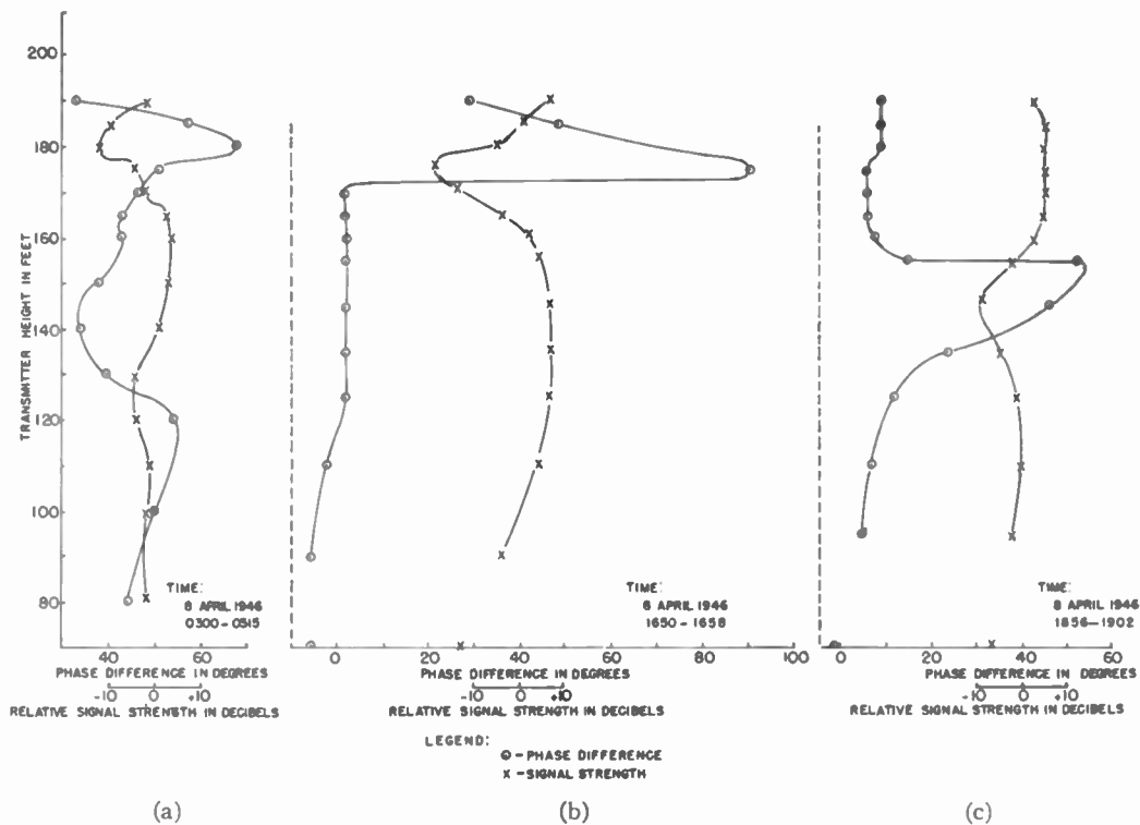
Fig. 2—Phase difference and signal strength versus height.
