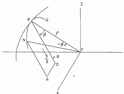
Fig. 1—Conditions for transverse sections of the reflector.
