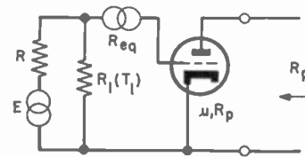
Fig. 13—Schematic for calculating the effect of transit-time loading on noise figure.
