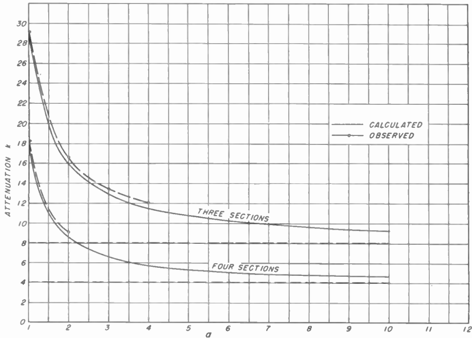
Fig. 2—Attenuation versus a .
