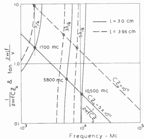
Fig. 2—Curves of 1/2\pi f CZ_0 and \tan 2\pi lf/v (ordinate) versus frequency (abscissa). Solid curves are for l = 3.0 cm and CZ_0 = 5 \times 10^{-11} ohm-farad; dashed curves are for l = 3.96 cm and CZ_0 = 10^{-11} ohm-farad.
