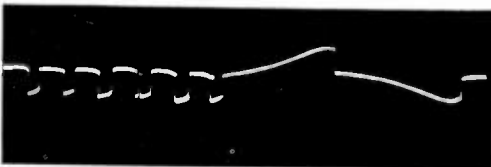
Output voltage of Type OB2 Voltage-Regulator Tube, with sudden applications of resistive load, using Type 314 Continuous-Motion/Single-Frame Camera.
