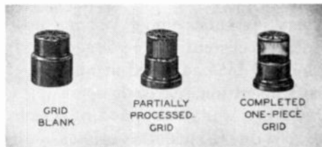
Fig. 8—Fabrication of one-piece grid.
