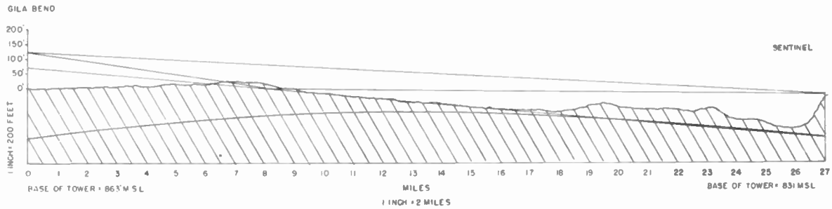
Fig. 5—Path profile for \gamma = 3.3 .
