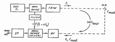
Fig. 13—A simple communications circuit showing the possibility of superheterodyne reception without the need of a local oscillator, the microwave local oscillator being replaced by an rf oscillator and associated mixers and filters.
