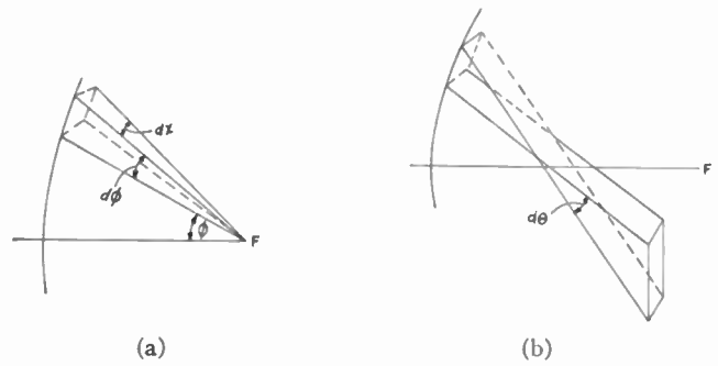
Fig. 3—On the energy relations in primary and secondary patterns.
