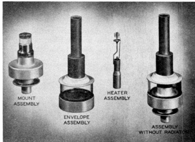
Fig. 4—Three main components and final assembly.
