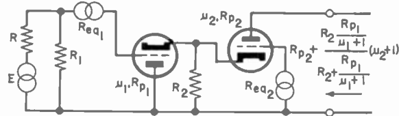
Fig. 11—Shunted generator feeding a cathode-coupled amplifier
