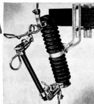
The flat "K" Monel spring on the top casting of this fuse cutout holds the fuse under constant pressure against the upper coating. A coil spring, also "K" Monel, trips the fuse tube when the fuse blows. According to James R. Kearney Corporation "K" Monel springs "are well adapted to applications in heavy industrial areas subjected to a salt and sulphurous atmosphere."
