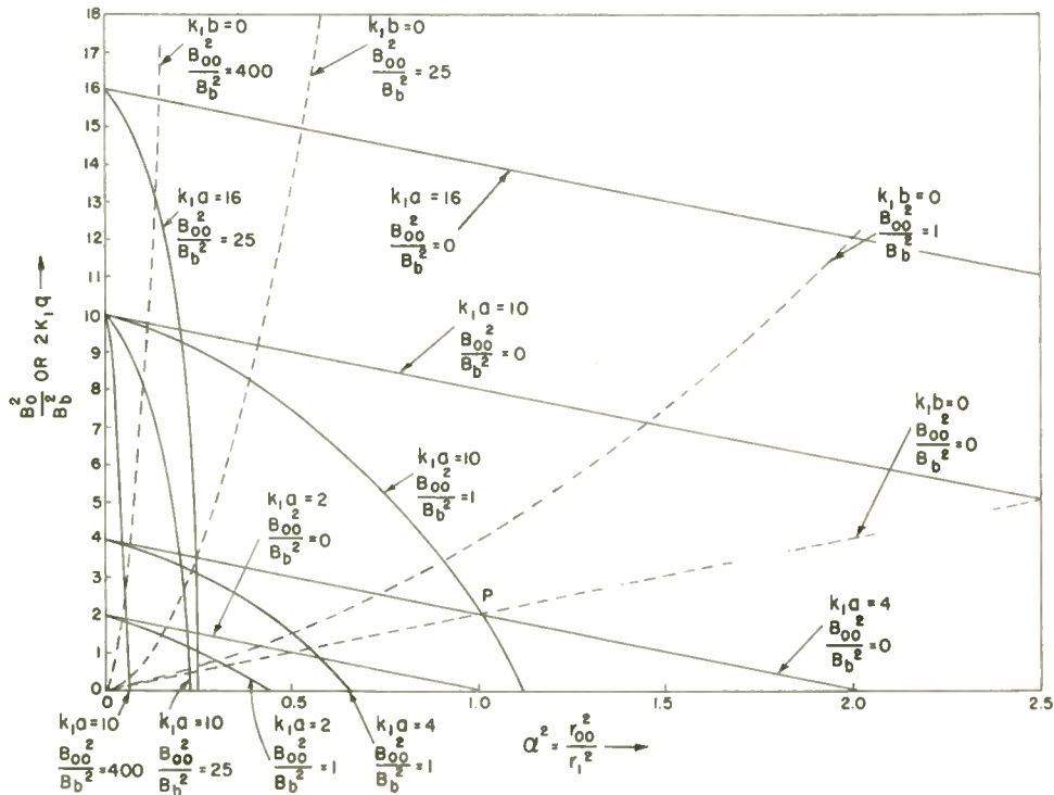
Fig. 7—The dashed curves give the values of (B_0/B_b)^2 vs \alpha^2 , for various ratios (B_{00}/B_b)^2 , when K_1 b = (B_0^2/B_b^2) - 2\alpha^2 - 2\alpha^4(B_{00}/B_b)^2 = 0 . The solid curves give the values of (B_0/B_b)^2 vs \alpha^2 for various ratios (B_{00}/B_b)^2 and various values of K_1 a = (B_0^2/B_b^2) + 2\alpha^2 + 6\alpha^4(B_{00}^2/B_b^2) .
