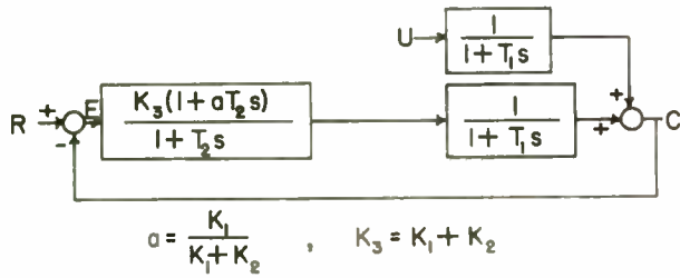
Fig. 3—Velocity servo with lag compensation (simplified diagram).
