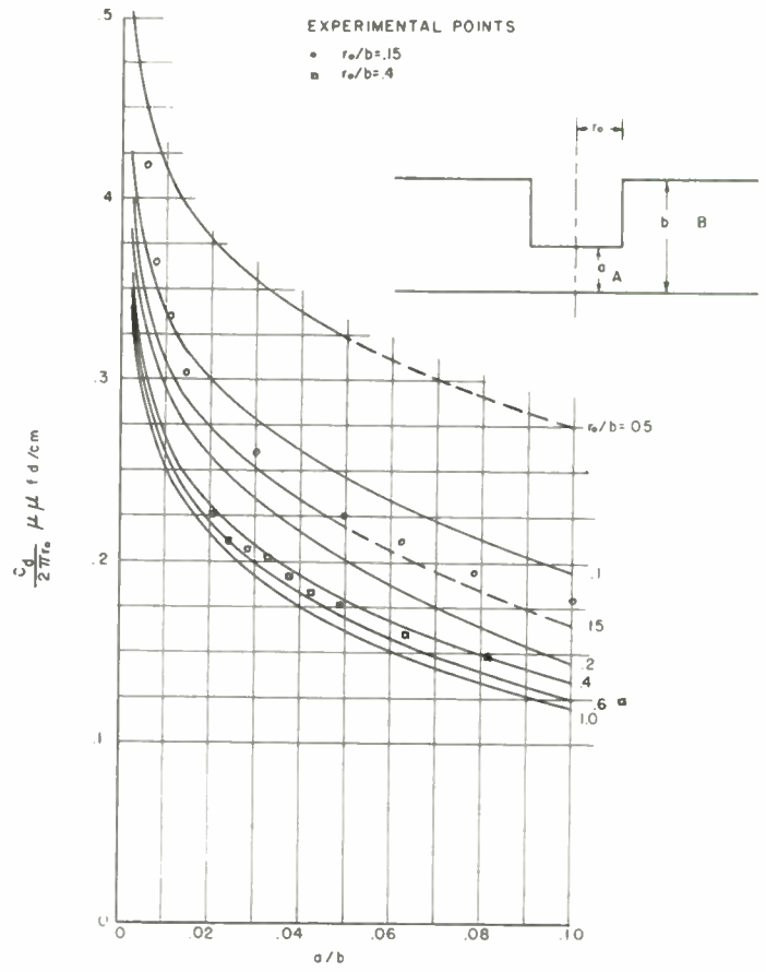
Fig. 1 (a) and (b)—Discontinuity capacitance for step in radial line, wider spacing outside.
