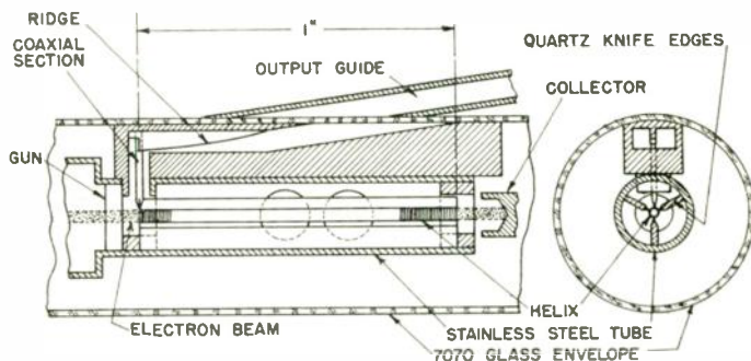
Fig. 1—Constructional details of the millimeter-wave tube. For minimum transmission loss the output waveguide is offset with respect to the internal waveguide as shown.
