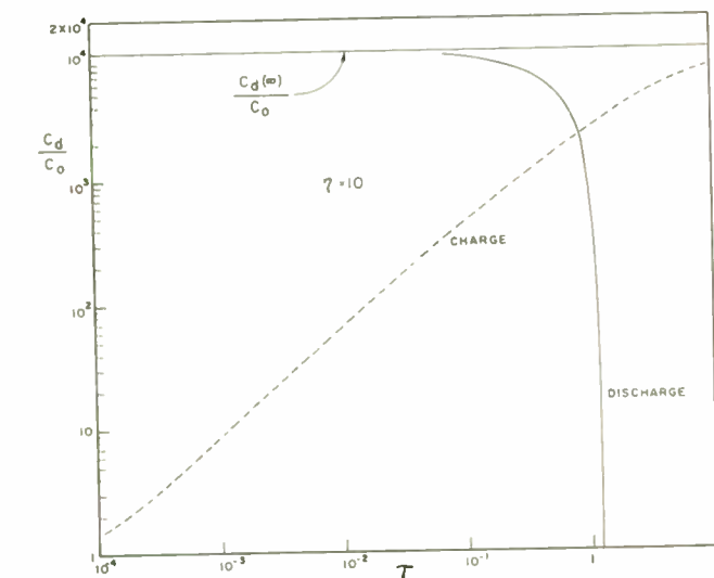
Fig. 10—Log-log plots of the time dependence of the differential capacitance of the space-charge capacitor for \eta=10 during charging and discharging.
