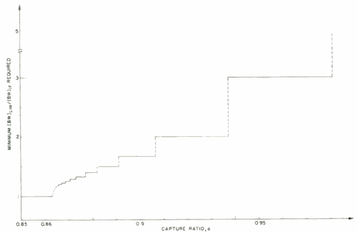
Fig. 7—Plot of the calculated minimum values of the ideal limiter filter bandwidth necessary for preserving the average instantaneous frequency of the resultant signal at that of the stronger signal.
