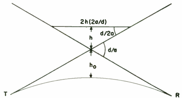
Fig. 2—Geometry of scattering volume.
