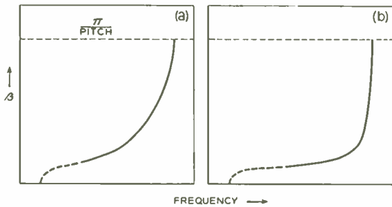
Fig. 3—Propagation characteristic of circuit of Fig. 1. (a) Widely-spaced slots. (b) Close-spaced slots. Propagation constant,
