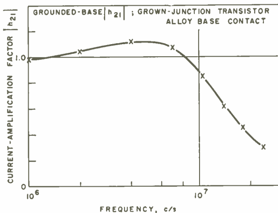
Fig. 2—Magnitude of grounded-base current-amplification factor |h_{21}| as a function of frequency for grown-junction transistor with alloy base contact.
