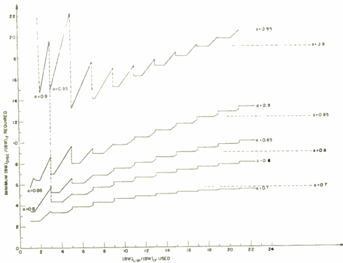
Fig. 10—Plots of the calculated values of minimum requirement in discriminator bandwidth as a function of the ideal limiter filter bandwidth used.
