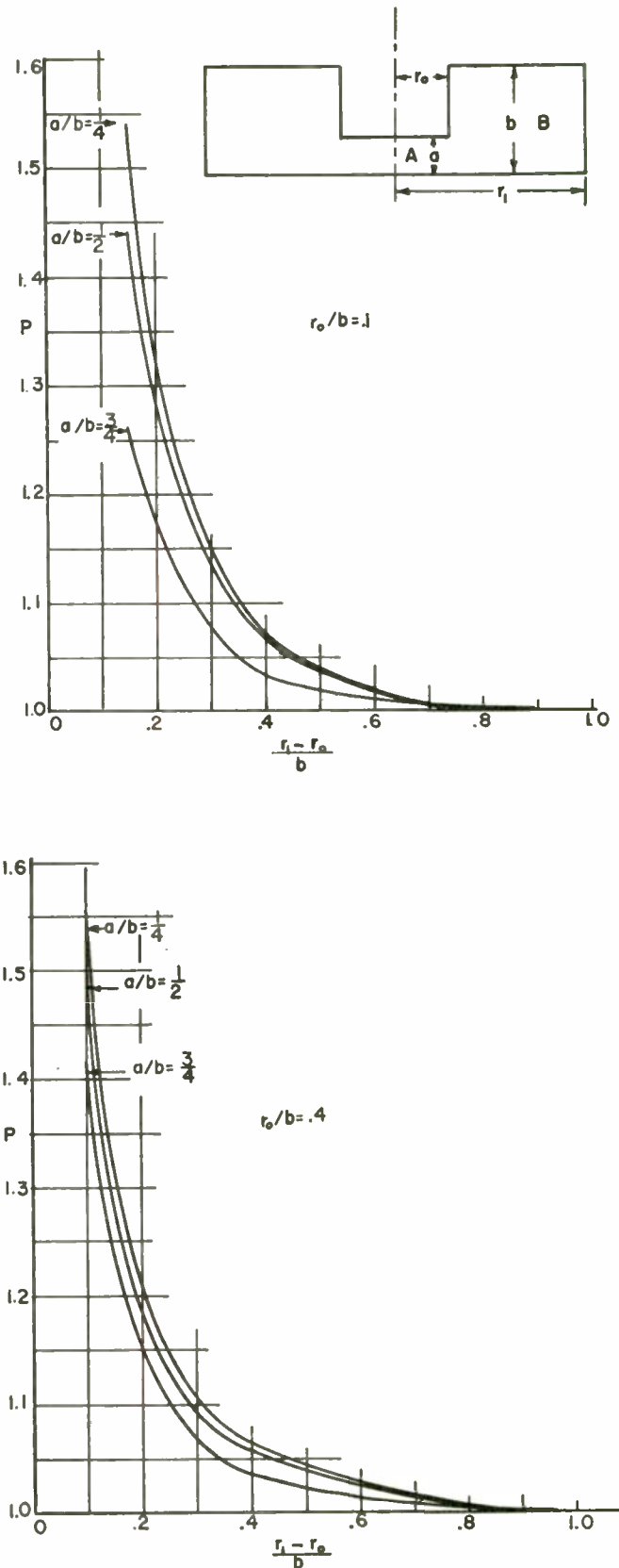
Fig. 6—Proximity factor for a shorting cylinder near the step.
