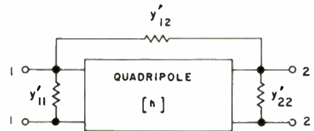
Fig. 4—Quadripole with external admittances between terminals.
