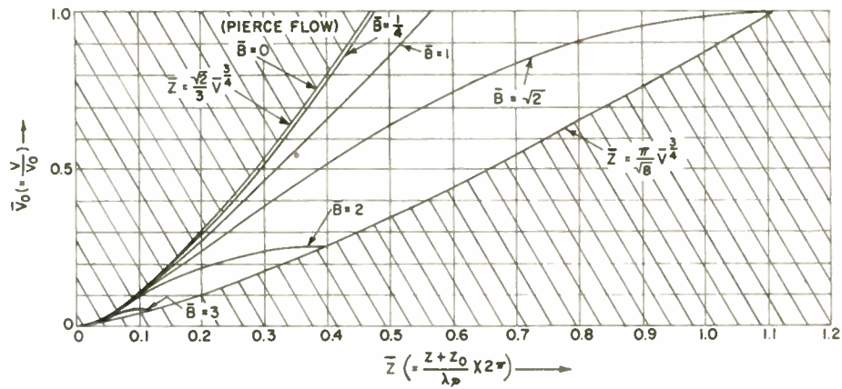
Fig. 4—Potential distribution required for parallel electron beam flow for different values of effective uniform magnetic field B_{z0} . Where \bar{B} = B_{z0}/B_0 , \bar{V} = V/V_0 , \bar{z} = 2\pi(z+z_0)/\lambda_p . The Pierce gun is a special case when \bar{B} = 0 .
