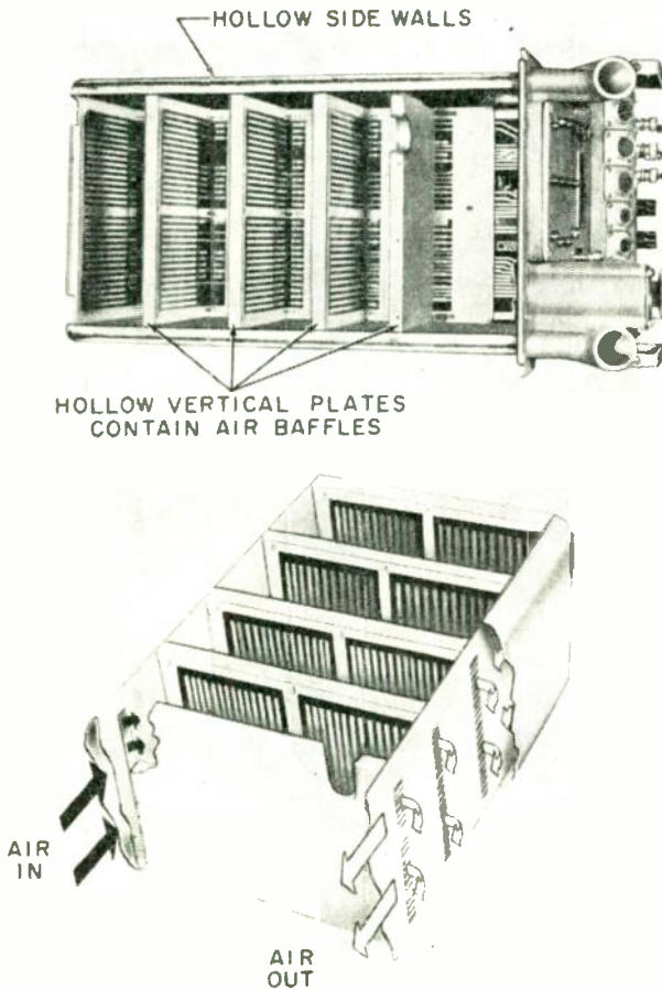
Fig. 3—Cooling chassis.
