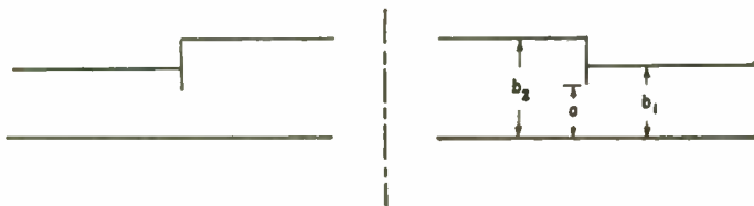
Fig. 7—Diaphragm discontinuity.
