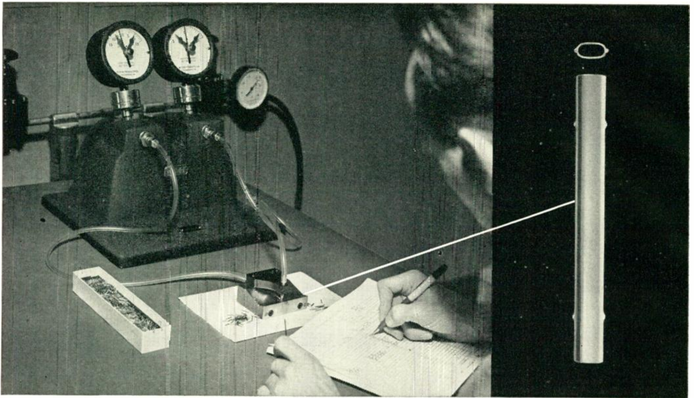
On this specially designed pneumatic comparator gage, the operator can check dimensions of elliptical cathodes to an accuracy of .0001" major axis and .00005" minor axis on mass production runs.
