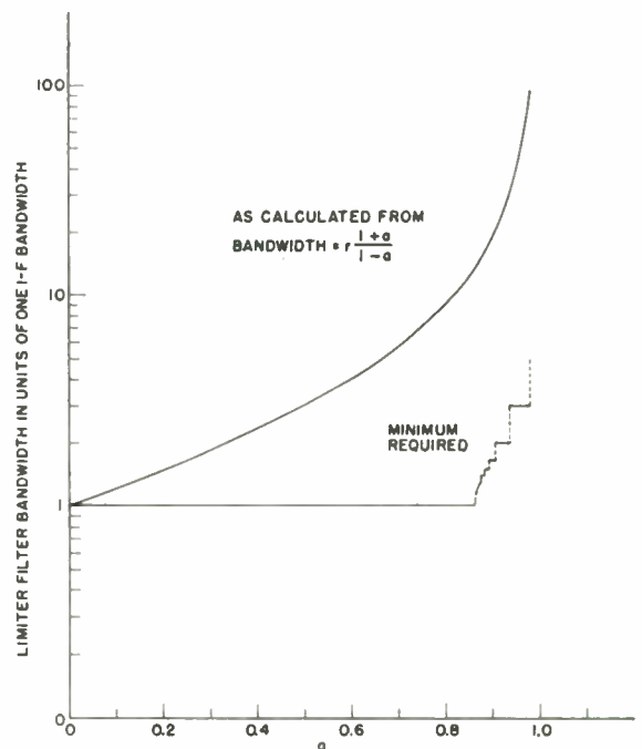
Fig. 8—Plot of the "sufficient" requirements in limiter bandwidth specified by previous investigators superimposed upon plot of the calculated minimum "necessary" requirements.
