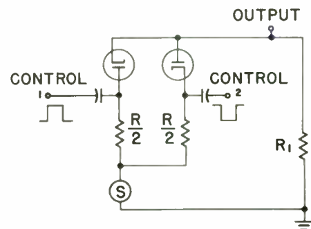
Fig. 2—Ac-coupled two-diode-bridge gate.
