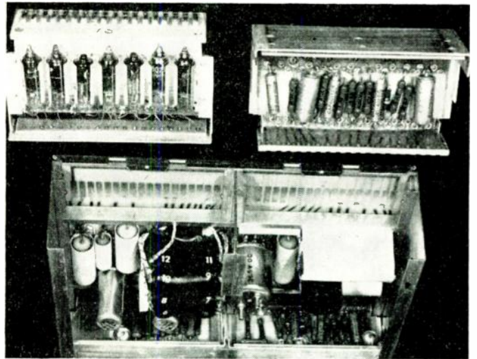
Fig. 8—Computer.
