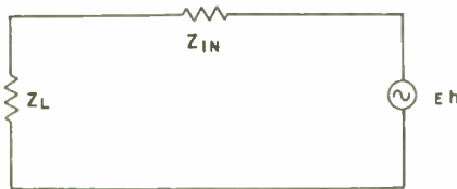
Fig. 6—Equivalent circuit for a receiving antenna.
