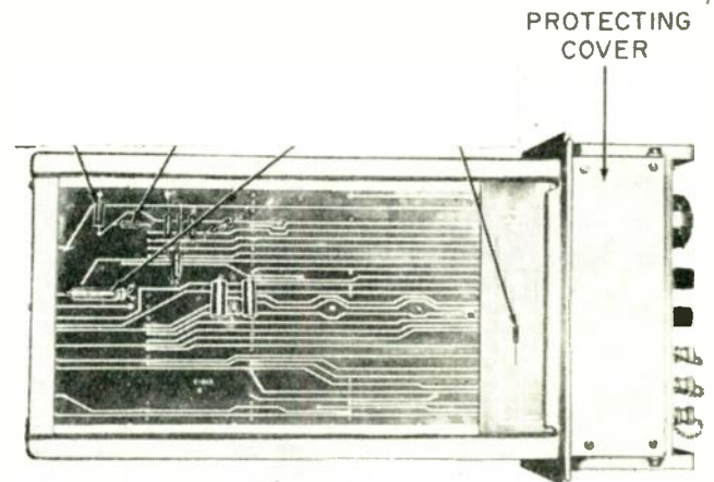
Fig. 4—Interconnecting plate on bottom of cooling chassis.
