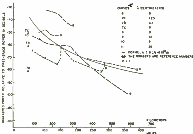
Fig. 5—Scattered power vs distance, centimeter waves.
