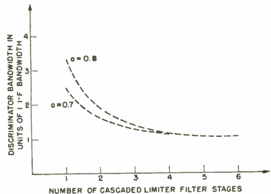
Fig. 11—Variation of the minimum discriminator bandwidth required with the number of cascaded stages of limiter-ideal filter combinations. The ideal limiter filter bandwidth used is just one IF bandwidth.
