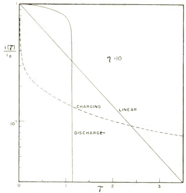
Fig. 5—Semi-log plot of normalized charging and discharge currents versus normalized time for the exponential capacitor with \eta=10 and for a linear capacitor.
