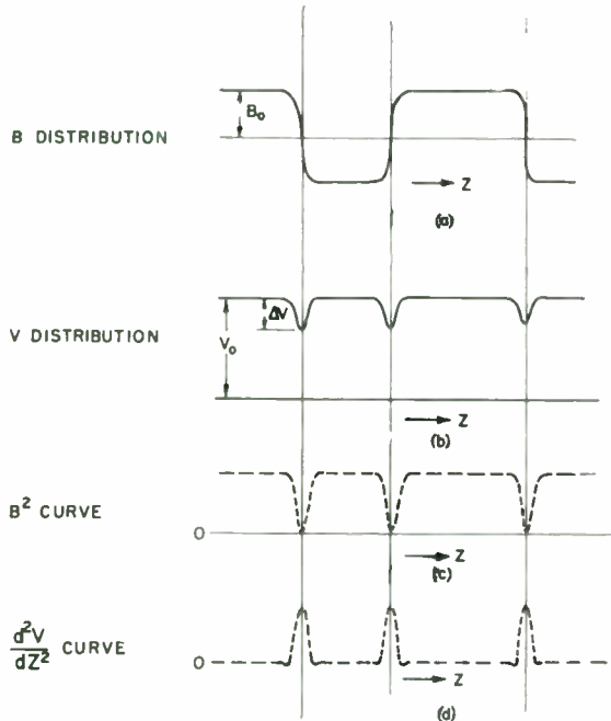
Fig. 2—Complementary diagram of focusing action in complementary fields.
