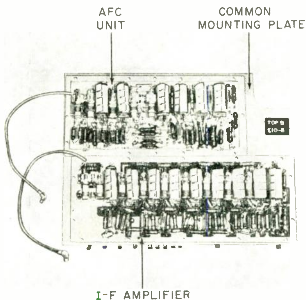
Fig. 6.—Intermediate frequency amplifier and automatic frequency control unit assembly with covers removed.
