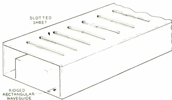
Fig. 1—General form of new space-harmonic circuit structure.
