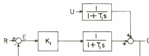
Fig. 1—Block diagram of velocity regulating system.
