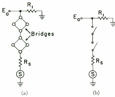
Fig. 13—A series combination of gates.
