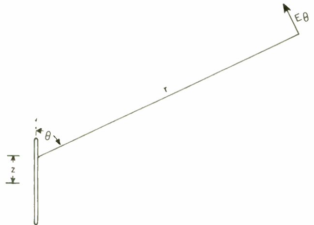
Fig. 8—Scattering wire with incident wavenormal not normal to the wire.
