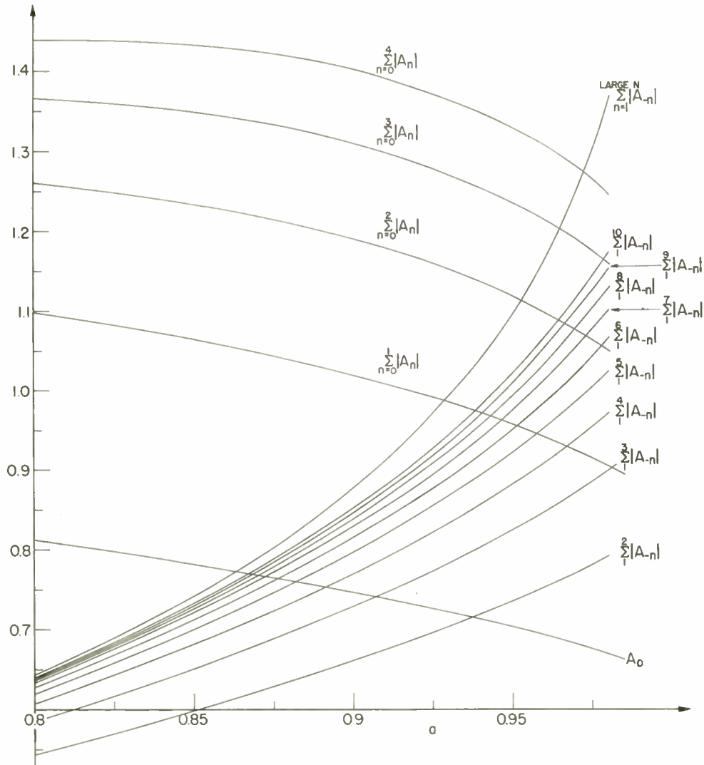
Fig. 4—Plots of the variation with a of: A_0 , the spectral component having the frequency of the stronger carrier; \sum_{n=1}^N |A_{-n}| , the sum of the magnitudes of the first N upper-sideband components (the curve for which the upper limit of the summation is marked "large N " represents essentially the sum of the magnitudes of all the upper-sideband components); \sum_{n=0}^M |A_n| , the sum of the magnitudes of A_0 and the first M lower-sideband components.
