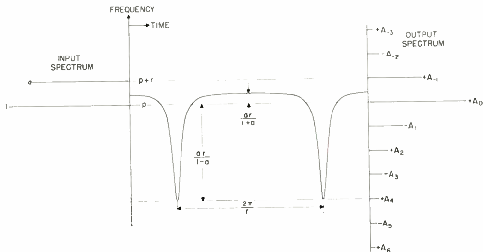
Fig. 2—The variation of the instantaneous frequency of the resultant signal with time. Input and calculated output spectra are superimposed to clarify the notations and the locations of the spectral components.
