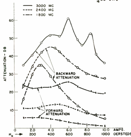
Fig. 2—Attenuation vs static magnetic field for constant frequency.
