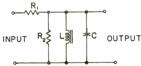
Fig. 4—Lag network.
