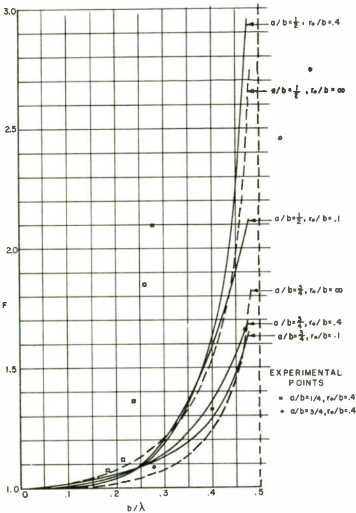
Fig. 5—Frequency factor for dimensions comparable with wavelength for Fig. 1.
