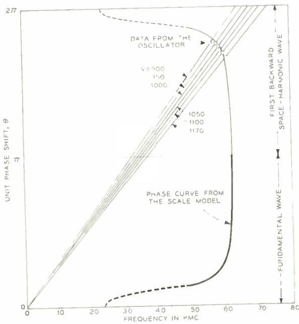
Fig. 8—Frequency vs beam voltage data of 60 mc backward-wave oscillator compared with phase characteristic of the circuit.
