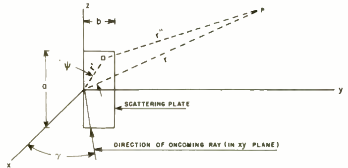
Fig. 4—Rectangular plate with electromagnetic wave incident from some direction in the XY plane.
