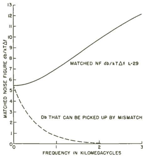
Fig. 6—Matched grounded-grid L-29 noise figure.
