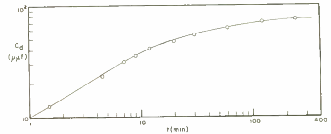
Fig. 11—Log-log plot of the time dependence of the differential capacitance of a large-area silicon p-n junction with 3 volts reverse bias applied at t=0 .
