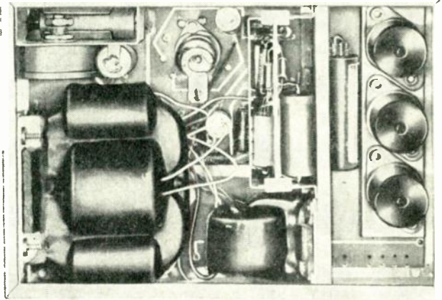
Fig. 10—Ac voltage regulator and power-switching unit assembly.
