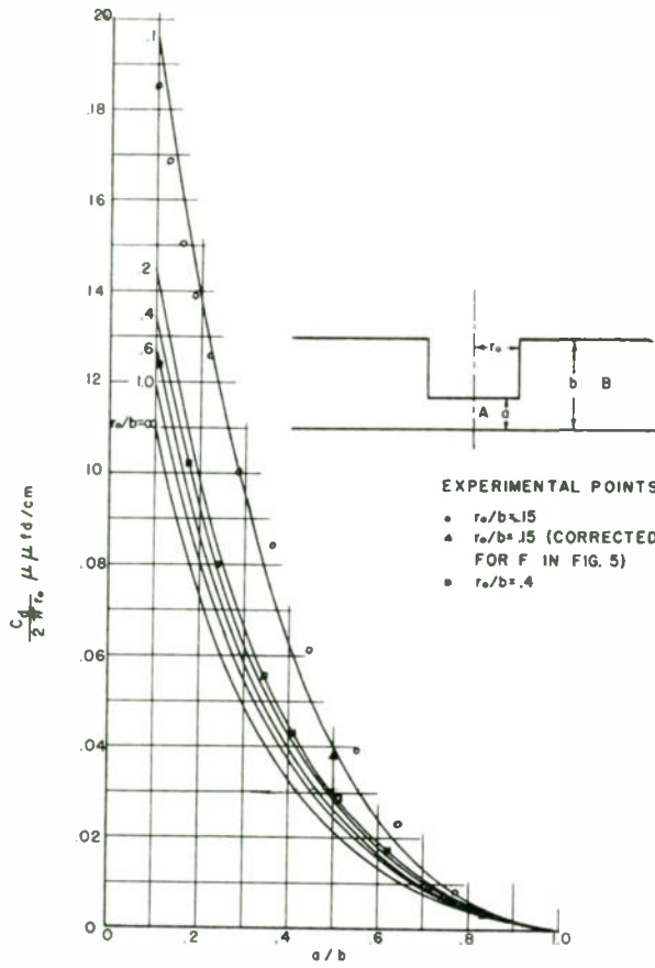
Fig. 1 (a) and (b)—Discontinuity capacitance for step in radial line, wider spacing outside.
