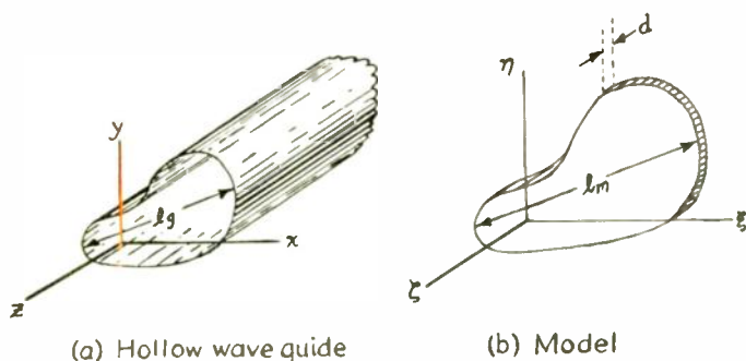
Fig. 1—Two-dimensional transmission line used as a model of a uniform metal-walled guide.
