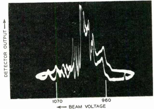
Fig. 9—Band of backward-wave oscillation centered at 3.6 mm wavelength. Oscillogram taken at Holmdel, N. J., on April 28, 1953.
