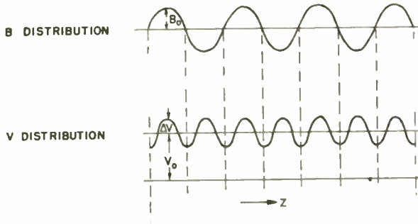
Fig. 3—Distribution of the flux density and the potential along the axis for a sinusoidal complementary field.
