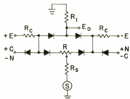
Fig. 10—Six-diode-bridge gate.
