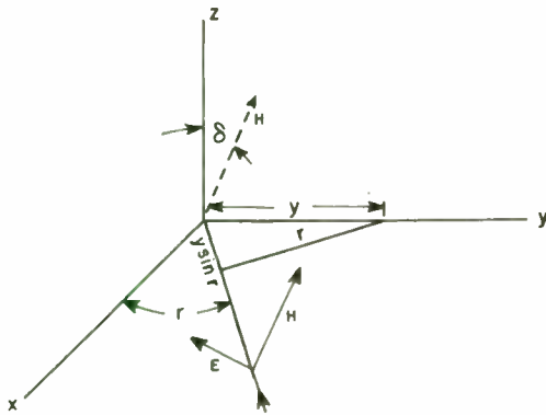
Fig. 5—Angles employed for the scattering calculation.
