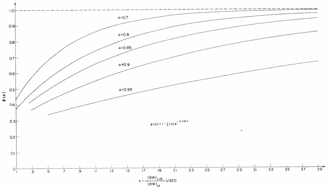
Fig. 12—Normalized plots of the "envelopes" of the broken curves of Fig. 10. \psi(a) equals the normalized minimum required discriminator bandwidths at the odd integral values of x .
