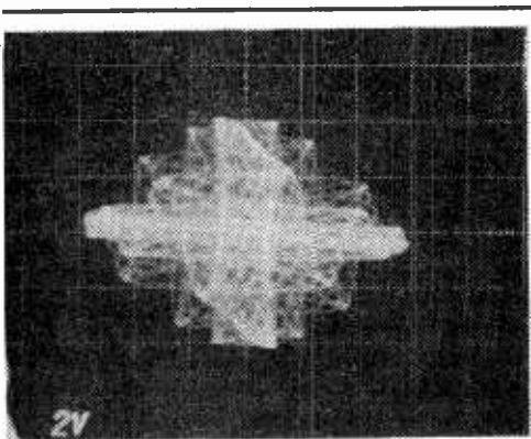
Fig. 3: An oscilloscope photo of the M7000 copying RTTY at 75 baud and 170 Hz shift.
