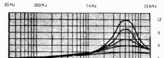
5000 Hz high-frequency equalization
