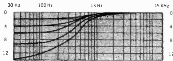
100 Hz low-frequency attenuation
