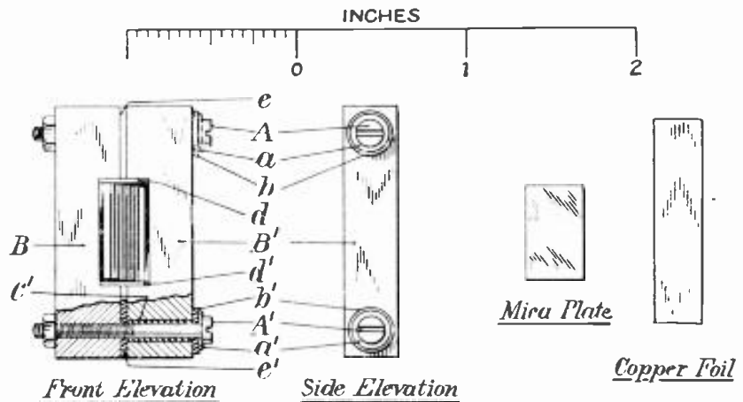
Fig. 1. Working Drawings
