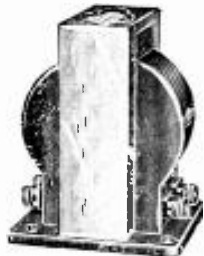
L.F. Transformer, Type "G." Gives the most even amplification of all frequencies under working conditions. A massive instrument in which neither materials nor workmanship has been stinted. Two ratios—3.0:1, for 20,000-30,000 ohm valves, and 7.2:1, for 10,000 ohm valves. Price 30/-.
