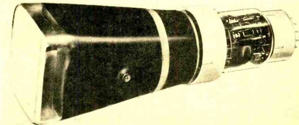
Fig. 6. This industrial multi-gun cathode-ray tube has five electron gun and deflection assemblies.
