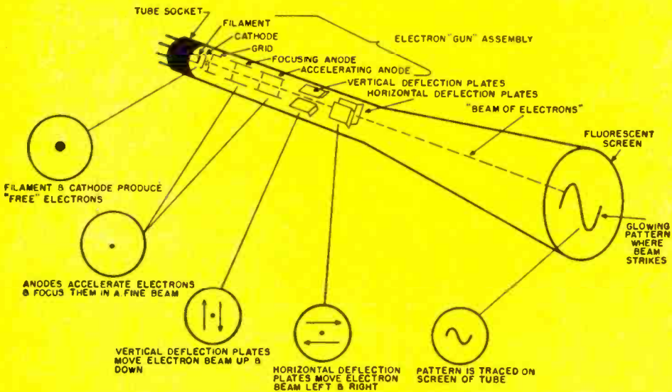
Fig. 2. Construction details of an electrostatic type cathode-ray tube.
