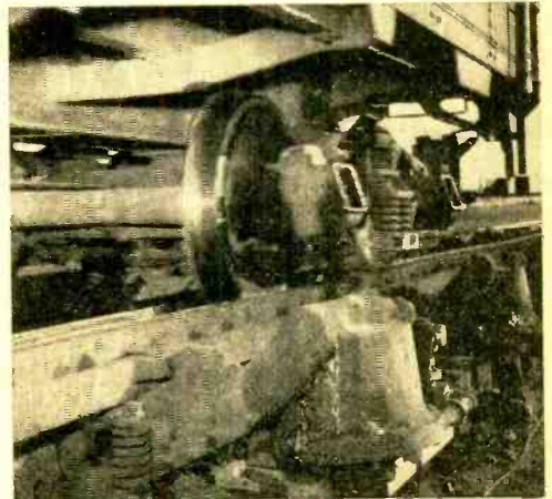
Air-operated pistons apply pressure to steel bars that grip the car's wheels. This slows the car to required speed.
