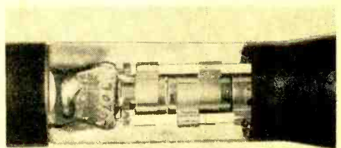
Fig. 3. Photographic illustration of the electron gun assembly of cathode-ray tube.
