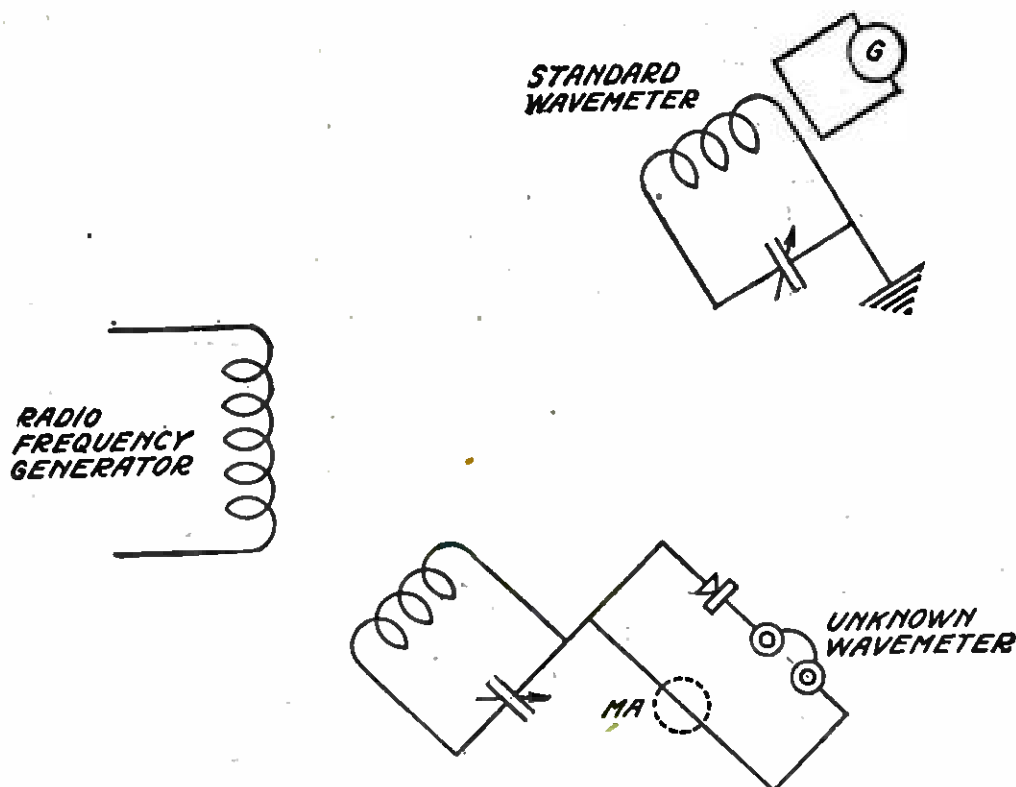
FIGURE 3: To calibrate an unknown wavemeter employing a uni-lateral connection either a crystal detector may be used or else a milliammeter, as indicated by the dotted circle.
