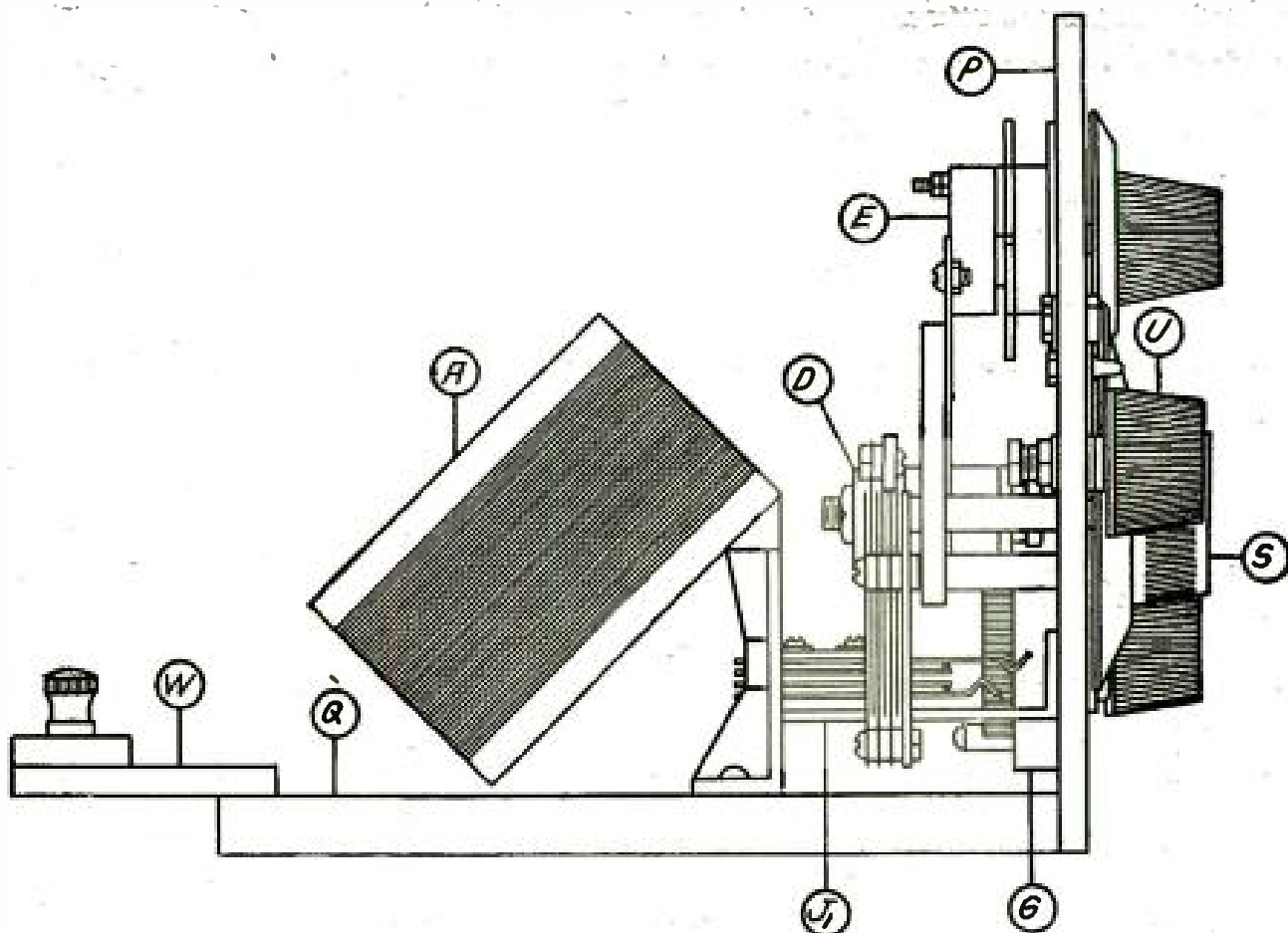
VIEW OF THE SET FROM THE LEFT
