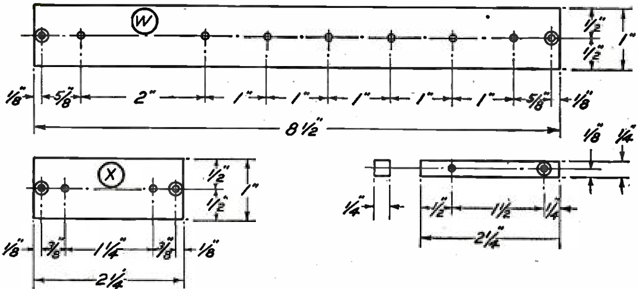
FIGURE 8: The sizes for the connecting blocks W and X and the brass supporting pieces. Two of the 2\frac{1}{4} inch brass pieces are used for mounting each block.
