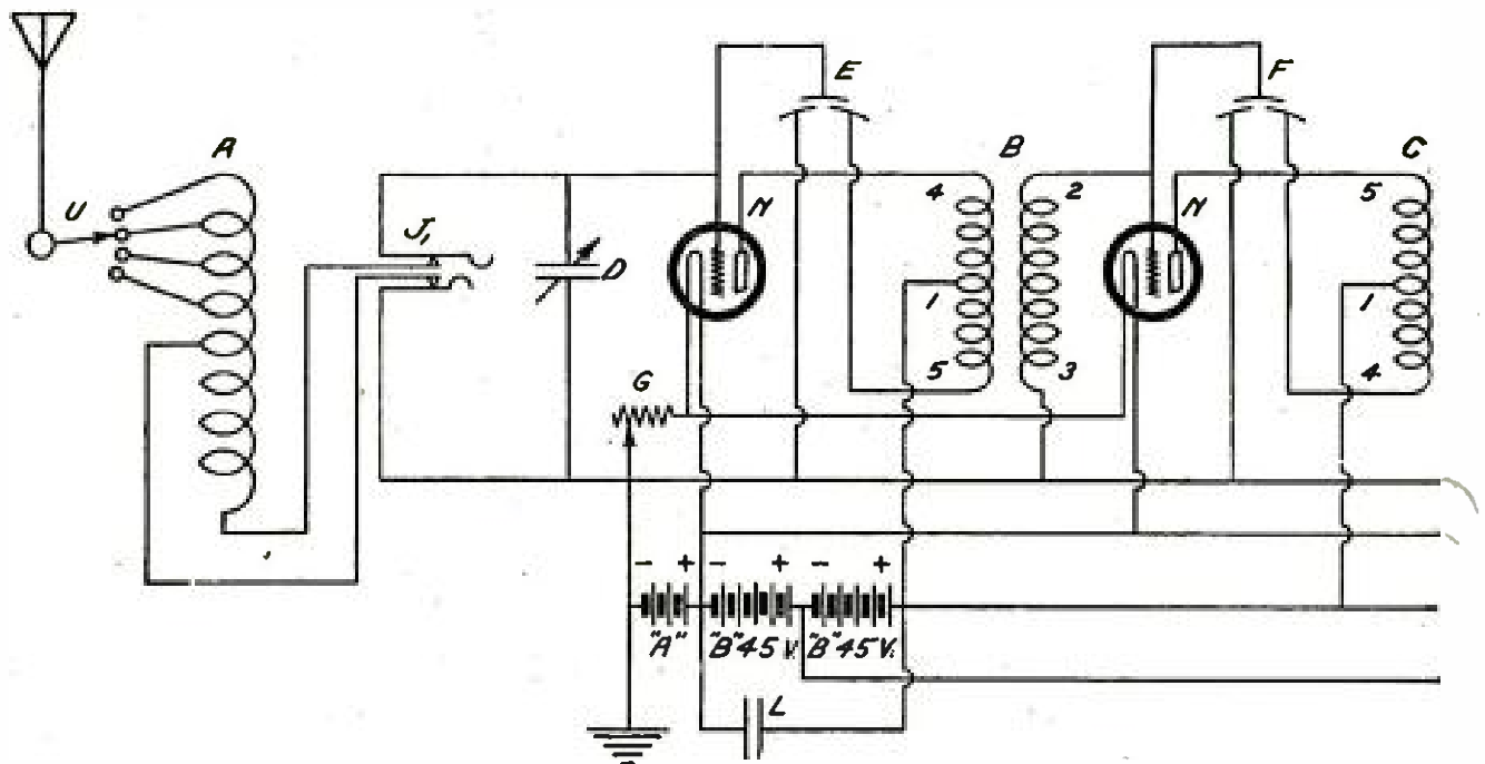
CIRCUIT DIAGRAM OF THE NEW 5-TUBE RECEIVER
