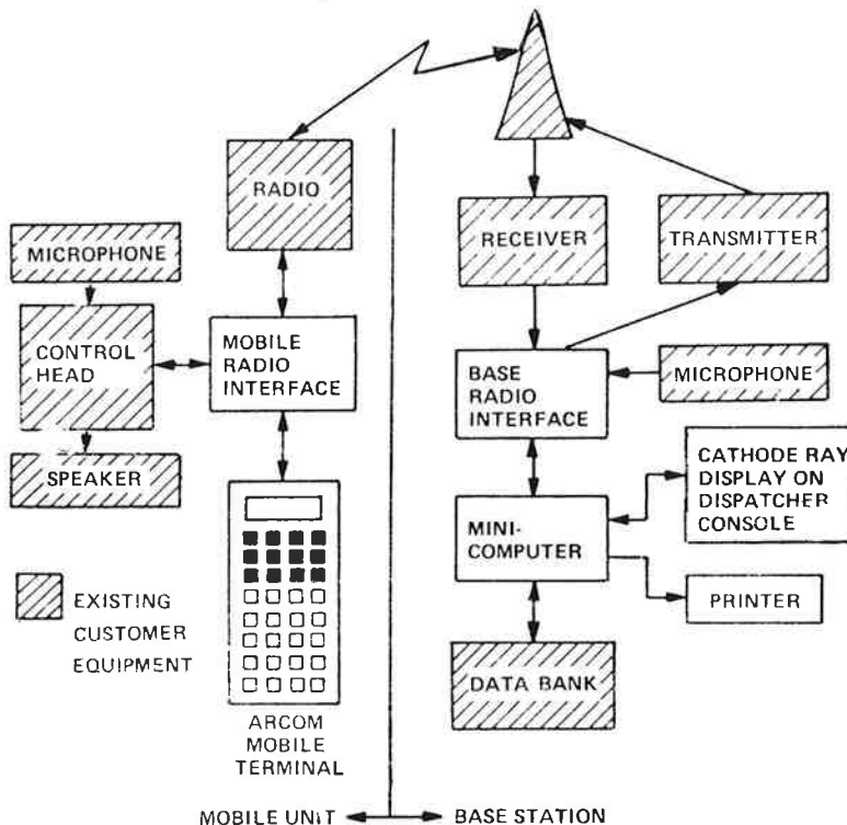
Fig. 2. Block diagram distinguishes new and existing equipment.
