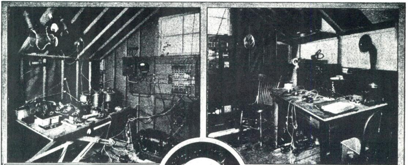
Above is the Transmitter at IBCG. It consists of Four 250-Watt Tubes Hooked up as Shown by the Diagram on This Page. The Radiation in the Aerials Was About Six Amperes.
