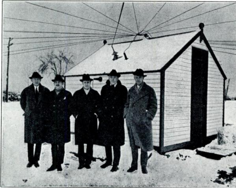
The station building at 1BCG and five of its owners. Left to right, Messrs. Amy, Grinan, Burghard, Armstrong, Cronkhite. Mr. Isman is missing in this photo. Note the counterpoise radiating from the top of the station, and the lead-in from it and the antenna.
