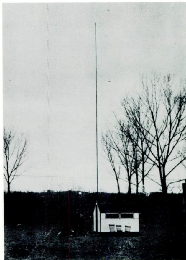
Overall view of station looking west. Counterpoise pole and wire in foreground, 108 foot mast in background.
