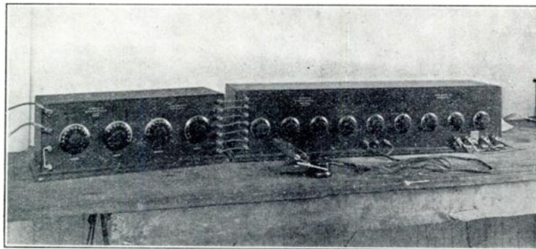
The tuner and amplifier which made up the Super-Heterodyne used at Ardara. As connected for use with Beverage antenna, the special regenerator shown on page 25 was inserted between this tuner and the antenna.
