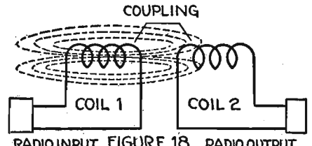
FIGURE 18 RADIO INPUT RADIO OUTPUT
