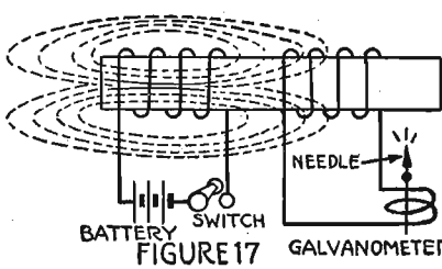
FIGURE 17 BATTERY SWITCH GALVANOMETER
