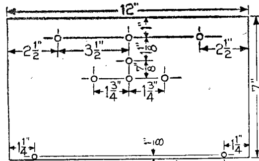
Figure 3. Panel drilling layout.
