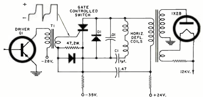
Fig. 3. Horizontal-output stage uses a gate-controlled switch.
