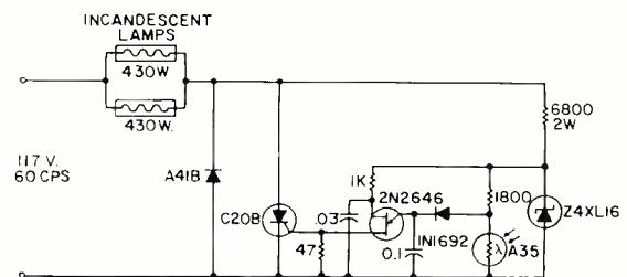
Fig. 4. High-gain limited-range light control circuit with unijunction transistor. For applications in which control of the load below the half-power point is not required, a rectifier can supply a half cycle uncontrolled, and an SCR can provide regulation by phase control during the other half cycle.
