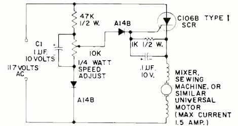
Fig. 3. A popular variable speed control circuit using SCR.
