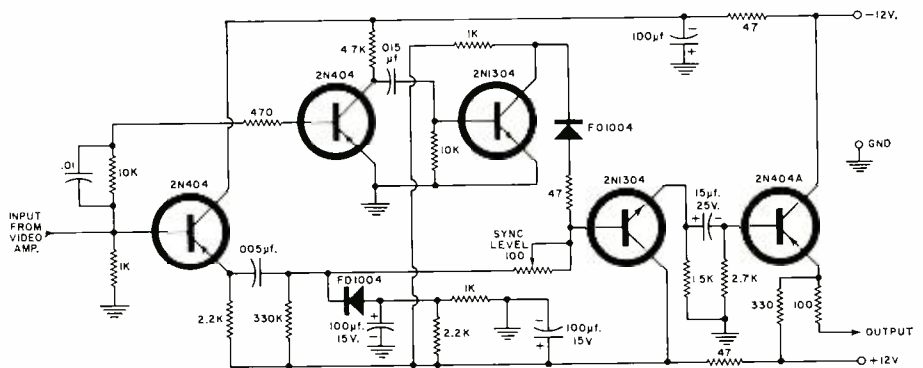
Fig. 4. (Below) Circuit employed for video clamping and for sync restoration.
