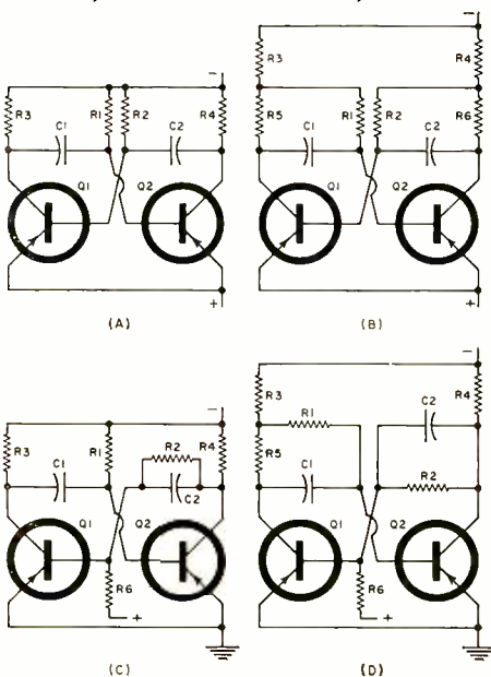
(A) Simple multivibrator circuit. (B) Improved circuit of simple multivibrator permits small-sized coupling capacitors. (C) Conventional monostable multivibrator. (D) The similar improvement also permits use of smaller capacitors.
