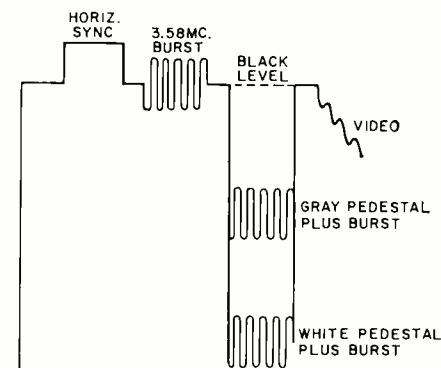
Fig. 1. Suggested locations for added bursts at gray and white video levels.
