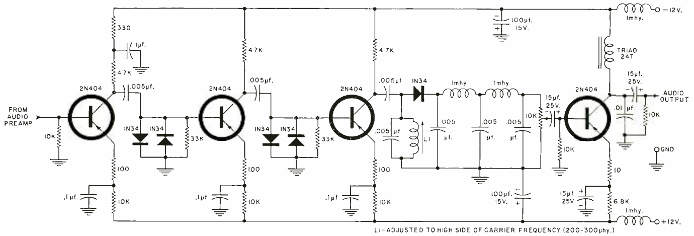
Fig. 6. A two-stage audio limiter is followed by a slope detector, low-pass filter, and audio output amplifier.
