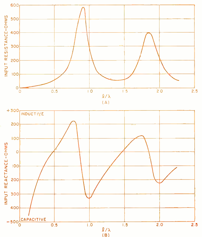
Fig. 1. (A) Resistive and (B) reactive components of the input impedance of a center-fed linear dipole antenna element.
