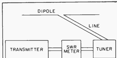
Figure 6—The antenna tuner allows the transmitter to work into an optimum load even if the dipole itself is not cut for the correct frequency. A tuner won't correct an inefficient antenna installation.
