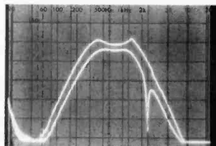
Fig. 2, Inner trace shows proper adjustment of PRIMARY and AUXILIARY controls. Outer trace shows breakup from misadjustments.
